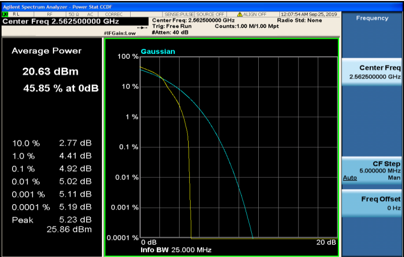
Band7-15MHz-16QAM-21375-75RB#0
