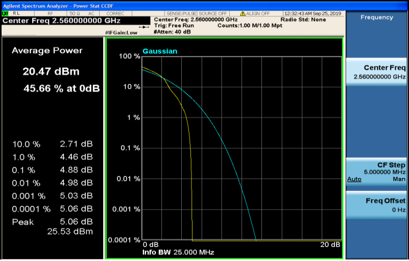
Band7-20MHz-16QAM-21350-100RB#0
