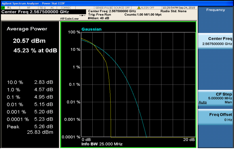
Band7-5MHz-16QAM-21425-25RB#0
