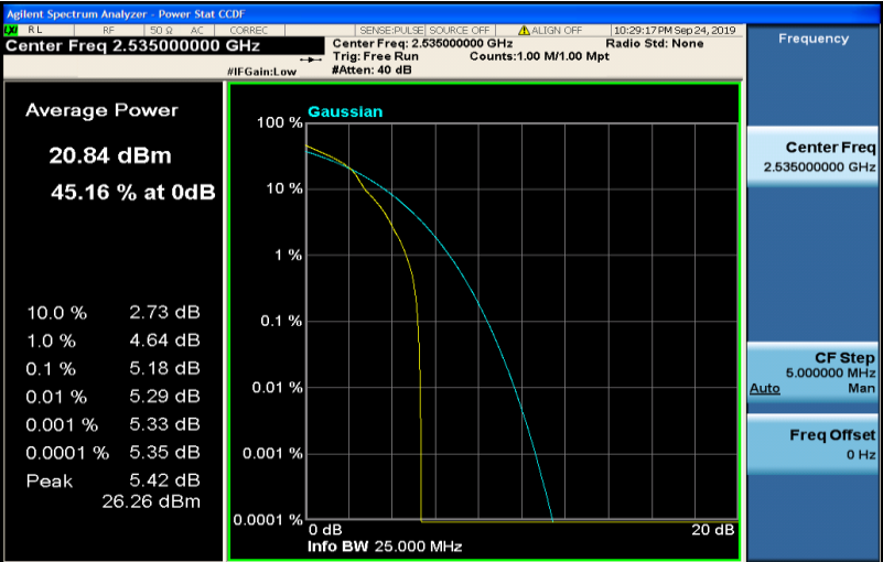
Band7-5MHz-16QAM-21100-25RB#0
