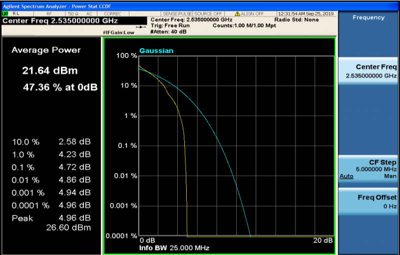
Band7-20MHz-QPSK-21100-100RB#0
