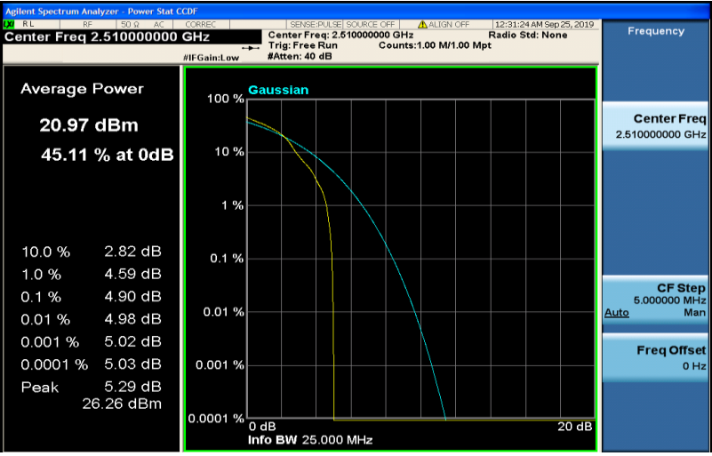
Band7-20MHz-16QAM-20850-100RB#0
