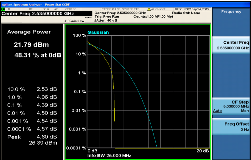
Band7-10MHz-QPSK-21100-50RB#0
