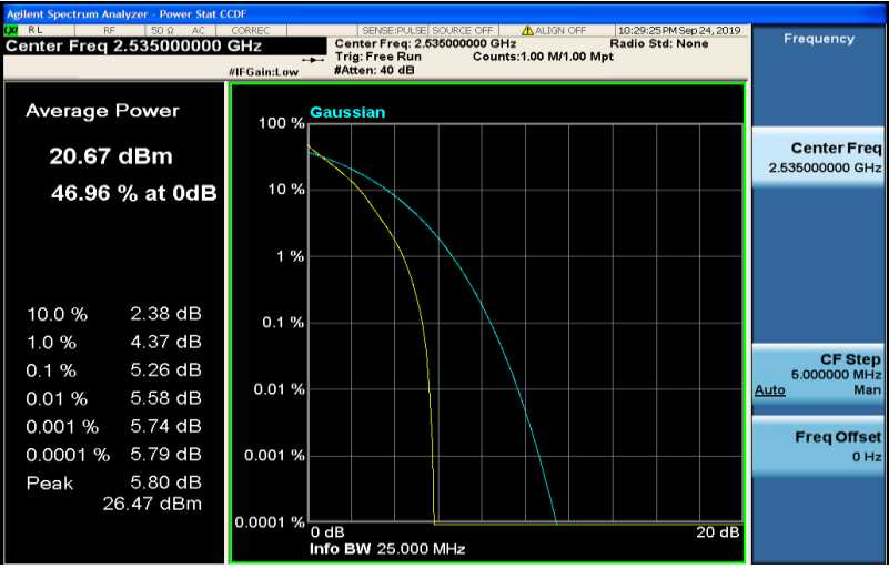
Band7-5MHz-QPSK-21425-1RB#0
