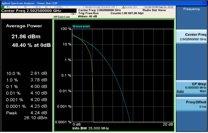
Band7-5MHz-QPSK-20775-25RB#0
