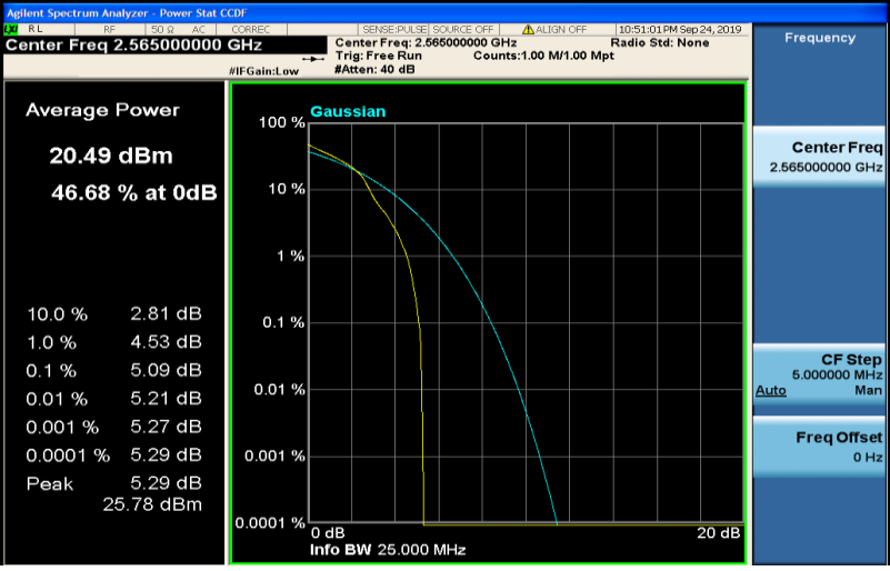
Band7-10MHz-16QAM-21400-50RB#0
