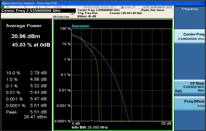
Band7-15MHz-16QAM-21100-75RB#0
