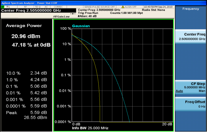
Band7-10MHz-QPSK-21100-1RB#0
