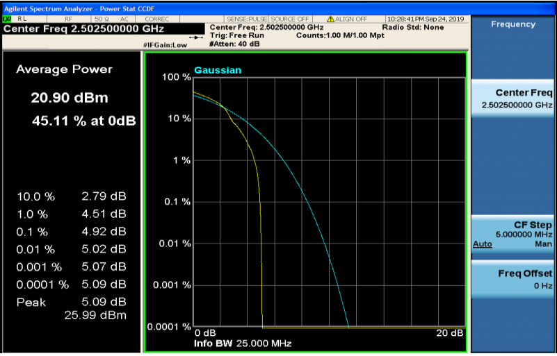
Band7-5MHz-16QAM-20775-25RB#0
