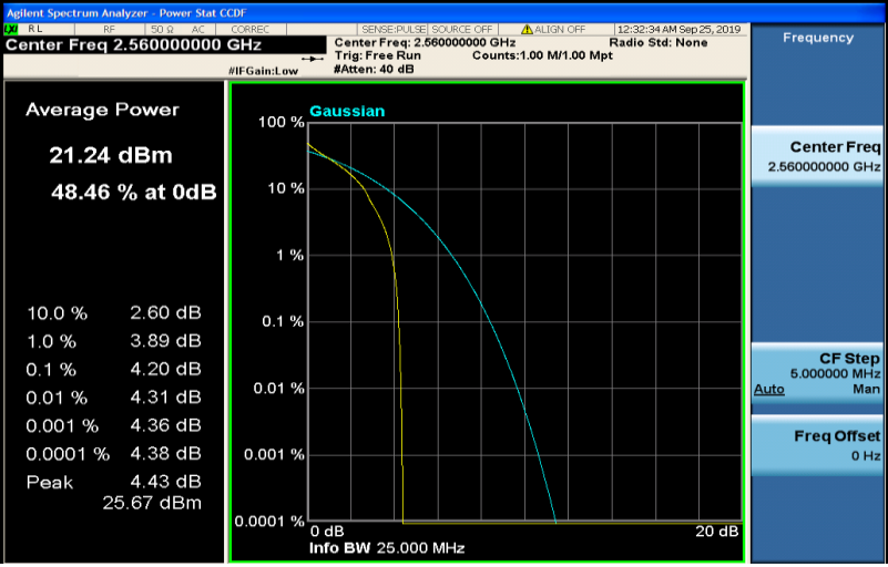
Band7-20MHz-QPSK-21350-100RB#0
