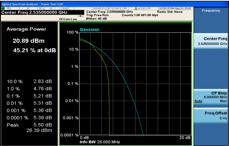
Band7-10MHz-16QAM-21100-50RB#0
