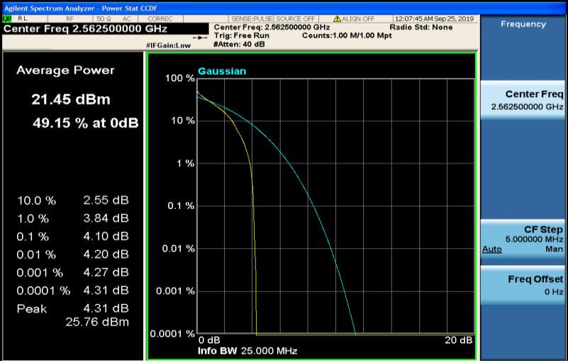
Band7-15MHz-QPSK-21375-75RB#0
