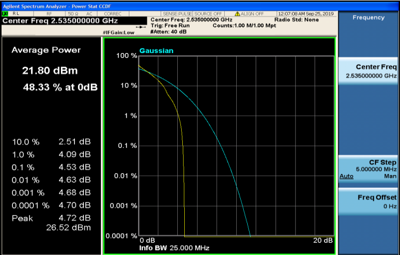
Band7-15MHz-QPSK-21100-75RB#0
