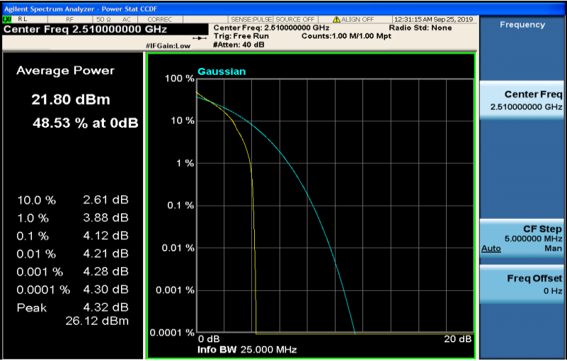
Band7-20MHz-QPSK-20850-100RB#0
