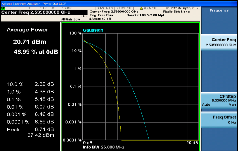
Band7-20MHz-QPSK-21350-1RB#0
