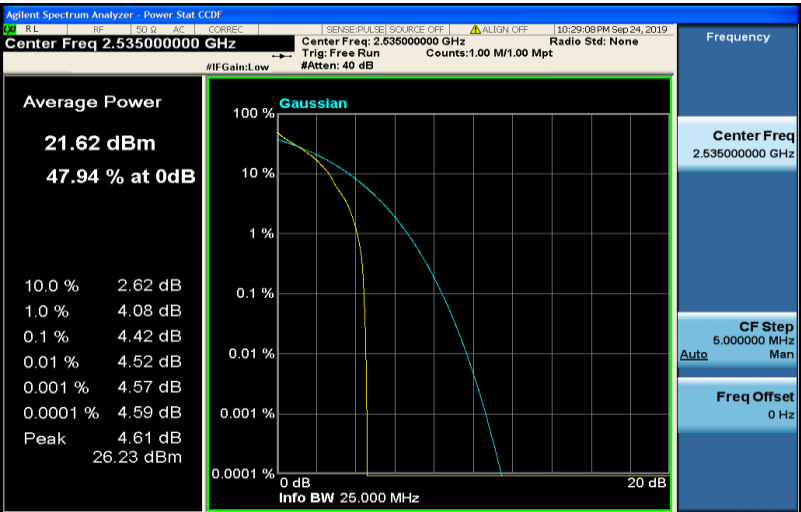
Band7-5MHz-QPSK-21100-25RB#0
