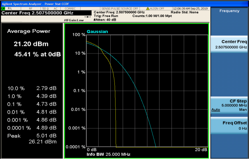
Band7-15MHz-16QAM-20825-75RB#0
