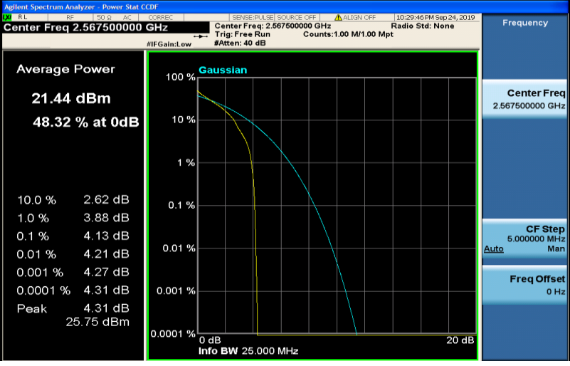
Band7-5MHz-QPSK-21425-25RB#0
