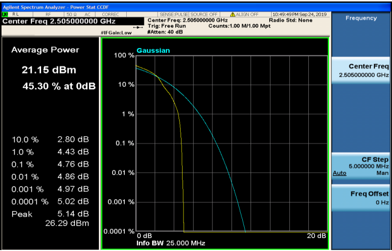
Band7-10MHz-16QAM-20800-50RB#0
