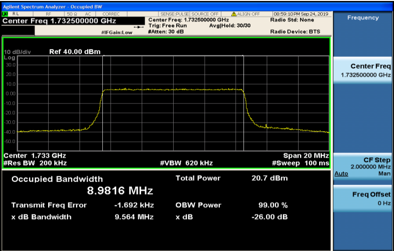
Band4-10MHz-16QAM-20350-50RB#0-8.9817
