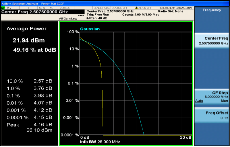
Band7-15MHz-QPSK-20825-75RB#0
