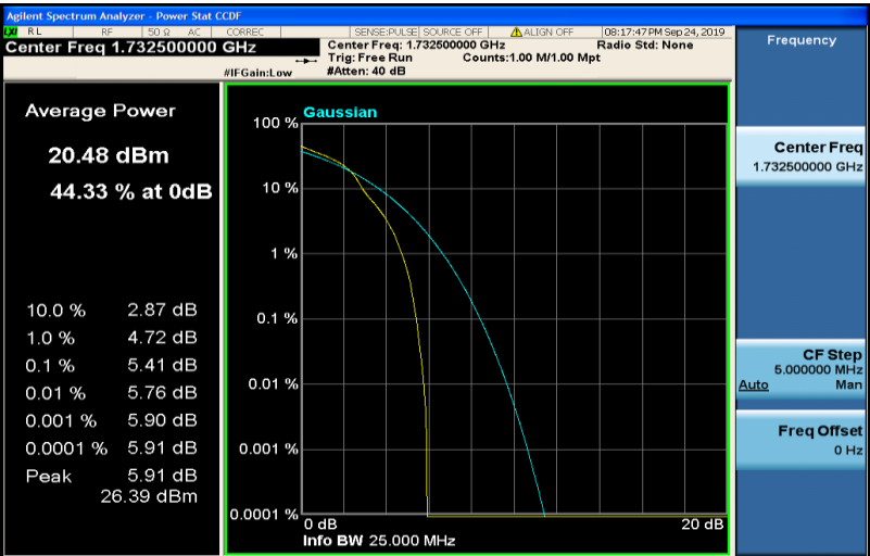
Band4-1.4MHz-16QAM-20175-6RB#0
