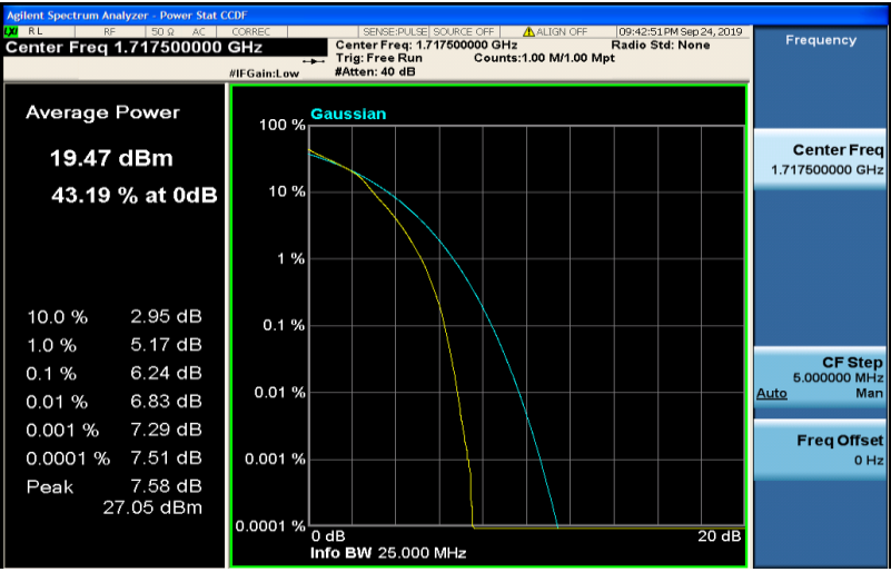
Band4-15MHz-16QAM-20175-1RB#0
