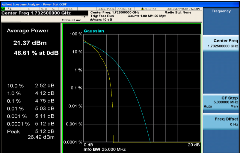
Band4-1.4MHz-QPSK-20175-6RB#0
