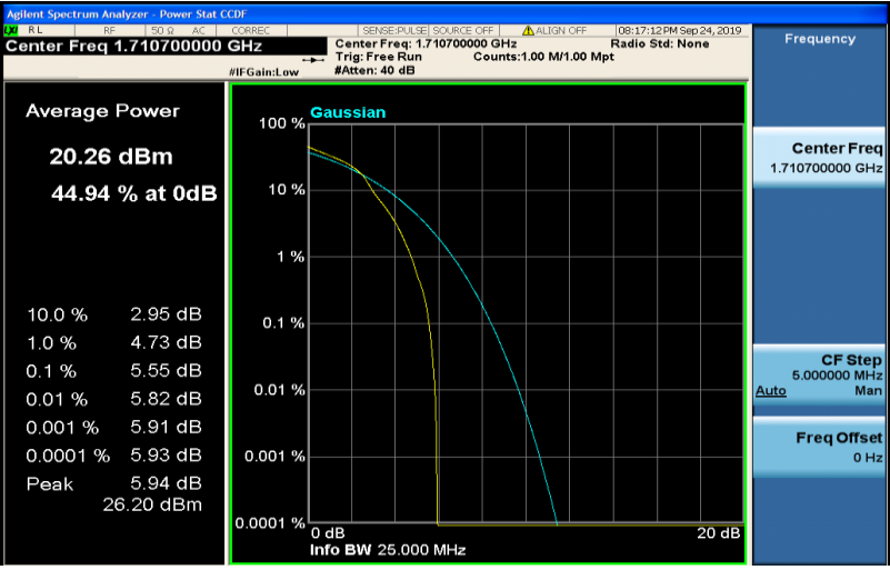
Band4-1.4MHz-16QAM-19957-6RB#0
