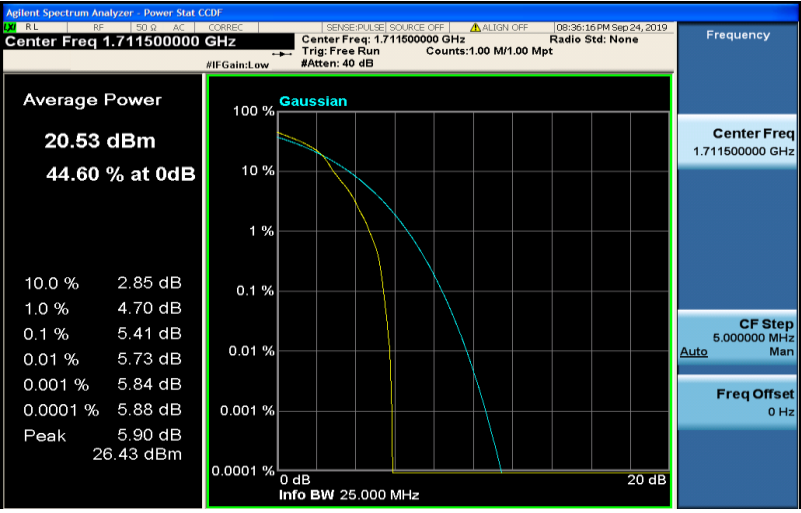
Band4-3MHz-16QAM-19965-15RB#0
