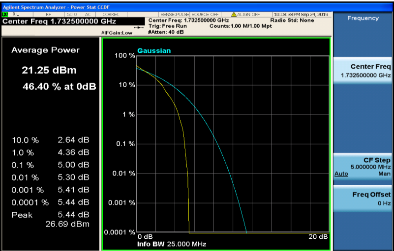
Band4-20MHz-QPSK-20175-100RB#0
