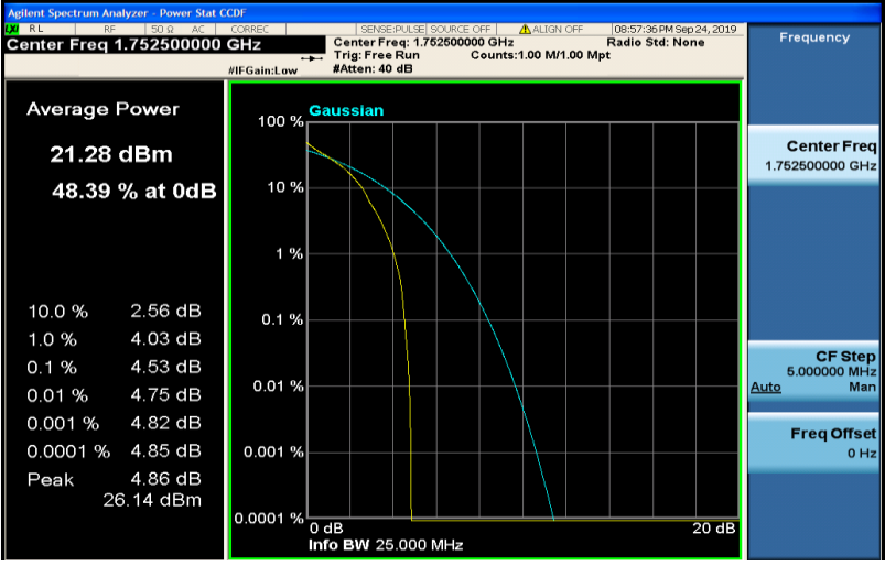
Band4-5MHz-QPSK-20375-25RB#0
