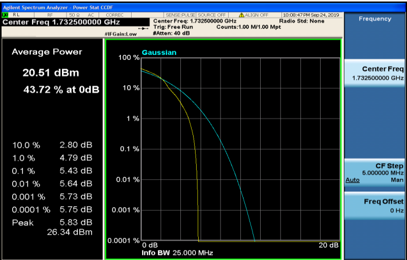
Band4-20MHz-16QAM-20175-100RB#0
