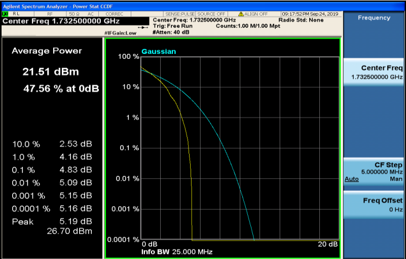
Band4-10MHz-QPSK-20175-50RB#0
