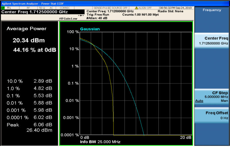
Band4-5MHz-16QAM-19975-25RB#0
