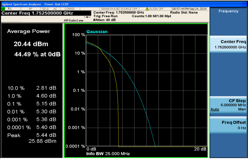
Band4-5MHz-16QAM-20375-25RB#0
