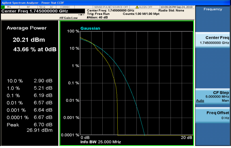
Band4-20MHz-16QAM-20300-100RB#0
