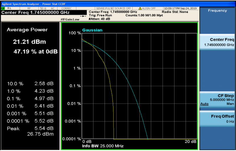
Band4-20MHz-QPSK-20300-100RB#0
