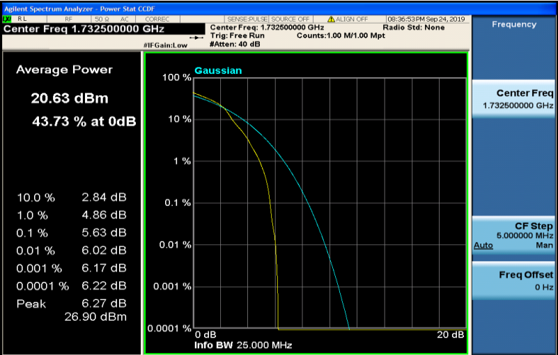
Band4-3MHz-16QAM-20175-15RB#0
