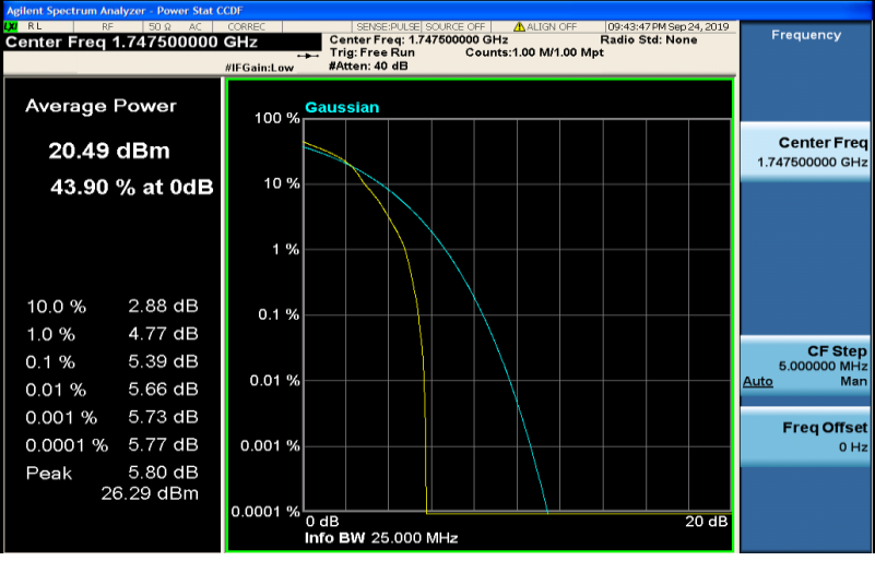
Band4-15MHz-16QAM-20325-75RB#0
