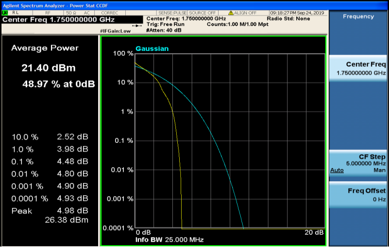
Band4-10MHz-QPSK-20350-50RB#0
