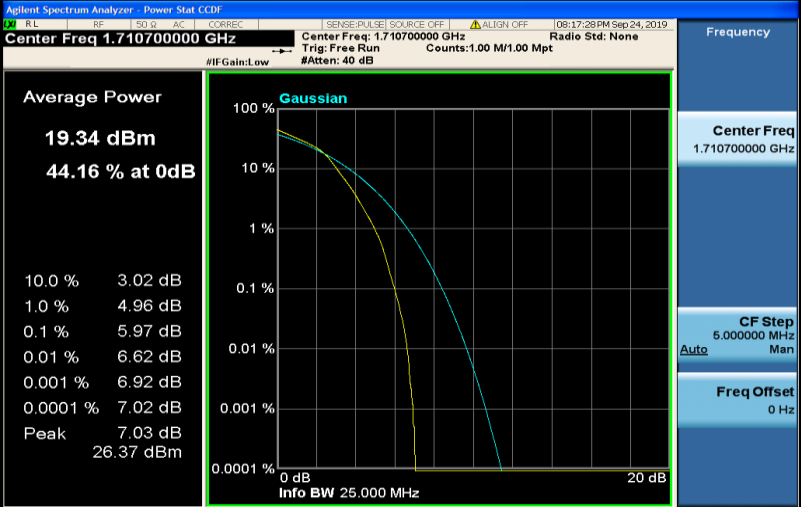
Band4-1.4MHz-16QAM-20175-1RB#0
