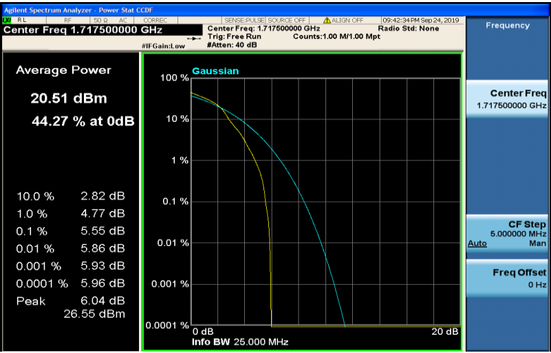
Band4-15MHz-16QAM-20025-75RB#0
