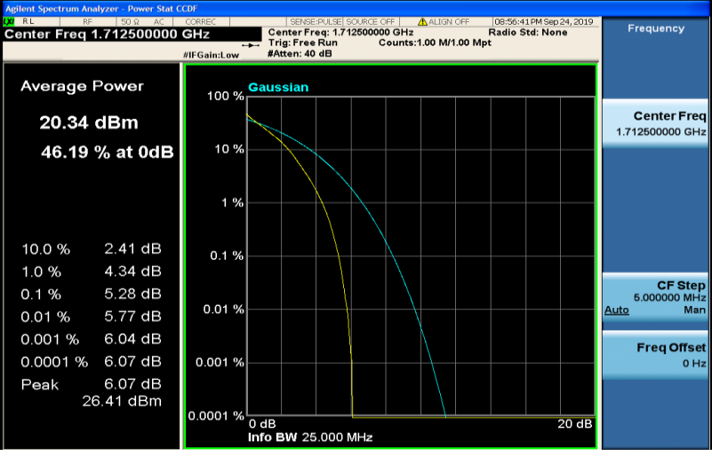
Band4-5MHz-QPSK-20175-1RB#0
