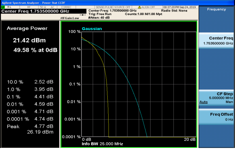
Band4-3MHz-QPSK-20385-15RB#0
