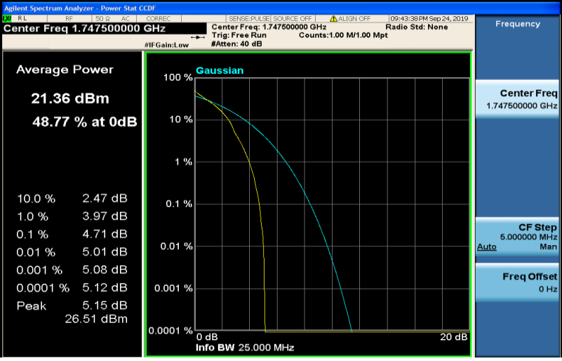
Band4-15MHz-QPSK-20325-75RB#0
