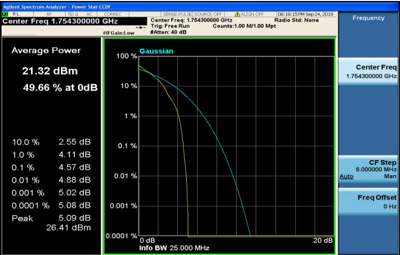
Band4-1.4MHz-QPSK-20393-6RB#0
