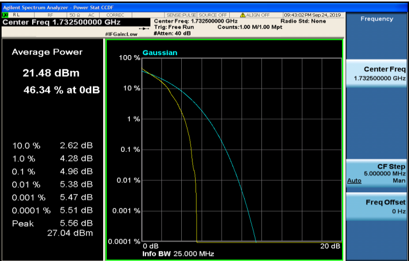
Band4-15MHz-QPSK-20175-75RB#0
