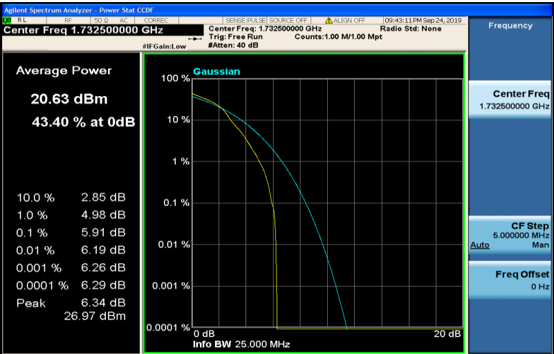
Band4-15MHz-16QAM-20175-75RB#0
