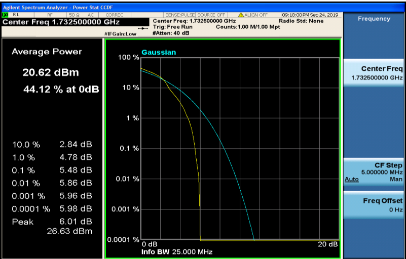
Band4-10MHz-16QAM-20175-50RB#0
