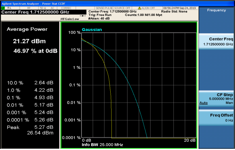
Band4-5MHz-QPSK-19975-25RB#0
