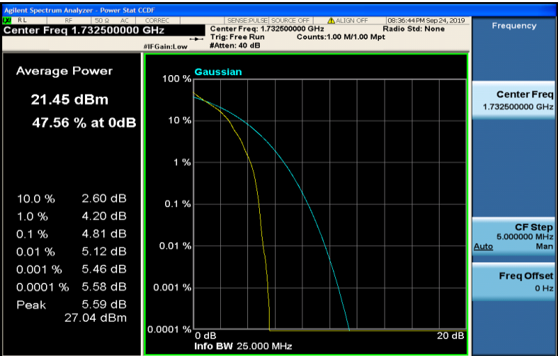
Band4-3MHz-QPSK-20175-15RB#0
