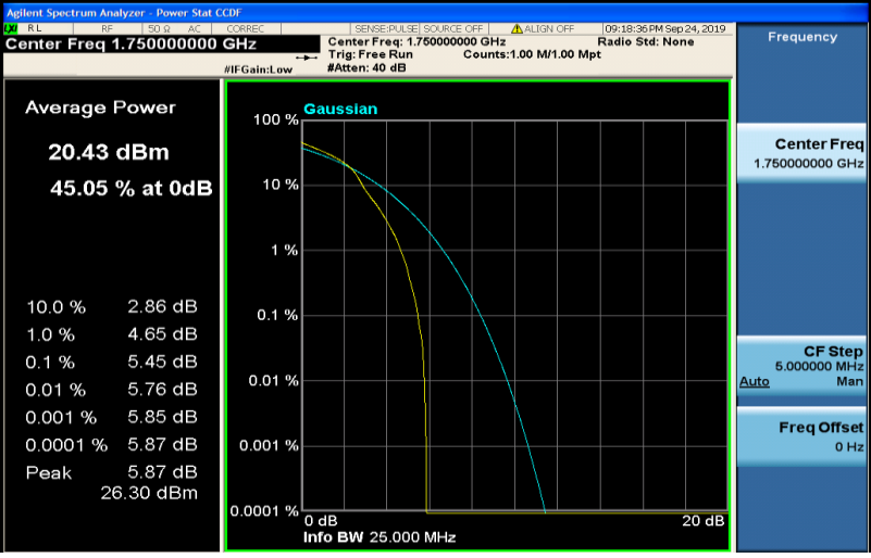
Band4-10MHz-16QAM-20350-50RB#0
