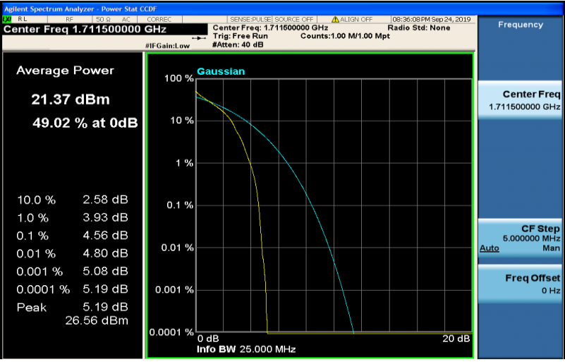
Band4-3MHz-QPSK-19965-15RB#0
