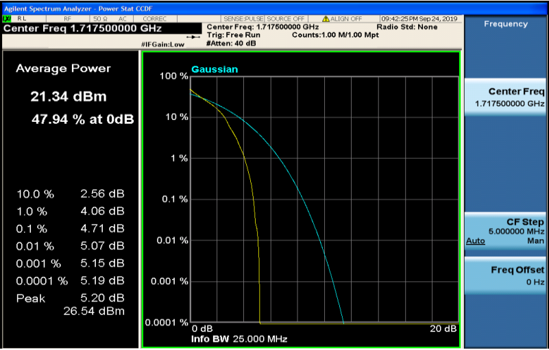
Band4-15MHz-QPSK-20025-75RB#0
