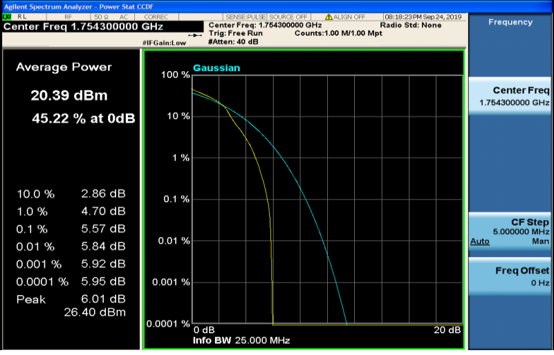
Band4-1.4MHz-16QAM-20393-6RB#0
