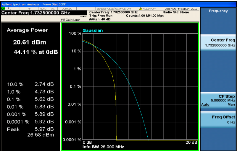
Band4-5MHz-16QAM-20175-25RB#0
