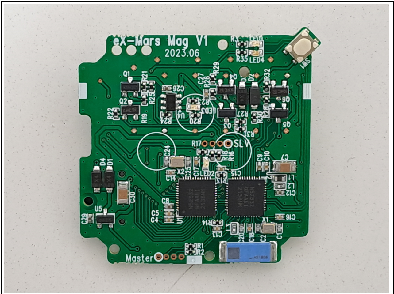
Bottom view of Main PCB
