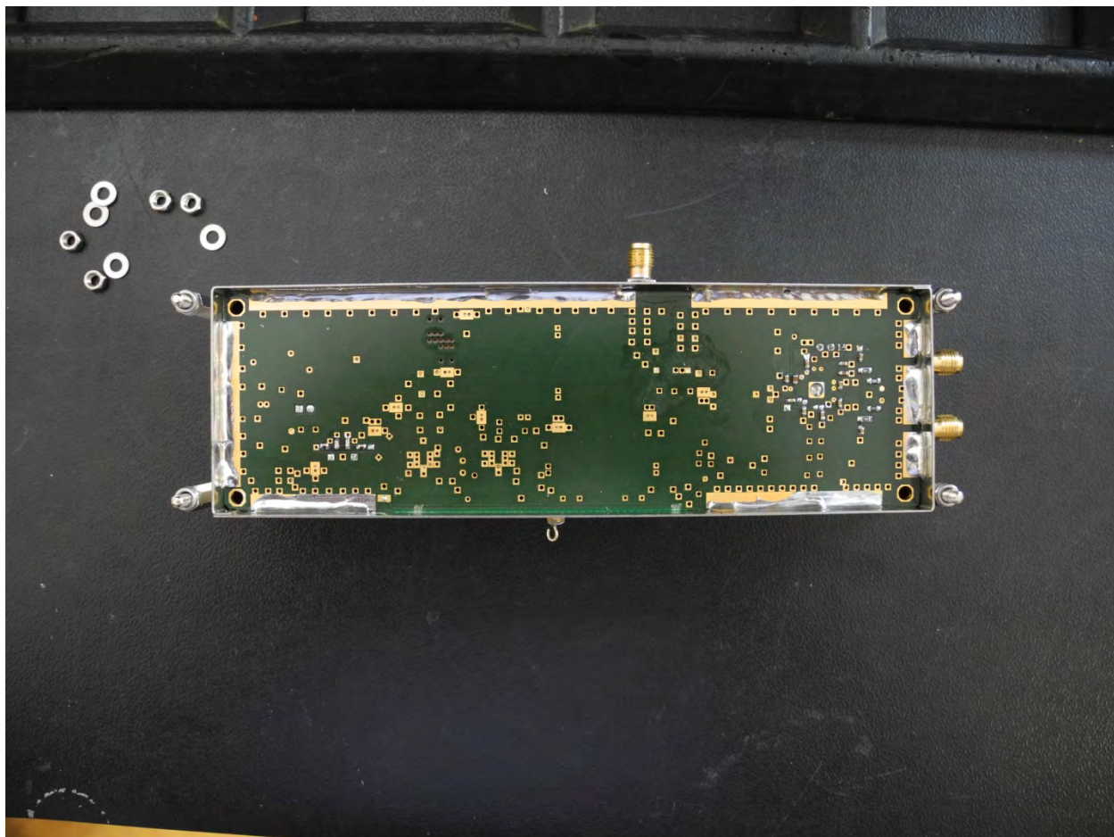
APS-500-CLK – BOTTOM VIEW
