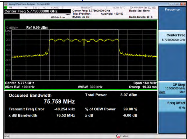
802.11AC80 plot on channel 155
