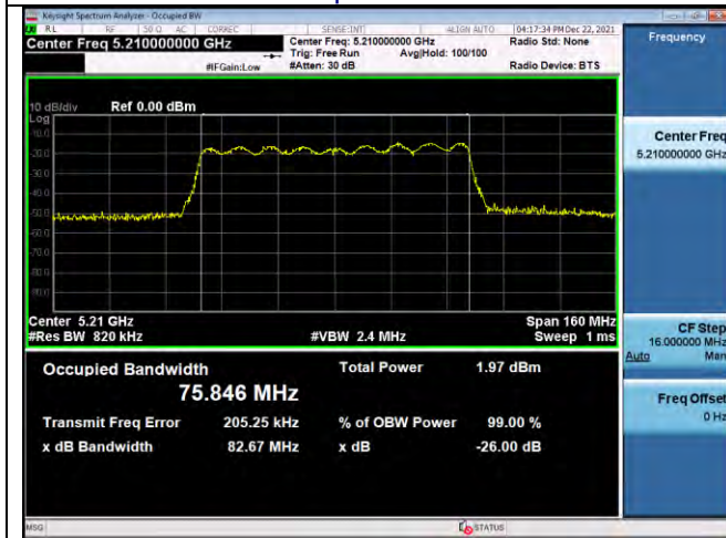
802.11AC80 plot on channel 42
