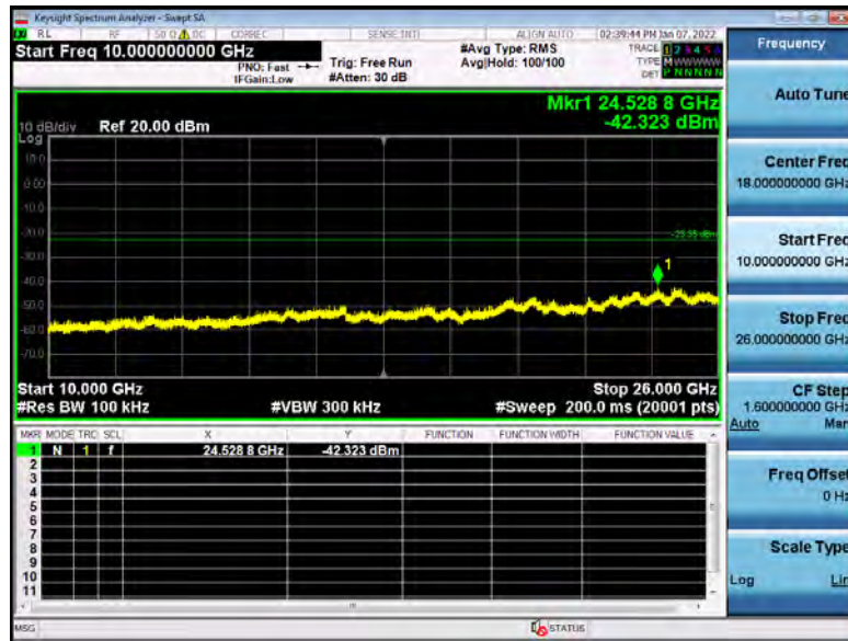
802.11n(HT40) Highest channel
