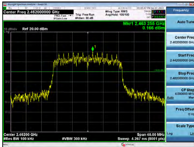
802.11n(HT20) Highest channel
