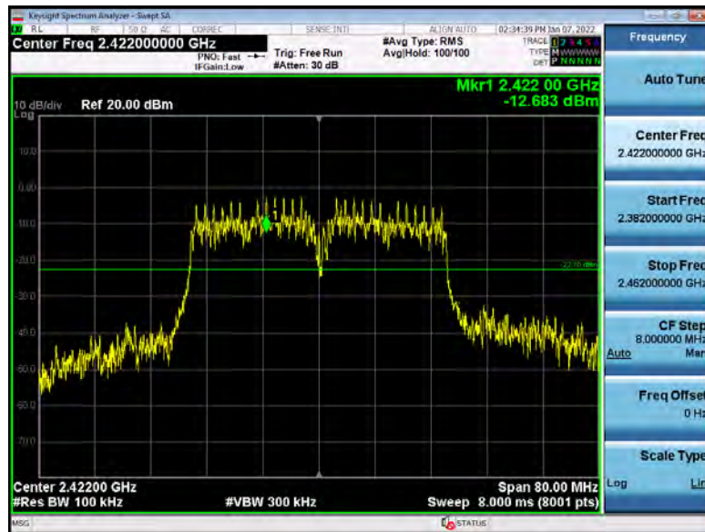
802.11n(HT40) Lowest channel
