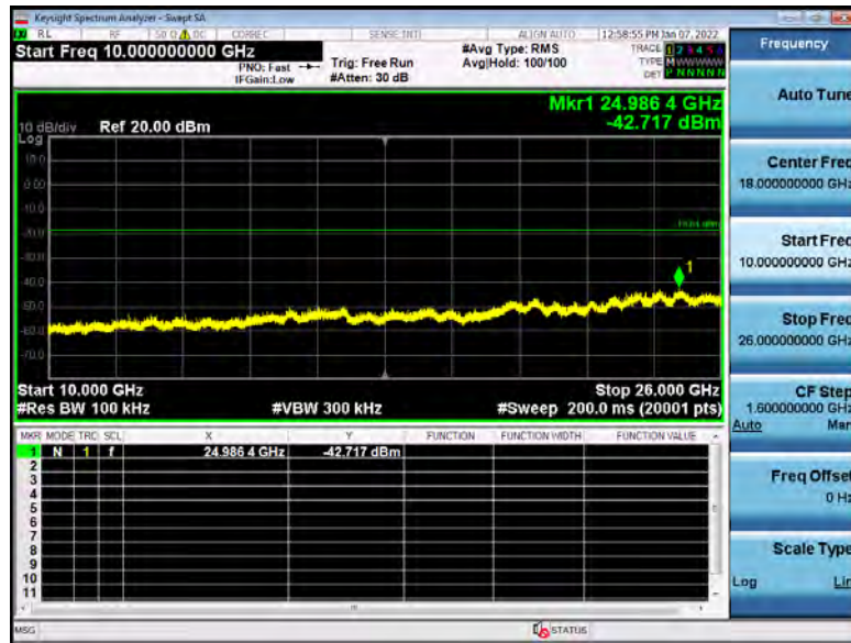
802.11n(HT20) Middle channel
