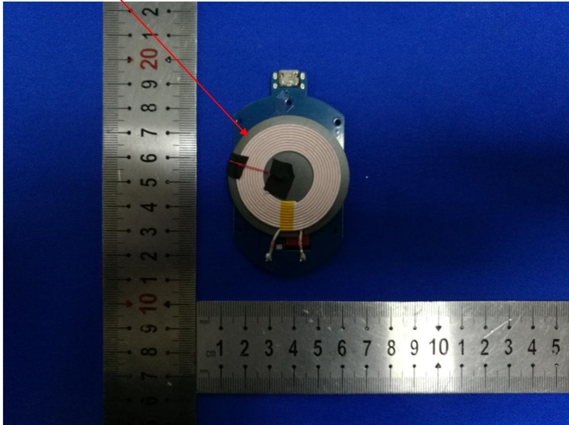
Coil Antenna:
