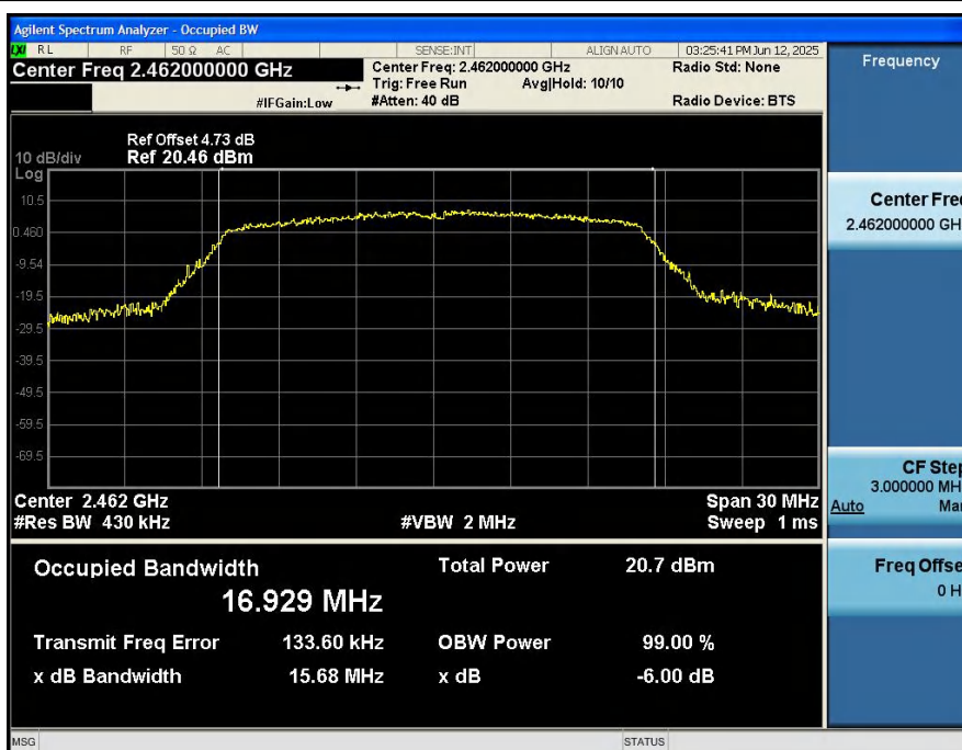
-6dB_Bandwidth_NVNT_ANT1_802_11g_2462
