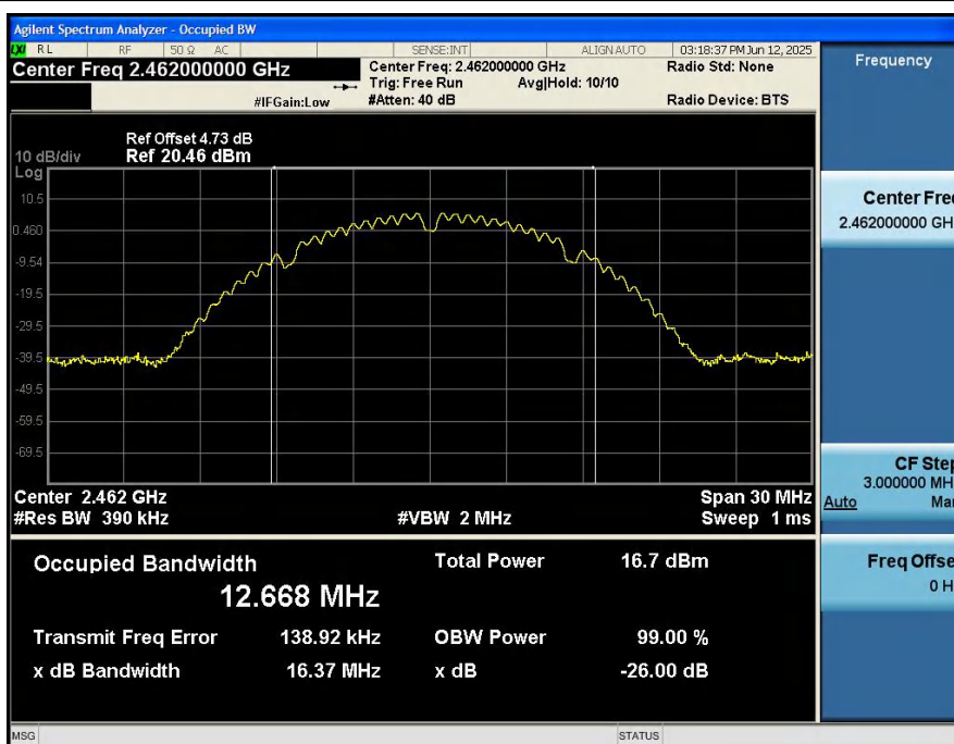
99%_Occupied_Bandwidth_NVNT_ANT1_802_11b_2462
