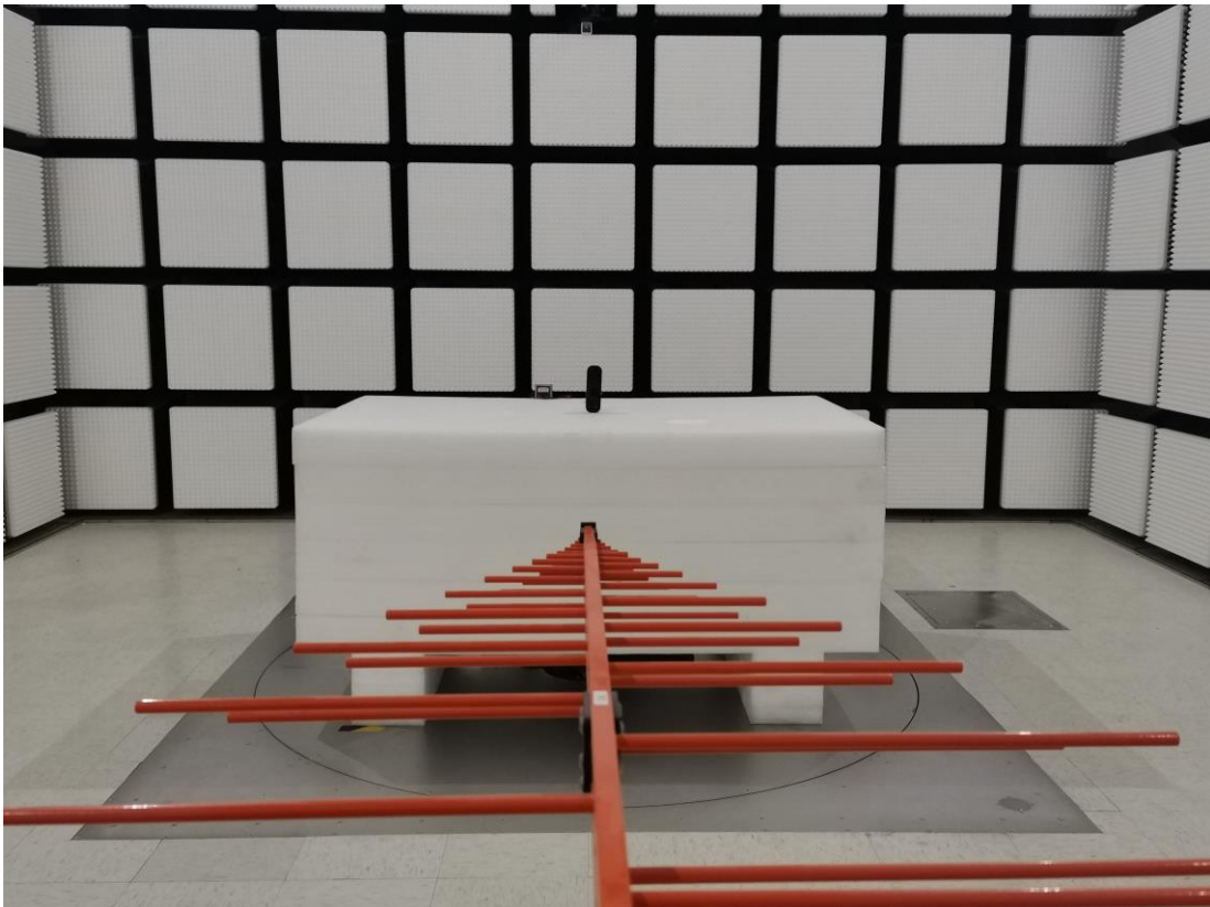
Radiated Emission Below 1GHz View- AC power
