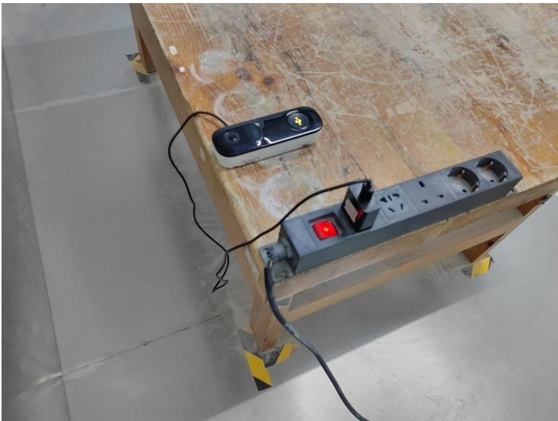
Conducted Emissions Side View- AC/DC Adapter power
