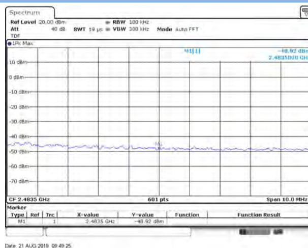
802.11n-20 MHz HIGH CHANNEL, Reference level
