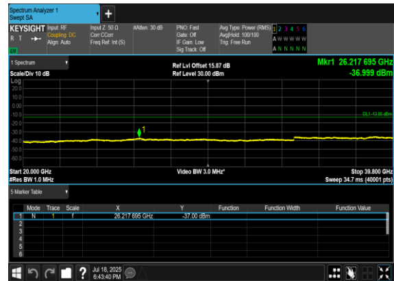
N77(50M)_DFT-s- OFDM_BPSK_Edge_1RB_Left_Low_CH
