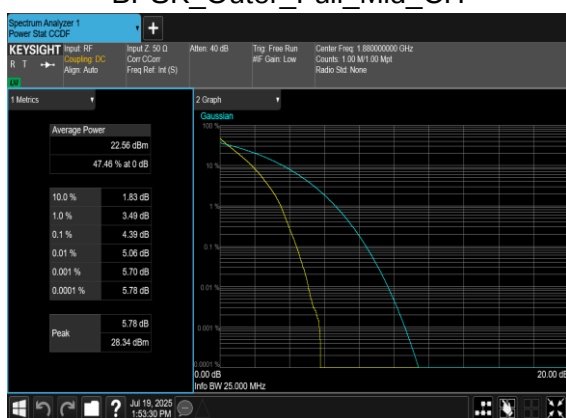
N2(20M)_DFT-s-OFDM_PI_2- BPSK_Outer_Full_Mid_CH
