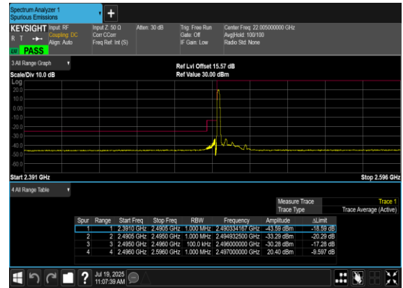
N41(10M)_DFT-s- OFDM_QPSK_Edge_1RB_Left_Low_CH
