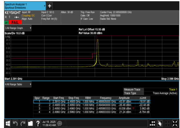
N41(100M)_DFT-s- OFDM_BPSK_Edge_1RB_Left_Low_CH
