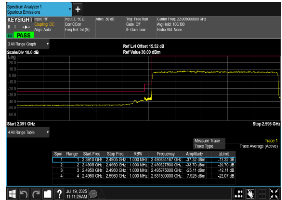
N41(100M)_DFT-s- OFDM_BPSK_Outer_Full_Low_CH
