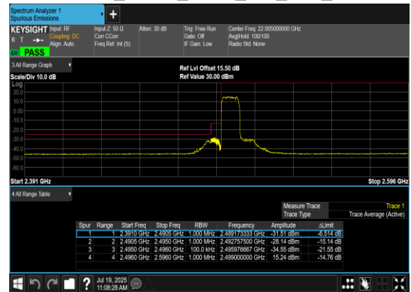
N41(10M)_DFT-s- OFDM_QPSK_Outer_Full_Low_CH
