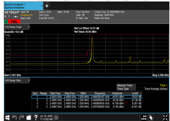
N41(100M)_DFT-s- OFDM_QPSK_Edge_1RB_Left_Low_CH
