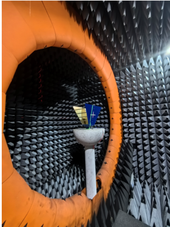
The DUT in the fully anechoic chamber
