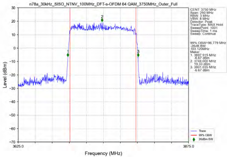
n78a_30kHz_SISO_NTNV_100MHz_DFT-s-OFDM_64_QAM_3750MHz_Outer_Full_Ant11
