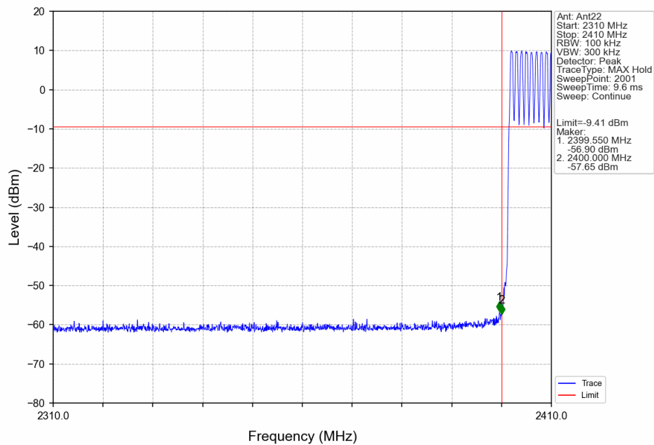
GFSK_DH5_HOPP_2410MHz_Ant22_NTNV
