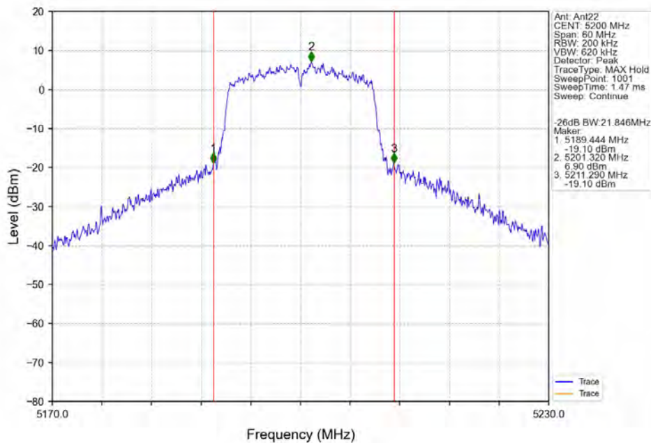
802.11ac(VHT20)_MCH_5200MHz_Ant22_NTNV
