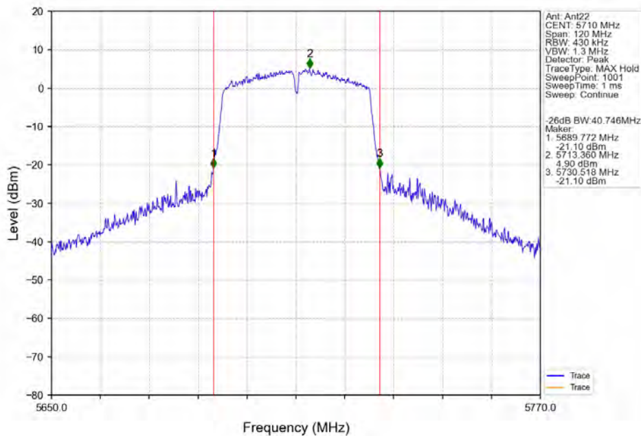
802.11ac(VHT40)_HCH_5710MHz_Ant22_NTNV
