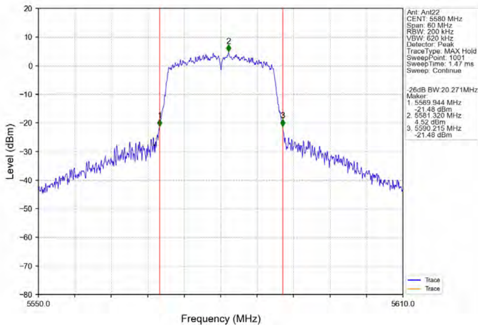
802.11ac(VHT20)_MCH_5580MHz_Ant22_NTNV
