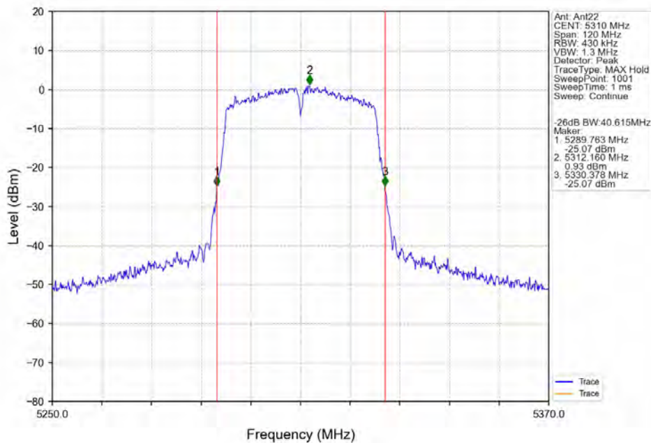
802.11ac(VHT40)_HCH_5310MHz_Ant22_NTNV
