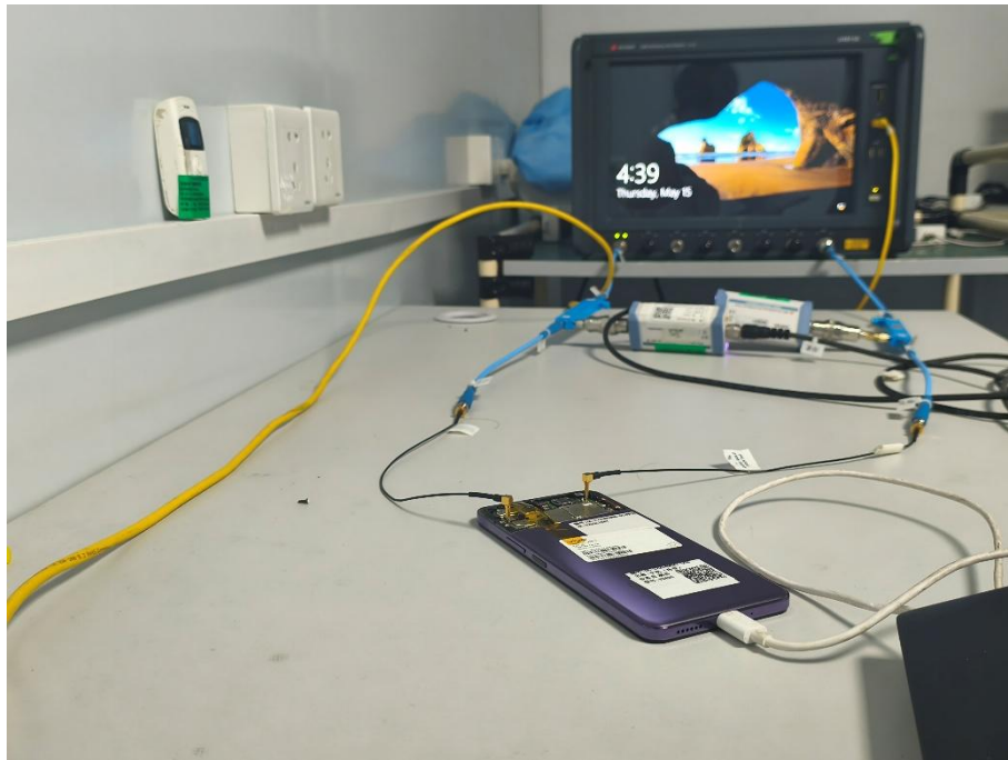
Test Setup Photo 2 on UXM E7515B
