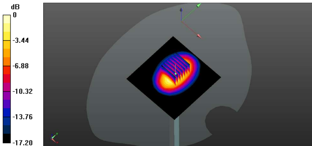
0 dB = 4.86 W/kg
