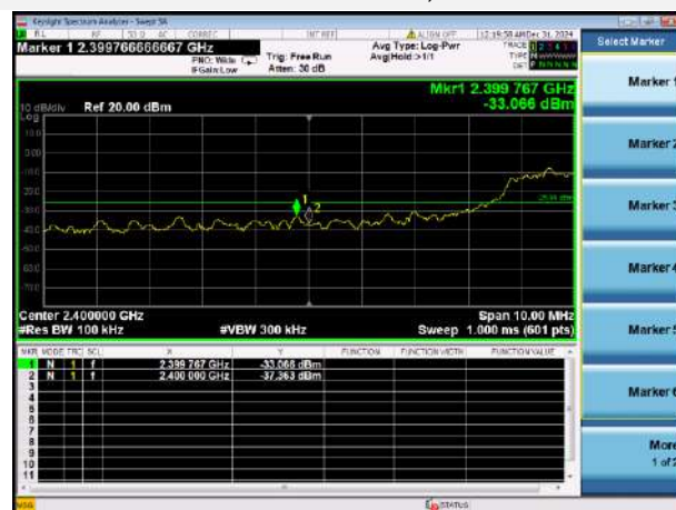
802.11n-40 MHz LOW CHANNEL, BAND EDGE
