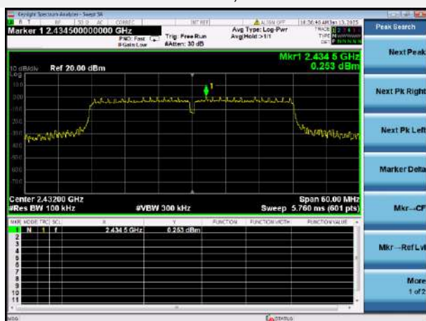
802.11n-40 MHz CHANNEL 5, CARRIER LEVEL
