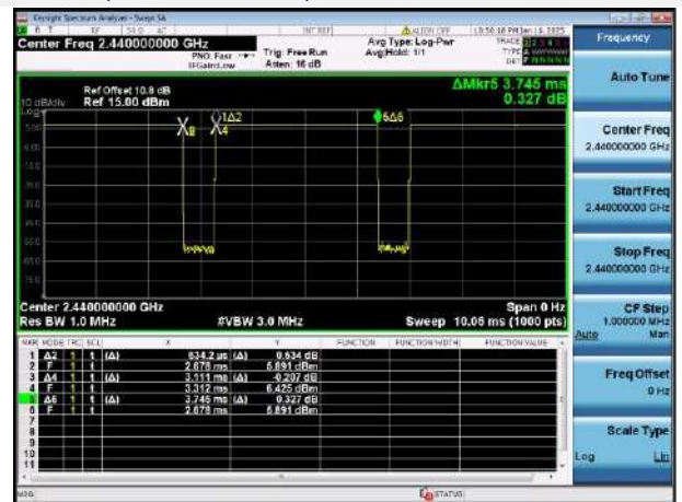
GFSK (BLE Coded S8)
