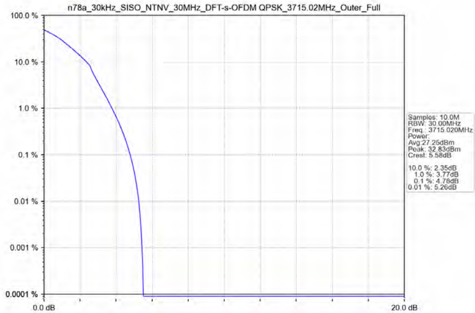
n78a_30kHz_SISO_NTNV_30MHz_DFT-s-OFDM QPSK 3715.02MHz_Outer_Full_Ant13
