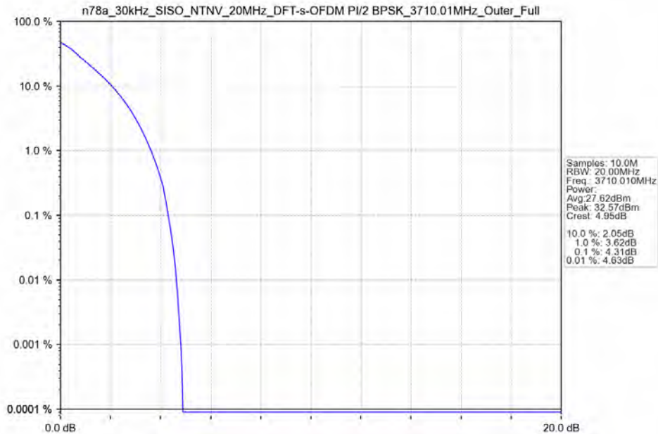
n78a_30kHz_SISO_NTNV_20MHz_DFT-s-OFDM PI/2 BPSK_3710.01MHz_Outer_Full_Ant13
