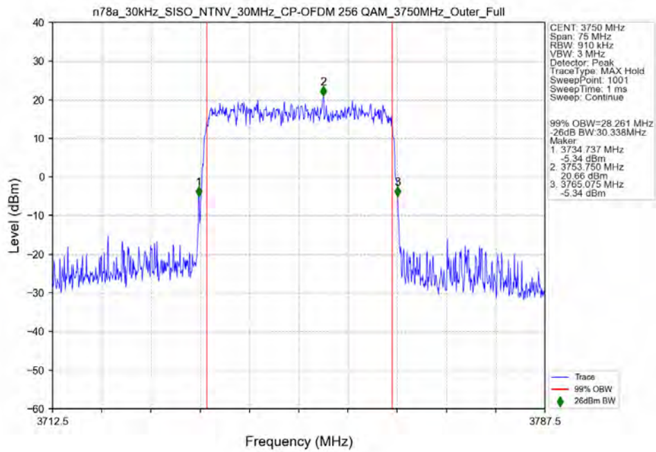
n78a_30kHz_SISO_NTNV_30MHz_CP-OFDM_256_QAM_3750MHz_Outer_Full_Ant13
