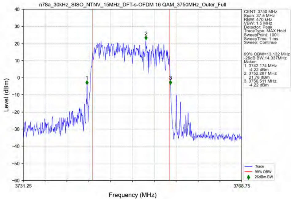
n78a_30kHz_SISO_NTNV_15MHz_DFT-s-OFDM_16_QAM_3750MHz_Outer_Full_Ant13
