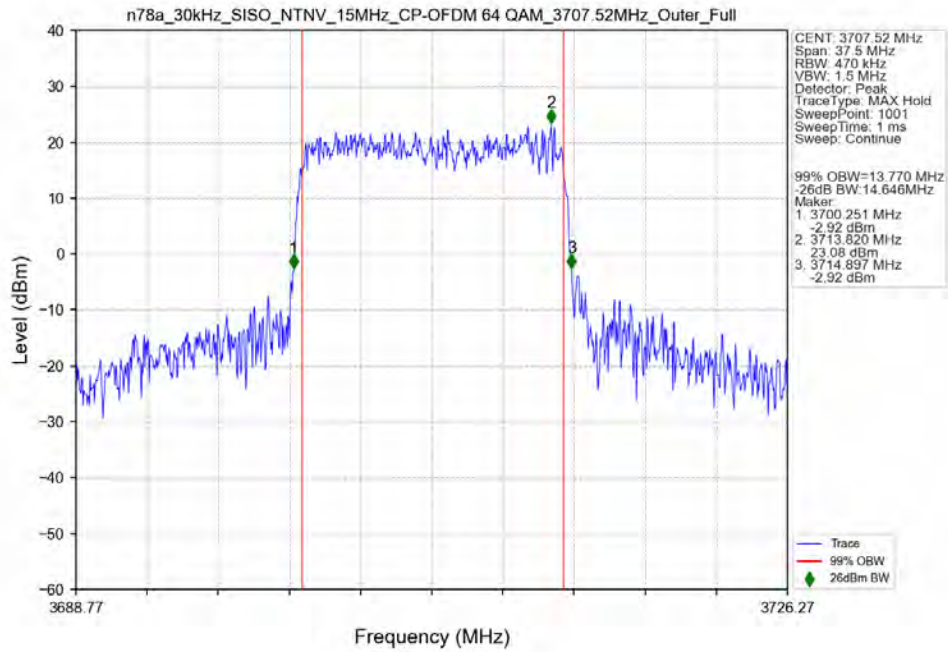
n78a_30kHz_SISO_NTNV_15MHz_CP-OFDM_64_QAM_3707.52MHz_Outer_Full_Ant13
