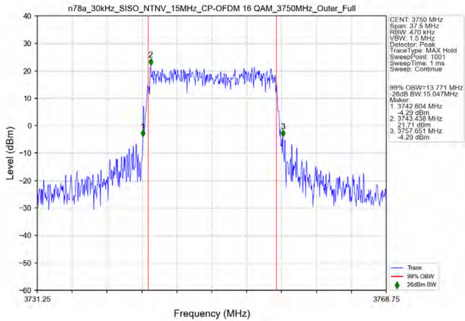
n78a_30kHz_SISO_NTNV_15MHz_CP-OFDM_16_QAM_3750MHz_Outer_Full_Ant13
