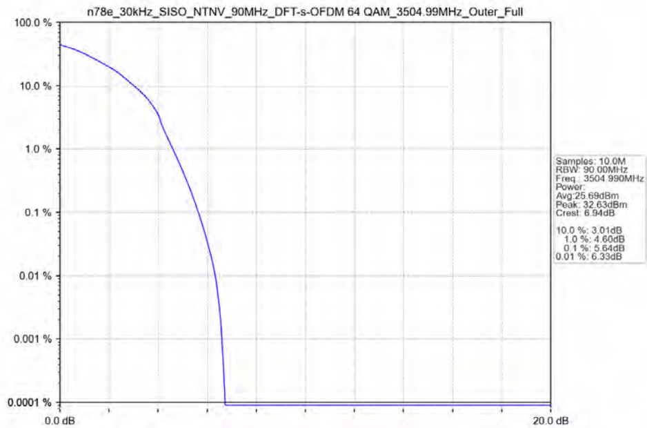
n78e_30kHz_SISO_NTNV_90MHz_DFT-s-OFDM_64_QAM_3504.99MHz_Outer_Full_Ant13
