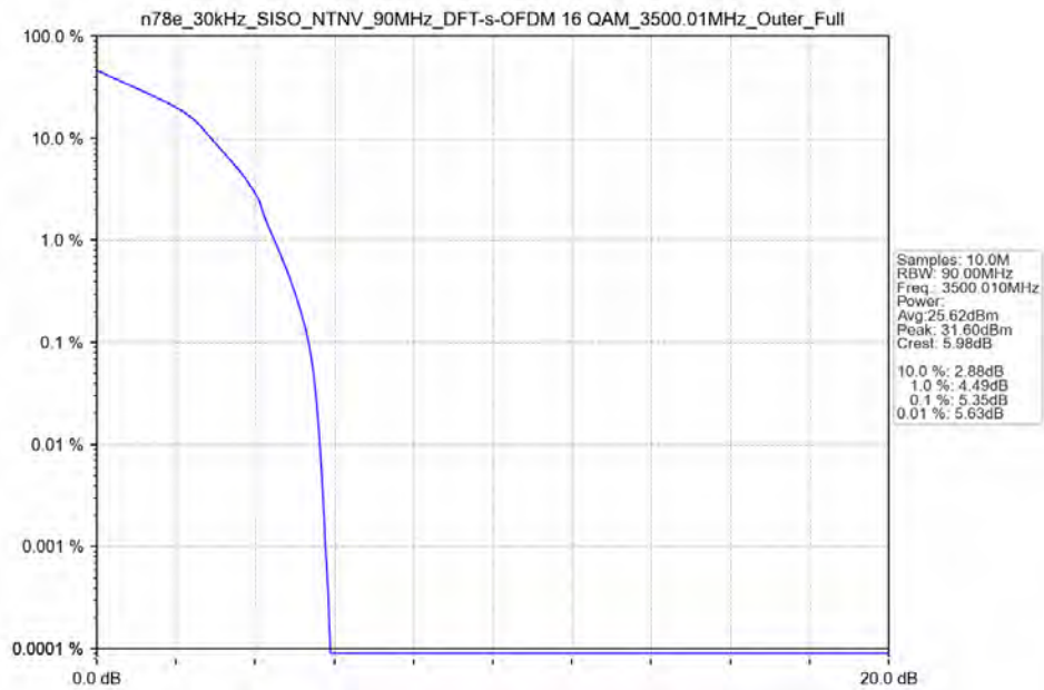
n78e_30kHz_SISO_NTNV_90MHz_DFT-s-OFDM_16_QAM_3500.01MHz_Outer_Full_Ant13
