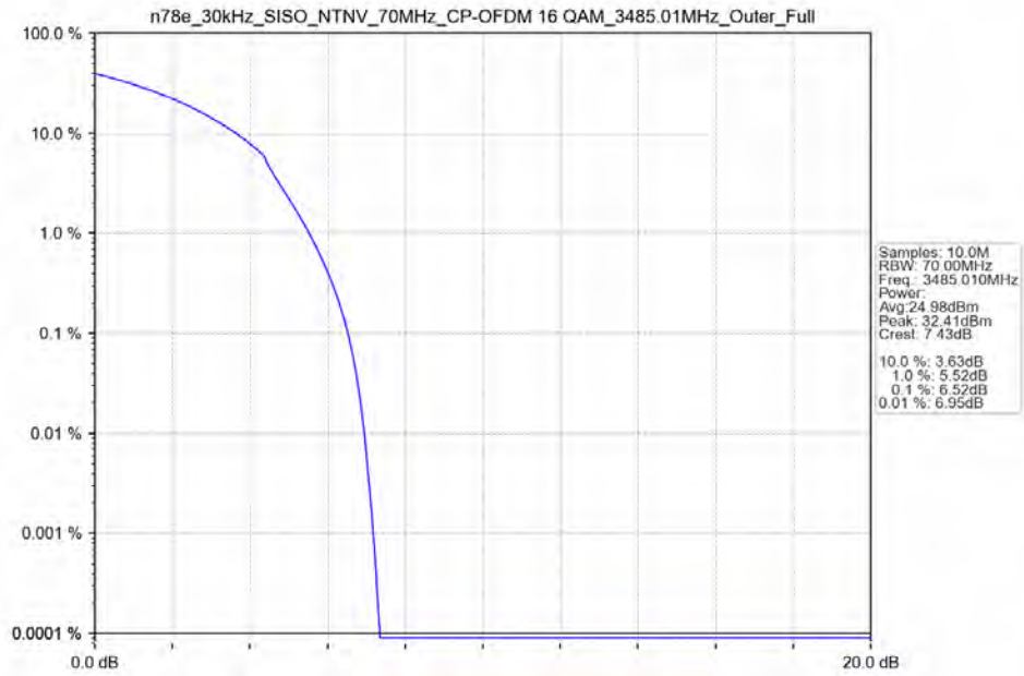
n78e_30kHz_SISO_NTNV_70MHz_CP-OFDM_16_QAM_3485.01MHz_Outer_Full_Ant13
