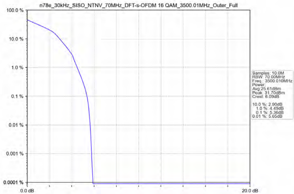
n78e_30kHz_SISO_NTNV_70MHz_DFT-s-OFDM_16_QAM_3500.01MHz_Outer_Full_Ant13
