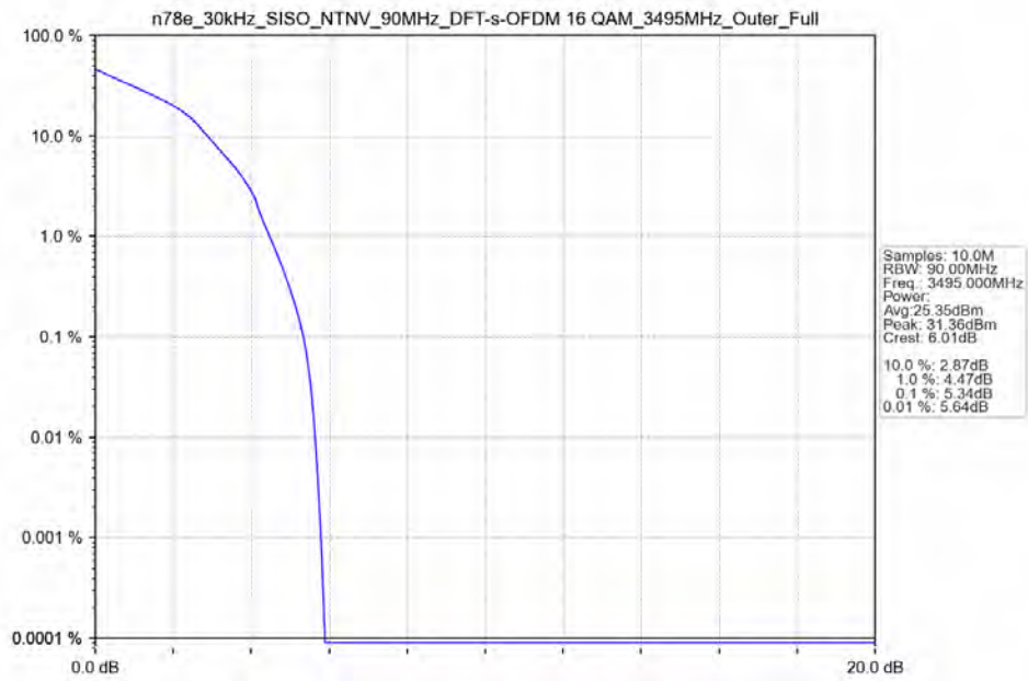
n78e_30kHz_SISO_NTNV_90MHz_DFT-s-OFDM_16_QAM_3495MHz_Outer_Full_Ant13
