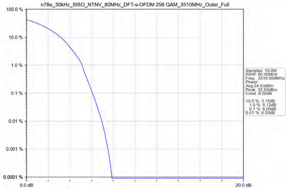
n78e_30kHz_SISO_NTNV_80MHz_DFT-s-OFDM_256_QAM_3510MHz_Outer_Full_Ant13
