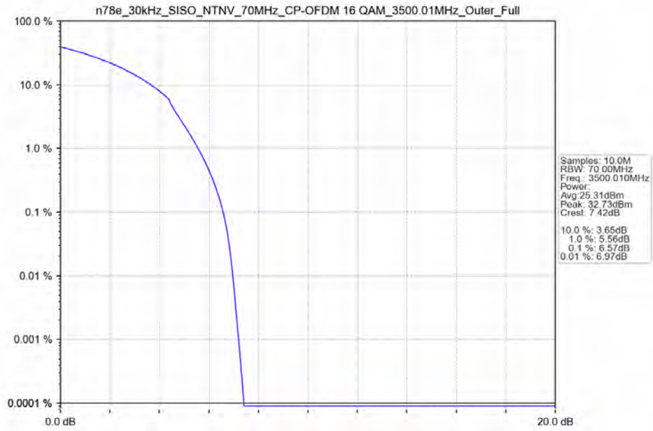
n78e_30kHz_SISO_NTNV_70MHz_CP-OFDM_16_QAM_3500.01MHz_Outer_Full_Ant13
