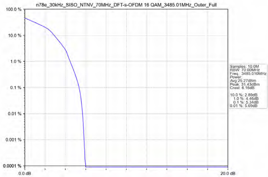
n78e_30kHz_SISO_NTNV_70MHz_DFT-s-OFDM_16_QAM_3485.01MHz_Outer_Full_Ant13
