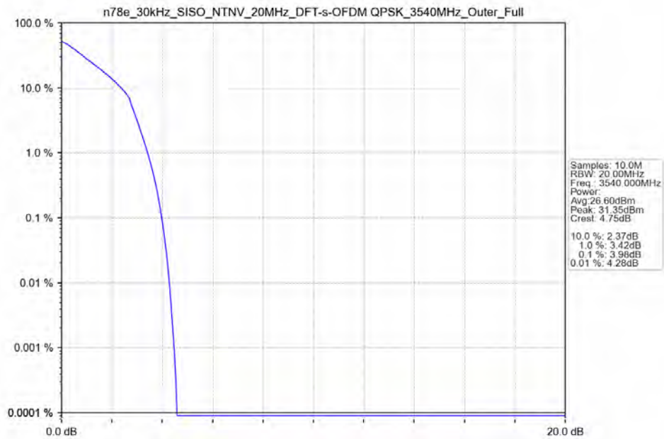
n78e_30kHz_SISO_NTNV_20MHz_DFT-s-OFDM_QPSK_3540MHz_Outer_Full_Ant13
