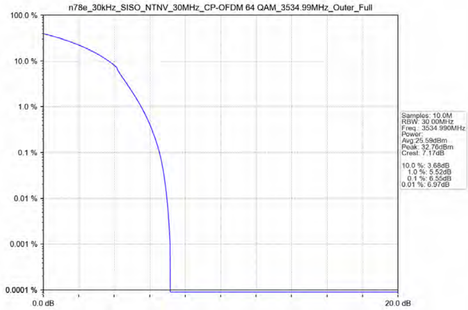
n78e_30kHz_SISO_NTNV_30MHz_CP-OFDM_64_QAM_3534.99MHz_Outer_Full_Ant13
