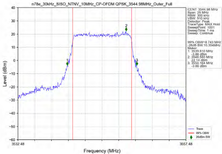
n78e_30kHz_SISO_NTNV_10MHz_CP-OFDM_QPSK_3544.98MHz_Outer_Full_Ant13
