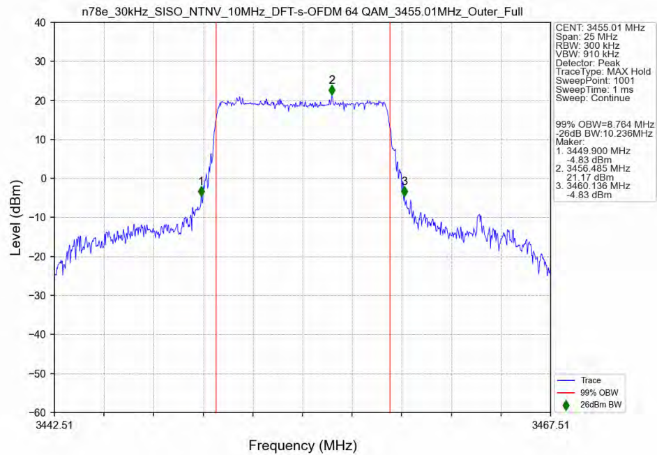
n78e_30kHz_SISO_NTNV_10MHz_DFT-s-OFDM_64_QAM_3455.01MHz_Outer_Full_Ant13
