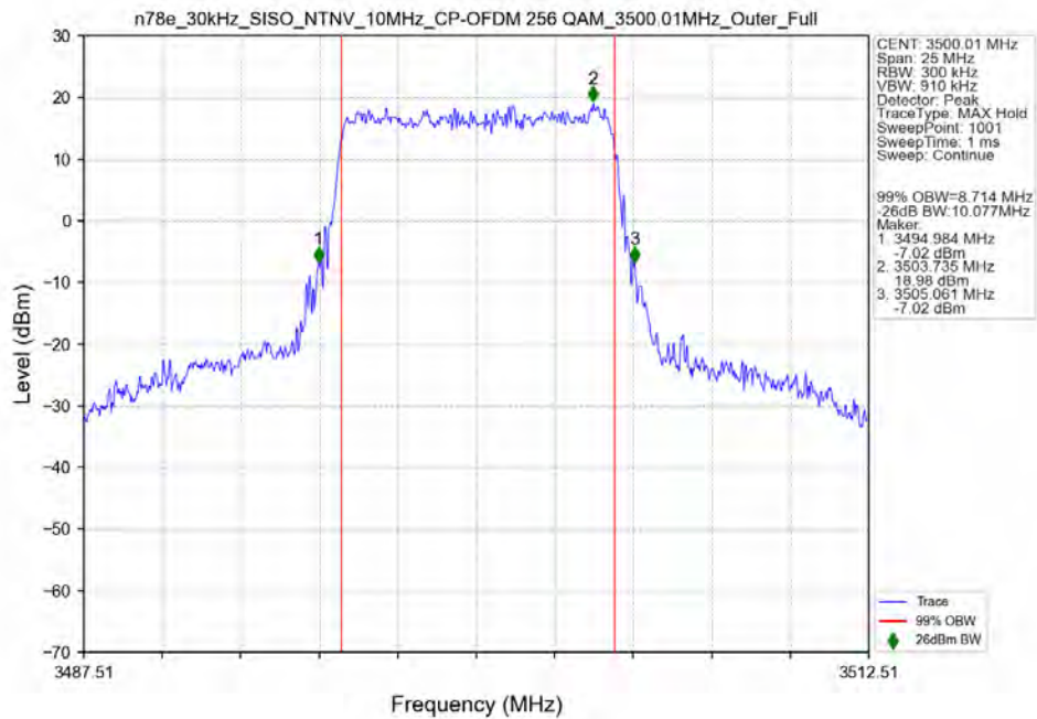
n78e_30kHz_SISO_NTNV_10MHz_CP-OFDM_256_QAM_3500.01MHz_Outer_Full_Ant13
