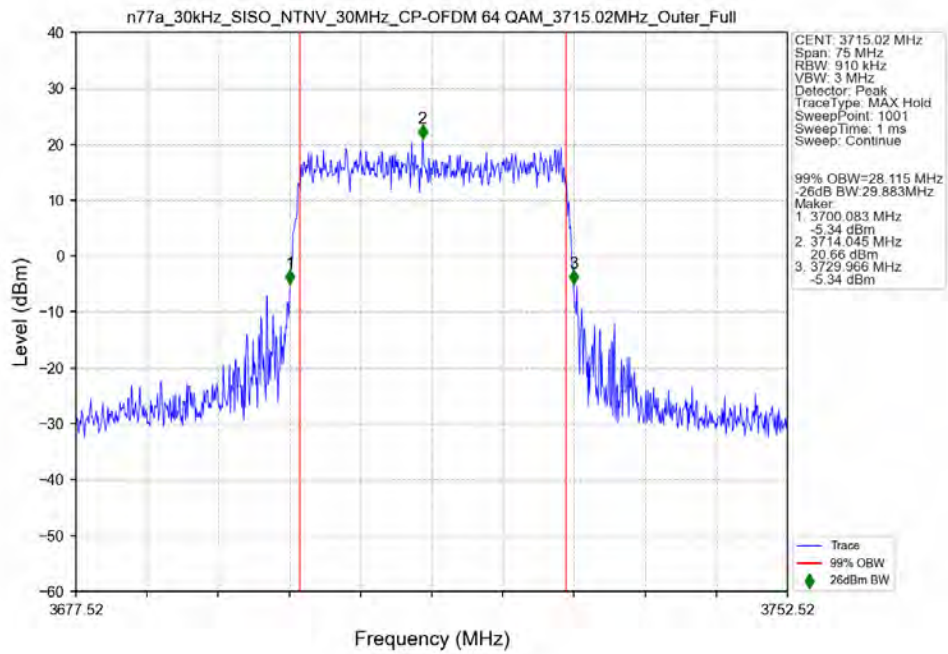
n77a_30kHz_SISO_NTNV_30MHz_CP-OFDM 64 QAM 3715.02MHz_Outer_Full_Ant13
