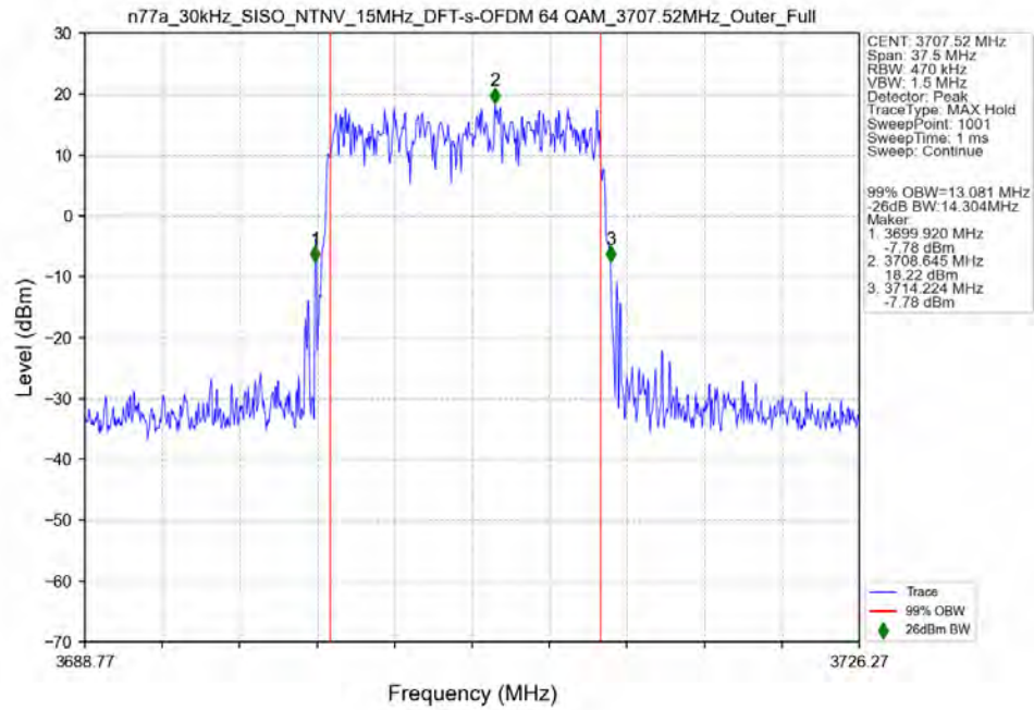
n77a_30kHz_SISO_NTNV_15MHz_DFT-s-OFDM_64_QAM_3707.52MHz_Outer_Full_Ant13
