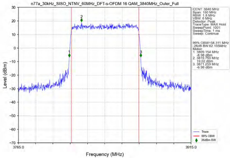
n77a_30kHz_SISO_NTNV_60MHz_DFT-s-OFDM_16_QAM_3840MHz_Outer_Full_Ant13
