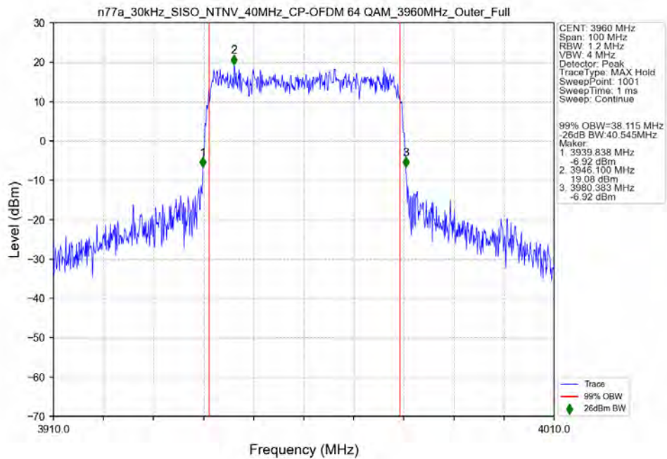
n77a_30kHz_SISO_NTNV_40MHz_CP-OFDM_64_QAM_3960MHz_Outer_Full_Ant13
