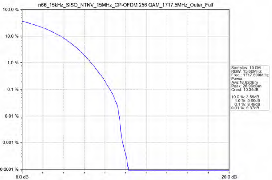
n66_15kHz_SISO_NTNV_15MHz_CP-OFDM_256_QAM_1717.5MHz_Outer_Full_Ant41
