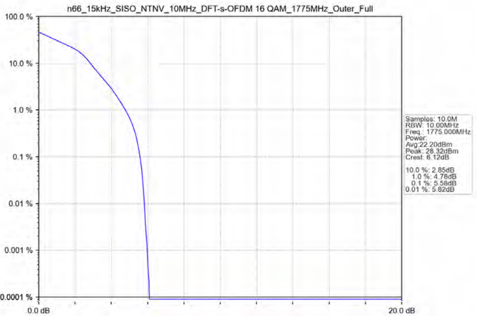
n66_15kHz_SISO_NTNV_10MHz_DFT-s-OFDM 16 QAM_1775MHz_Outer_Full_Ant41
