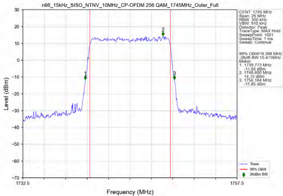
n66_15kHz_SISO_NTNV_10MHz_CP-OFDM_256_QAM_1745MHz_Outer_Full_Ant41
