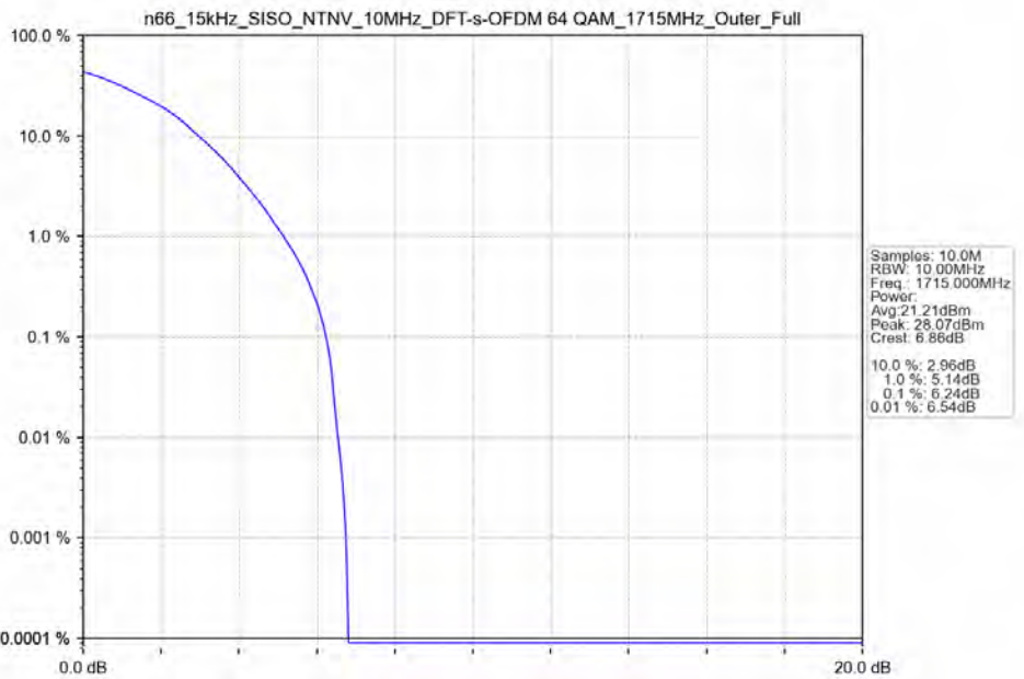
n66_15kHz_SISO_NTNV_10MHz_DFT-s-OFDM 64 QAM_1715MHz_Outer_Full_Ant41
