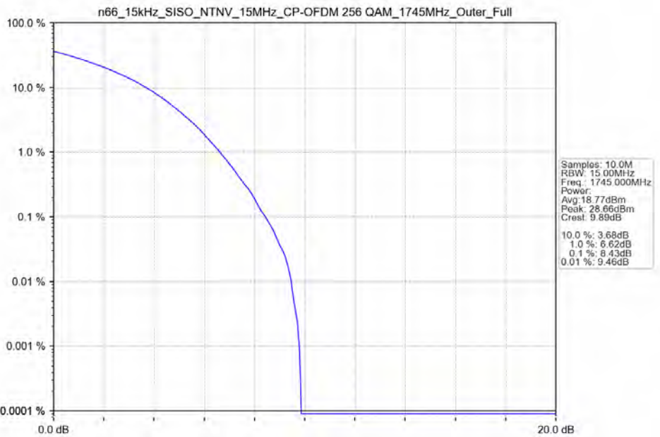
n66_15kHz_SISO_NTNV_15MHz_CP-OFDM_256_QAM_1745MHz_Outer_Full_Ant41
