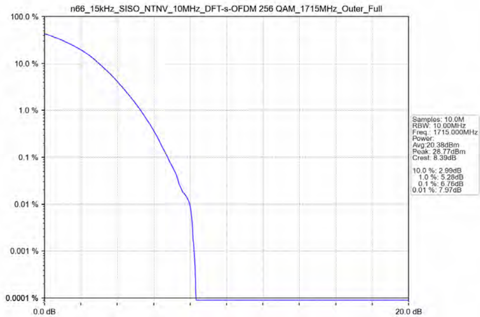
n66_15kHz_SISO_NTNV_10MHz_DFT-s-OFDM_256_QAM_1715MHz_Outer_Full_Ant41
