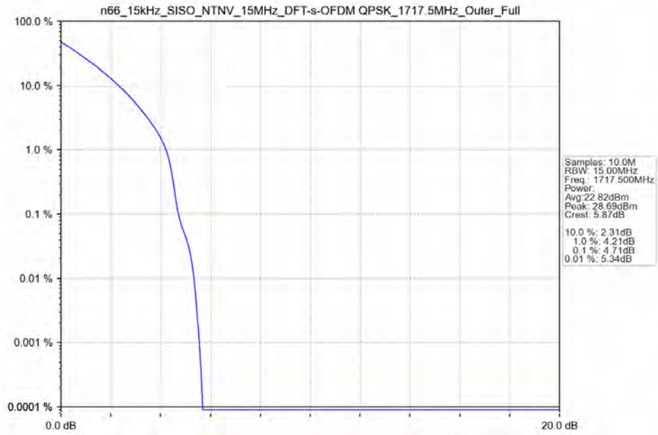
n66_15kHz_SISO_NTNV_15MHz_DFT-s-OFDM QPSK_1717.5MHz_Outer_Full_Ant41
