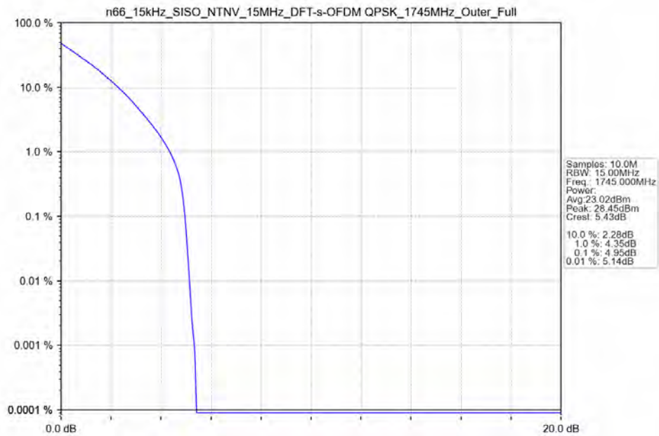
n66_15kHz_SISO_NTNV_15MHz_DFT-s-OFDM_QPSK_1745MHz_Outer_Full_Ant41
