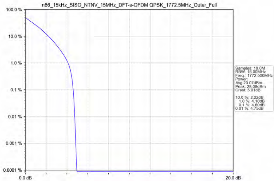
n66_15kHz_SISO_NTNV_15MHz_DFT-s-OFDM_QPSK_1772.5MHz_Outer_Full_Ant41
