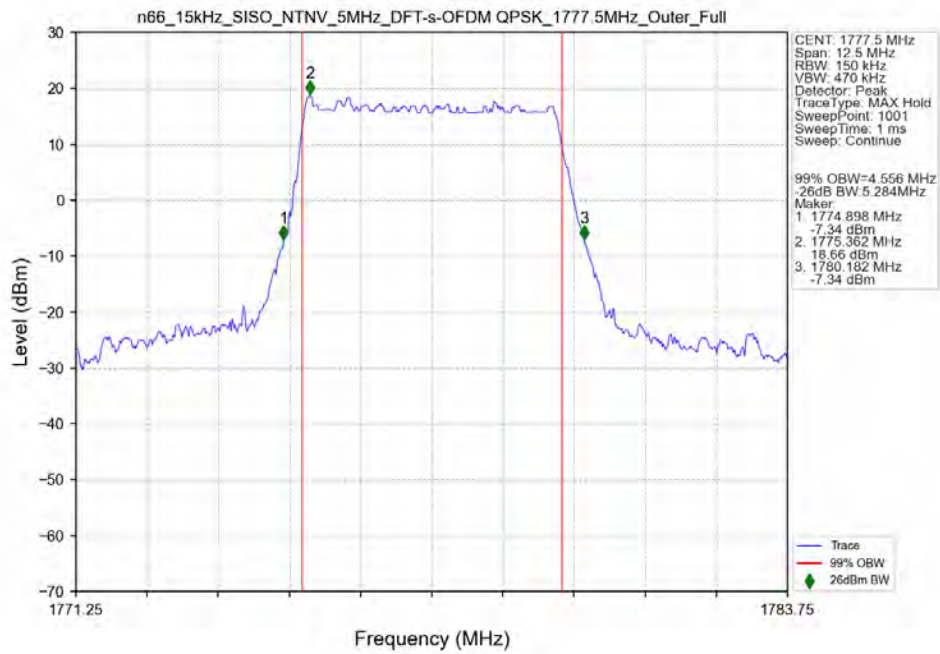
n66_15kHz_SISO_NTNV_5MHz_DFT-s-OFDM_QPSK_1777.5MHz_Outer_Full_Ant41
