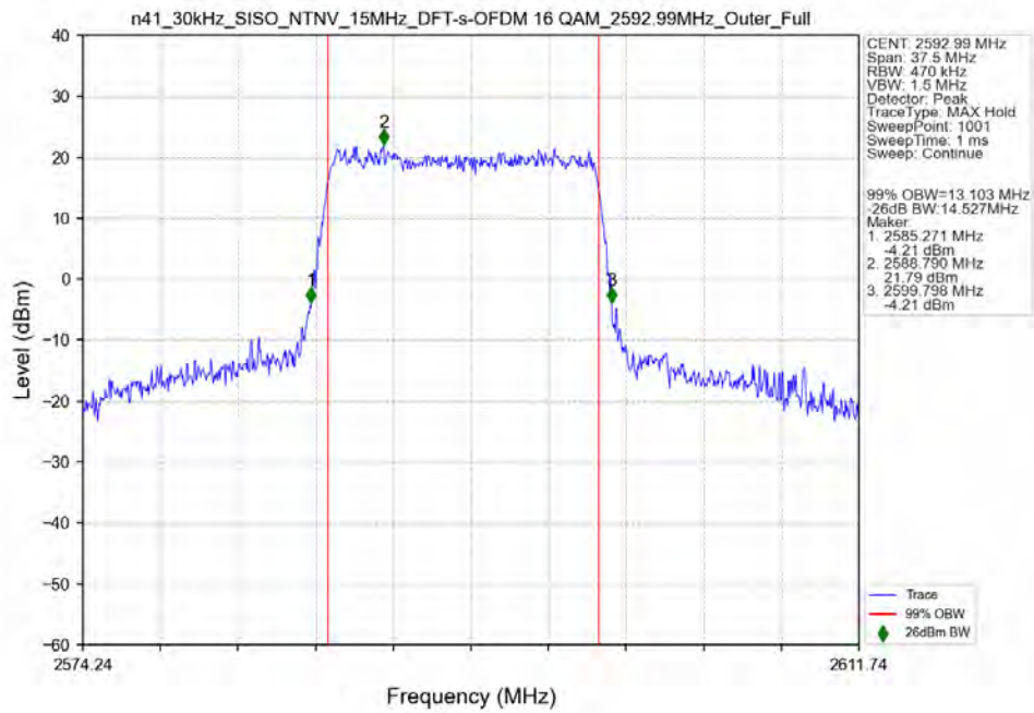
n41_30kHz_SISO_NTNV_15MHz_DFT-s-OFDM_16_QAM_2592.99MHz_Outer_Full_Ant41
