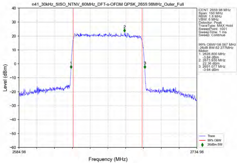
n41_30kHz_SISO_NTNV_60MHz_DFT-s-OFDM_QPSK_2659.98MHz_Outer_Full_Ant41
