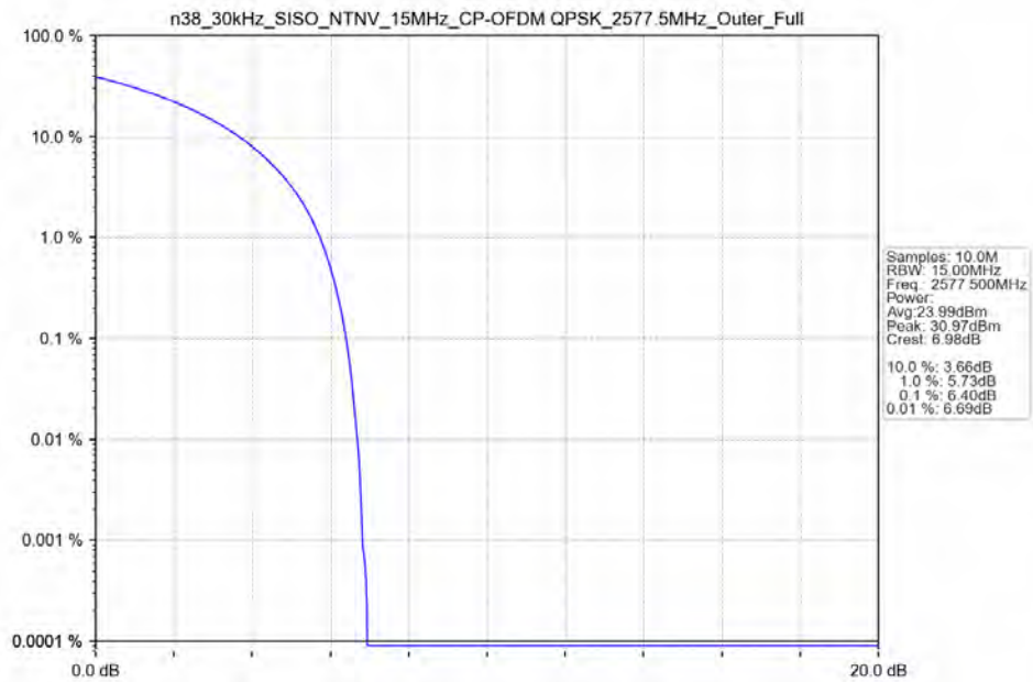
n38_30kHz_SISO_NTNV_15MHz_CP-OFDM_QPSK_2577.5MHz_Outer_Full_Ant41
