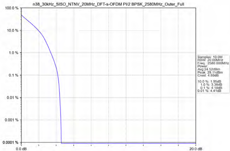
n38_30kHz_SISO_NTNV_20MHz_DFT-s-OFDM PI/2 BPSK_2580MHz_Outer_Full_Ant41
