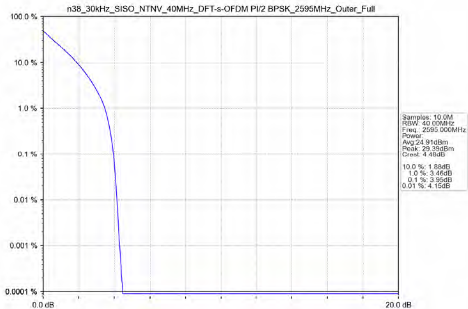
n38_30kHz_SISO_NTNV_40MHz_DFT-s-OFDM PI/2 BPSK_2595MHz_Outer_Full_Ant41
