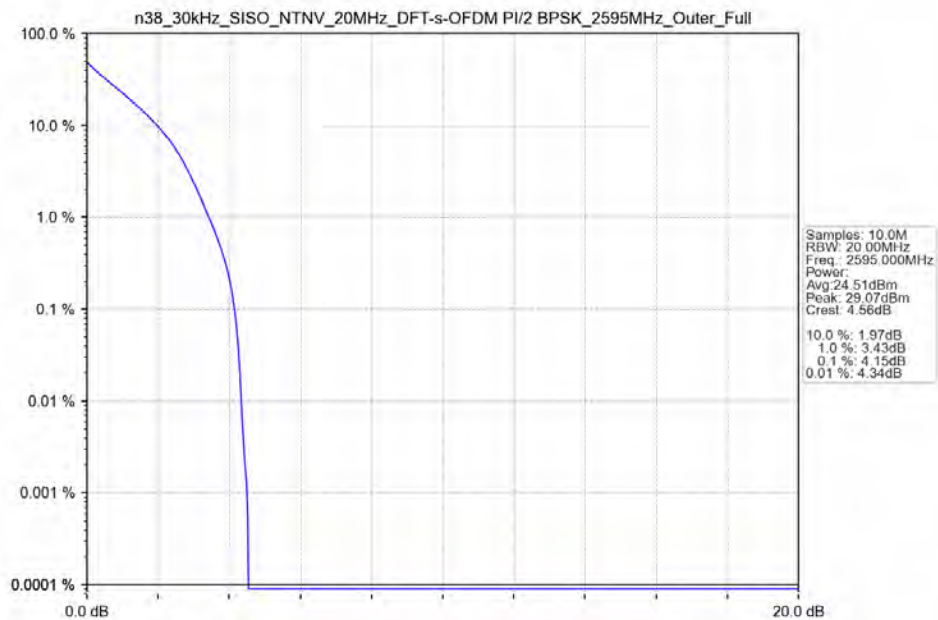
n38_30kHz_SISO_NTNV_20MHz_DFT-s-OFDM PI/2 BPSK_2595MHz_Outer_Full_Ant41
