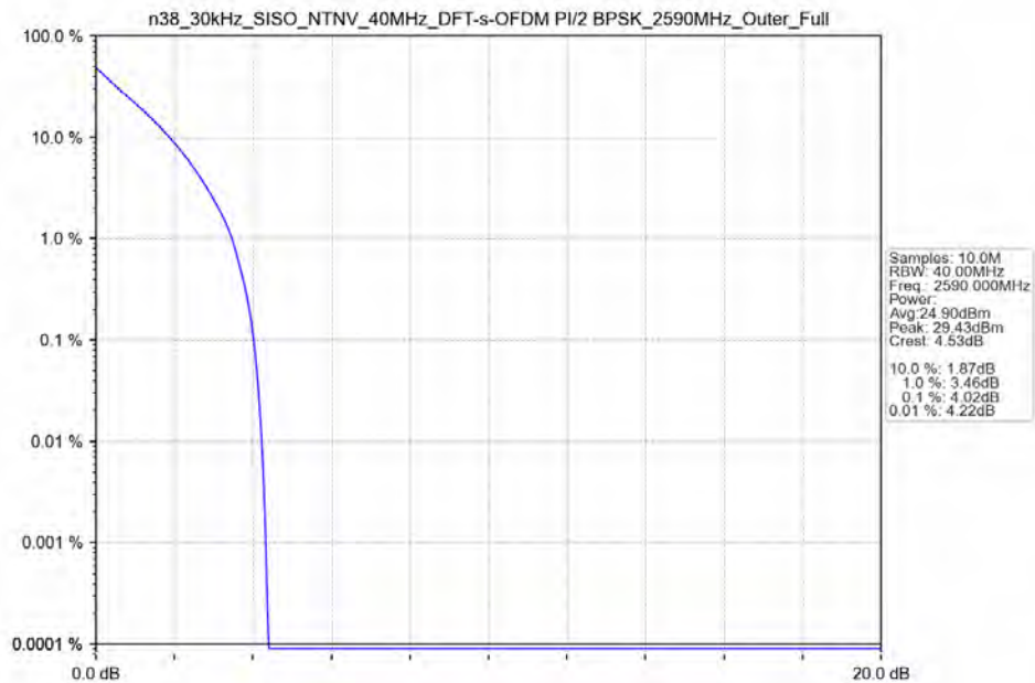
n38_30kHz_SISO_NTNV_40MHz_DFT-s-OFDM PI/2 BPSK_2590MHz_Outer_Full_Ant41
