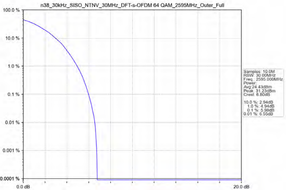
n38_30kHz_SISO_NTNV_30MHz_DFT-s-OFDM_64_QAM_2595MHz_Outer_Full_Ant41
