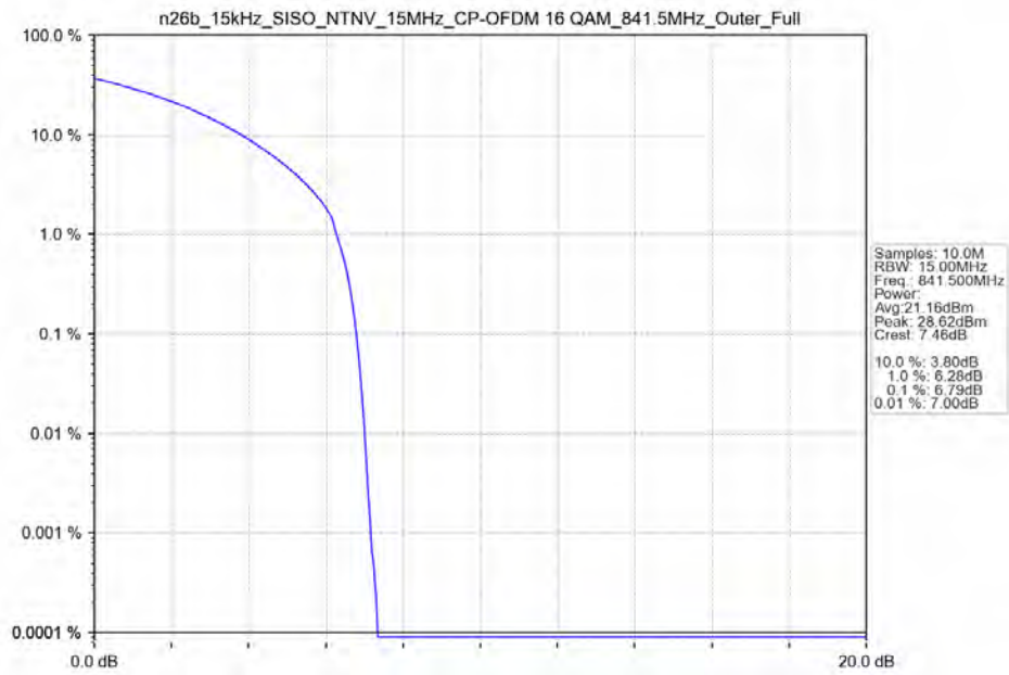
n26b_15kHz_SISO_NTNV_15MHz_CP-OFDM 16 QAM_841.5MHz_Outer_Full_Ant31
