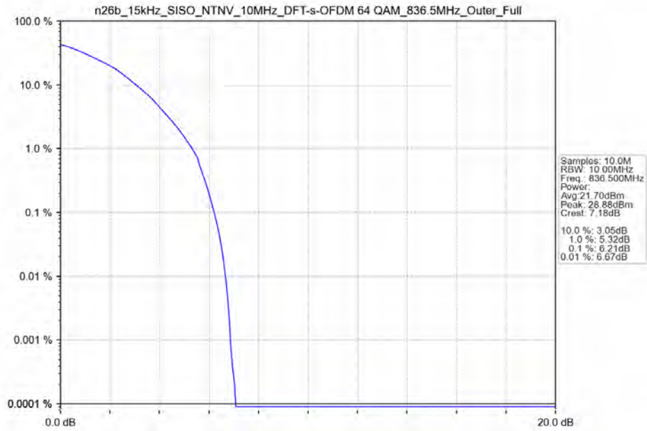
n26b_15kHz_SISO_NTNV_10MHz_DFT-s-OFDM 64 QAM_836.5MHz_Outer_Full_Ant31
