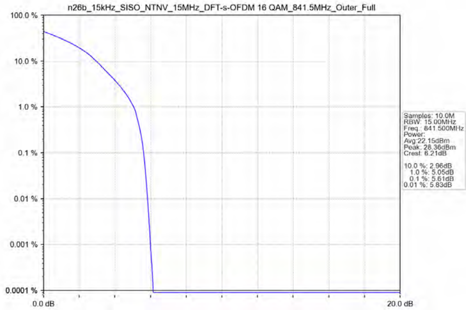
n26b_15kHz_SISO_NTNV_15MHz_DFT-s-OFDM_16_QAM_841.5MHz_Outer_Full_Ant31
