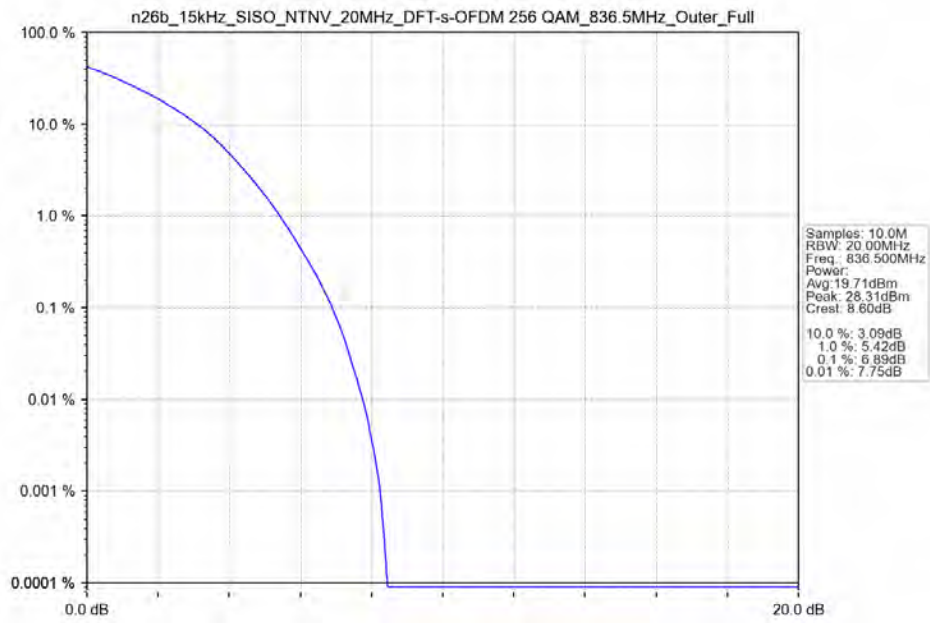
n26b_15kHz_SISO_NTNV_20MHz_DFT-s-OFDM_256_QAM_836.5MHz_Outer_Full_Ant31
