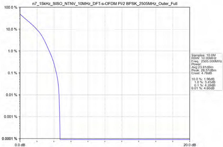
n7_15kHz_SISO_NTNV_10MHz_DFT-s-OFDM PI/2 BPSK_2505MHz_Outer_Full_Ant41
