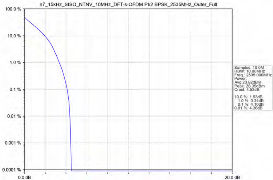
n7_15kHz_SISO_NTNV_10MHz_DFT-s-OFDM PI/2 BPSK_2535MHz_Outer_Full_Ant41
