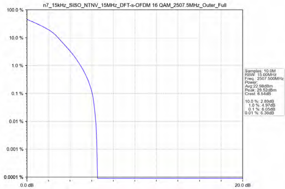
n7_15kHz_SISO_NTNV_15MHz_DFT-s-OFDM_16_QAM_2507.5MHz_Outer_Full_Ant41
