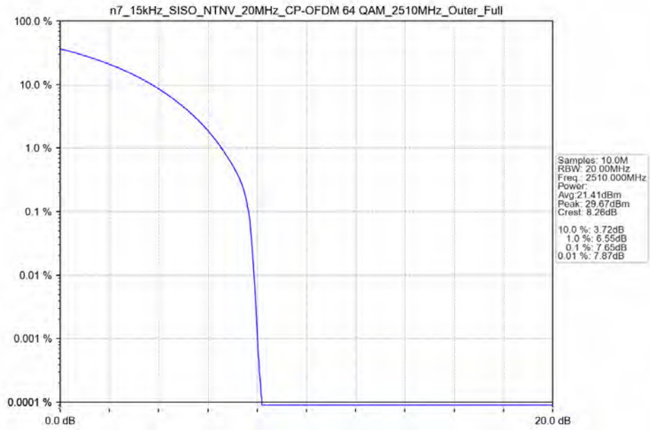
n7_15kHz_SISO_NTNV_20MHz_CP-OFDM 64 QAM_2510MHz_Outer_Full_Ant41
