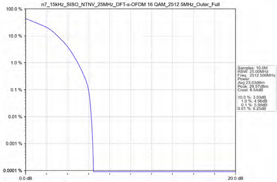
n7_15kHz_SISO_NTNV_25MHz_DFT-s-OFDM_16_QAM_2512.5MHz_Outer_Full_Ant41
