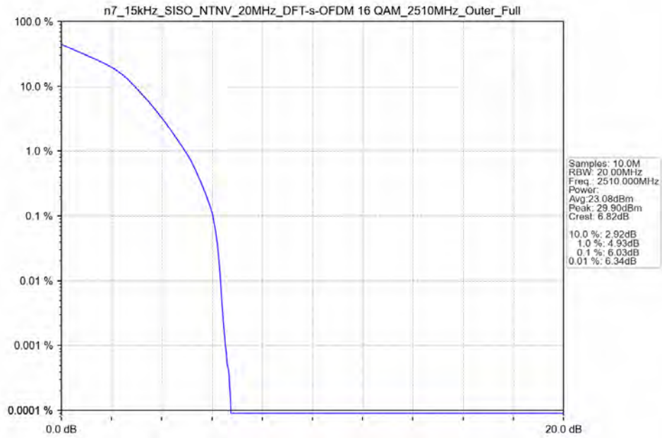
n7_15kHz_SISO_NTNV_20MHz_DFT-s-OFDM_16_QAM_2510MHz_Outer_Full_Ant41
