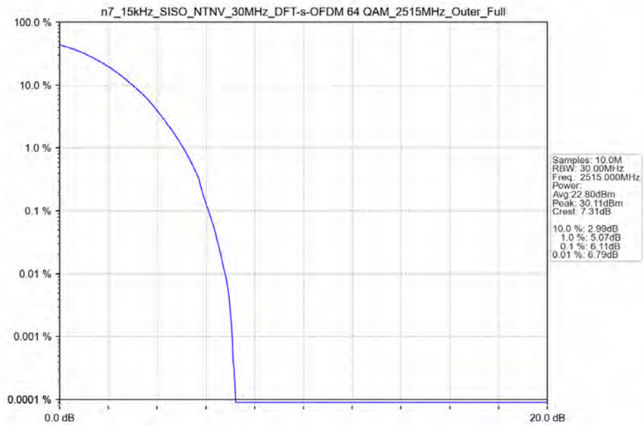
n7_15kHz_SISO_NTNV_30MHz_DFT-s-OFDM_64_QAM_2515MHz_Outer_Full_Ant41
