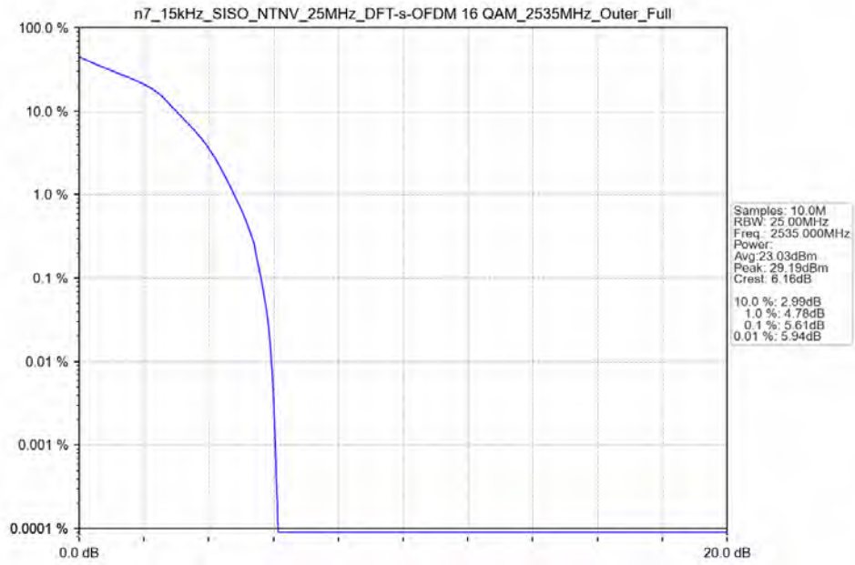
n7_15kHz_SISO_NTNV_25MHz_DFT-s-OFDM_16_QAM_2535MHz_Outer_Full_Ant41
