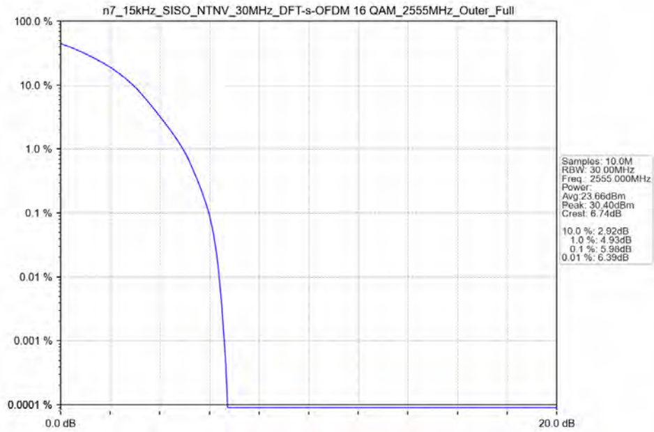
n7_15kHz_SISO_NTNV_30MHz_DFT-s-OFDM_16_QAM_2555MHz_Outer_Full_Ant41
