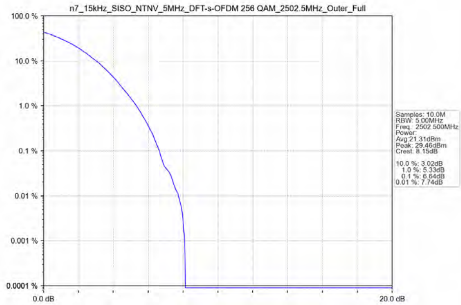
n7_15kHz_SISO_NTNV_5MHz_DFT-s-OFDM_256_QAM_2502.5MHz_Outer_Full_Ant41
