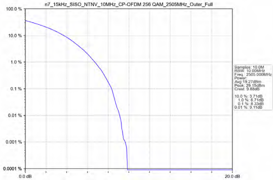
n7_15kHz_SISO_NTNV_10MHz_CP-OFDM_256_QAM_2505MHz_Outer_Full_Ant41
