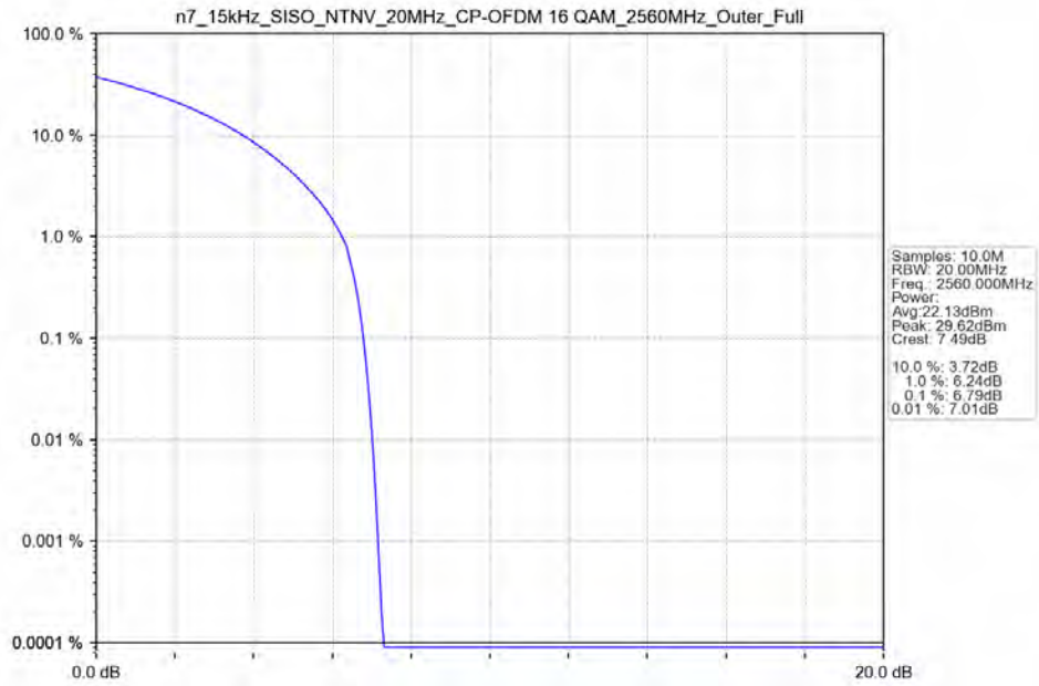
n7_15kHz_SISO_NTNV_20MHz_CP-OFDM 16 QAM_2560MHz_Outer_Full_Ant41
