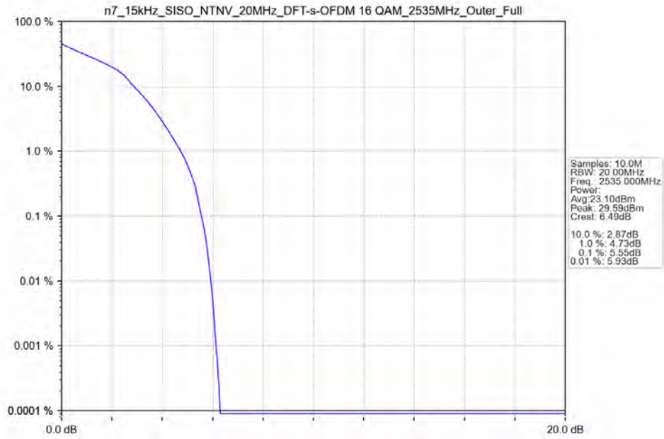
n7_15kHz_SISO_NTNV_20MHz_DFT-s-OFDM_16_QAM_2535MHz_Outer_Full_Ant41
