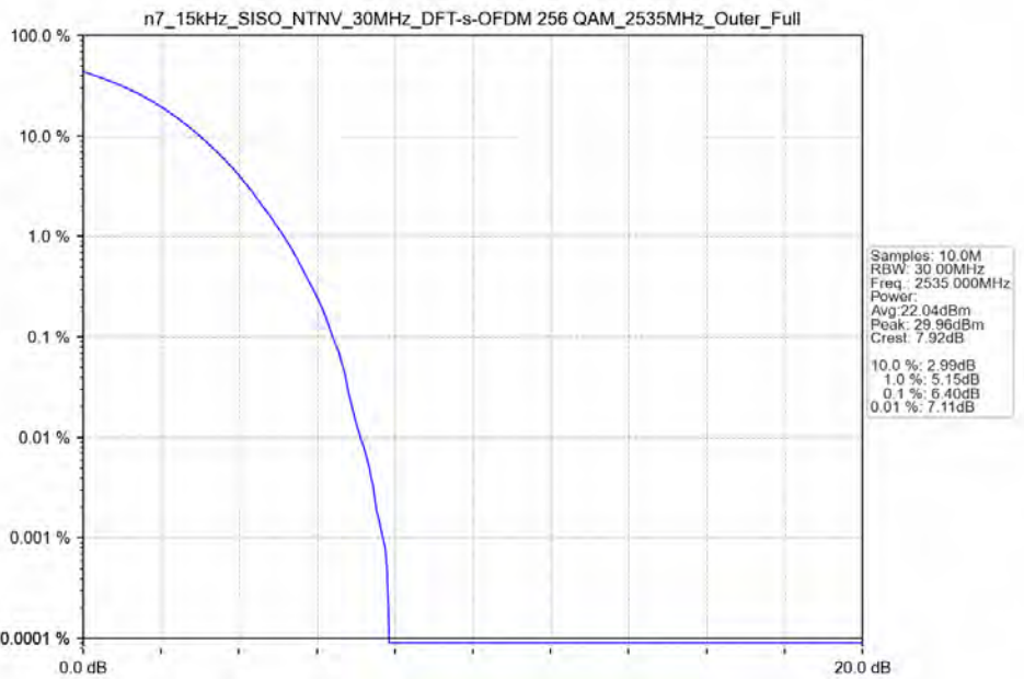
n7_15kHz_SISO_NTNV_30MHz_DFT-s-OFDM_256_QAM_2535MHz_Outer_Full_Ant41
