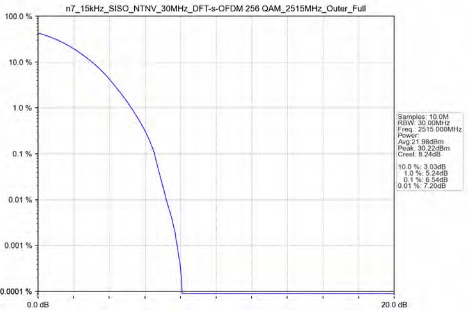
n7_15kHz_SISO_NTNV_30MHz_DFT-s-OFDM_256_QAM_2515MHz_Outer_Full_Ant41
