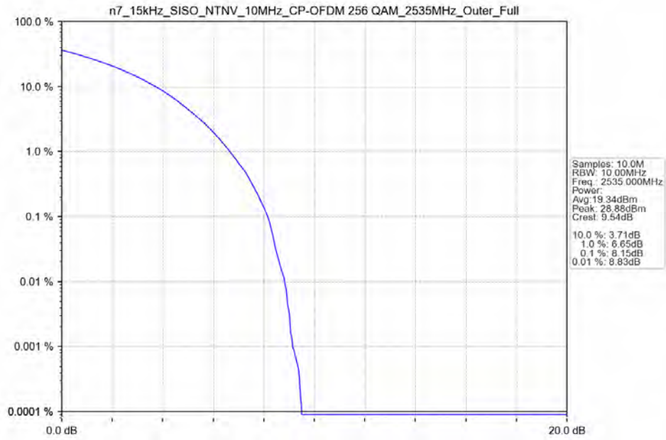
n7_15kHz_SISO_NTNV_10MHz_CP-OFDM_256_QAM_2535MHz_Outer_Full_Ant41
