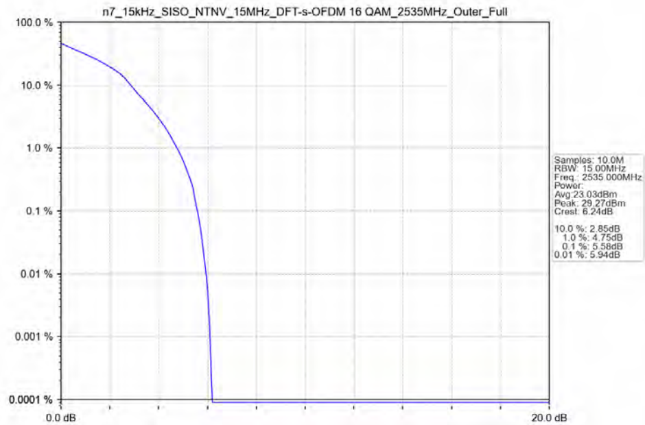
n7_15kHz_SISO_NTNV_15MHz_DFT-s-OFDM_16_QAM_2535MHz_Outer_Full_Ant41
