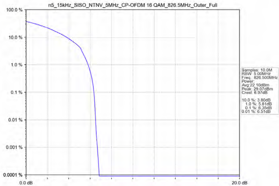
n5_15kHz_SISO_NTNV_5MHz_CP-OFDM_16_QAM_826.5MHz_Outer_Full_Ant11
