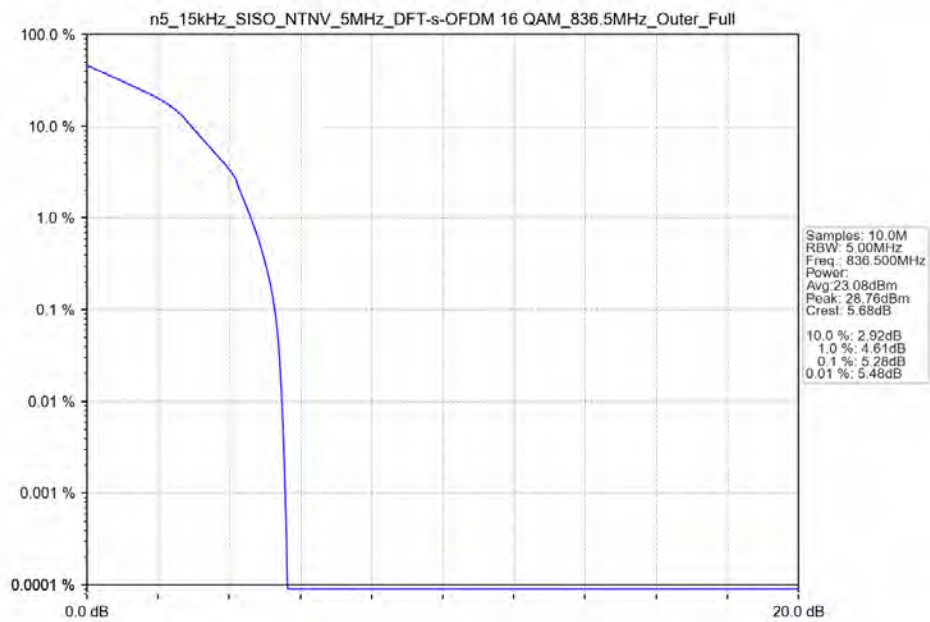
n5_15kHz_SISO_NTNV_5MHz_DFT-s-OFDM_16_QAM_836.5MHz_Outer_Full_Ant11
