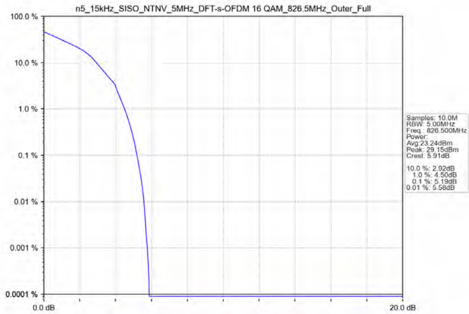
n5_15kHz_SISO_NTNV_5MHz_DFT-s-OFDM_16_QAM_826.5MHz_Outer_Full_Ant11
