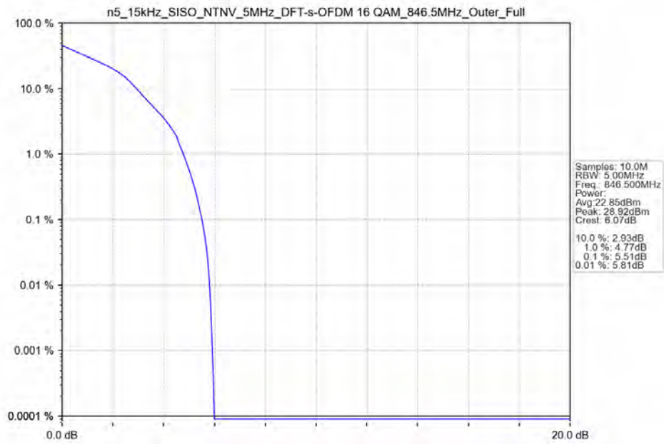
n5_15kHz_SISO_NTNV_5MHz_DFT-s-OFDM 16 QAM_846.5MHz_Outer_Full_Ant11
