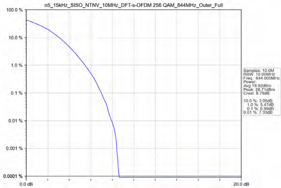
n5_15kHz_SISO_NTNV_10MHz_DFT-s-OFDM_256_QAM_844MHz_Outer_Full_Ant11
