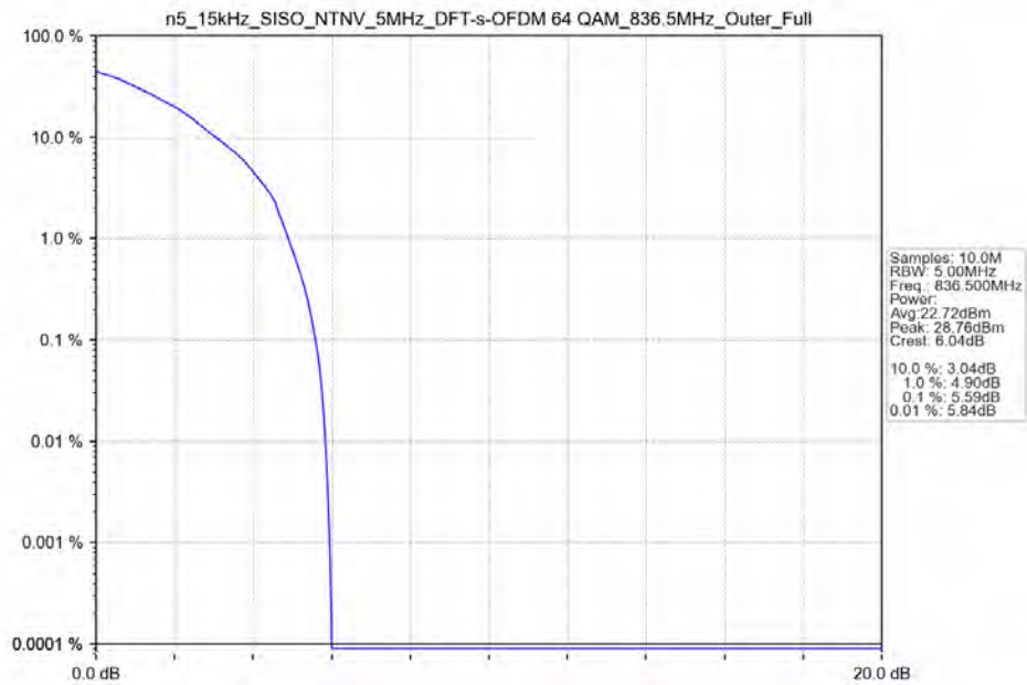
n5_15kHz_SISO_NTNV_5MHz_DFT-s-OFDM_64_QAM_836.5MHz_Outer_Full_Ant11
