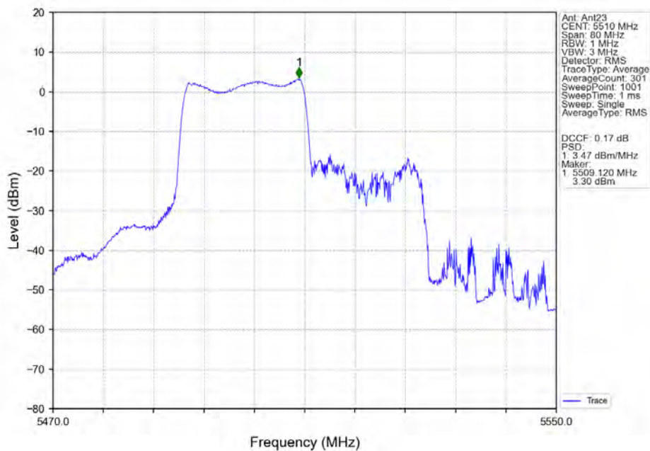
802.11ax(HEW40)_LCH_5510MHz_RU242_Left_Ant23_NTNV
