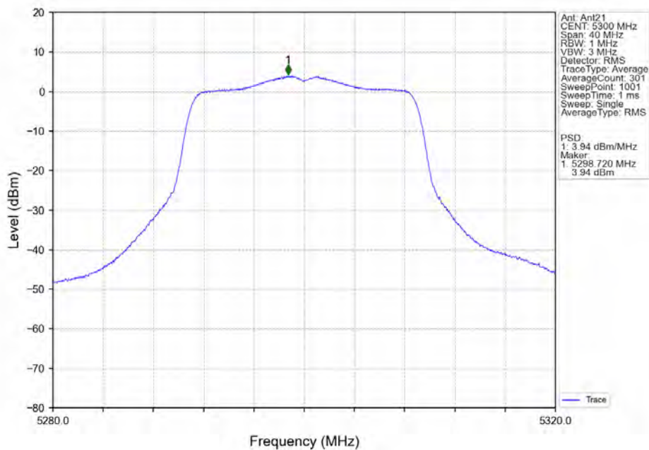
802.11ac(VHT20)_MCH_5300MHz_Ant21_NTNV
