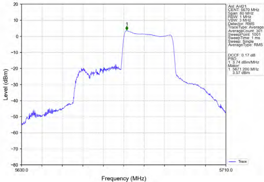
802.11ax(HEW40)_HCH_5670MHz_RU242_Right_MIMO_NTNV
