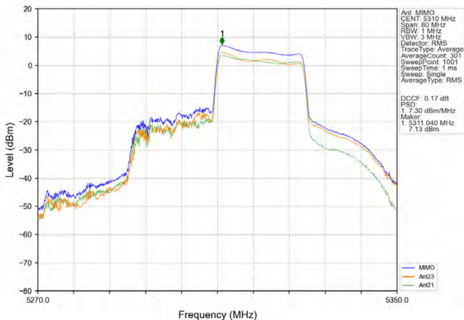
802.11ax(HEW40)_HCH_5310MHz_RU242_Right_MIMO_NTNV
