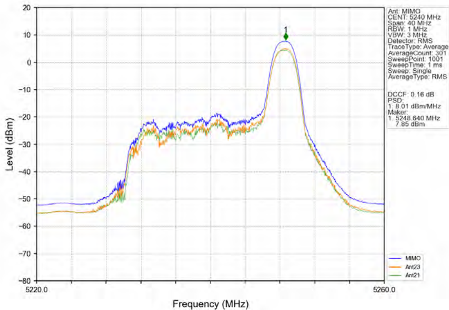
802.11ax(HEW20)_HCH_5240MHz_RU26_Right_MIMO_NTNV
