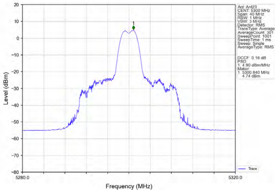
802.11ax(HEW20)_MCH_5300MHz_RU26_Mid_Ant23_NTNV
