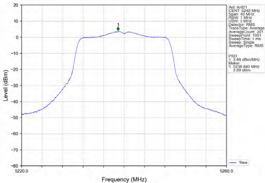
802.11ac(VHT20)_HCH_5240MHz_Ant21_NTNV
