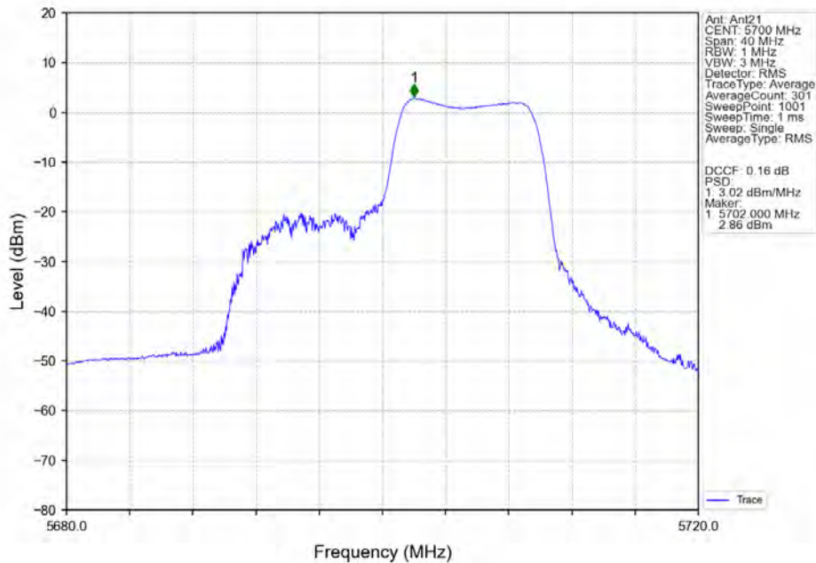
802.11ax(HEW20)_HCH_5700MHz_RU106_Right_MIMO_NTNV
