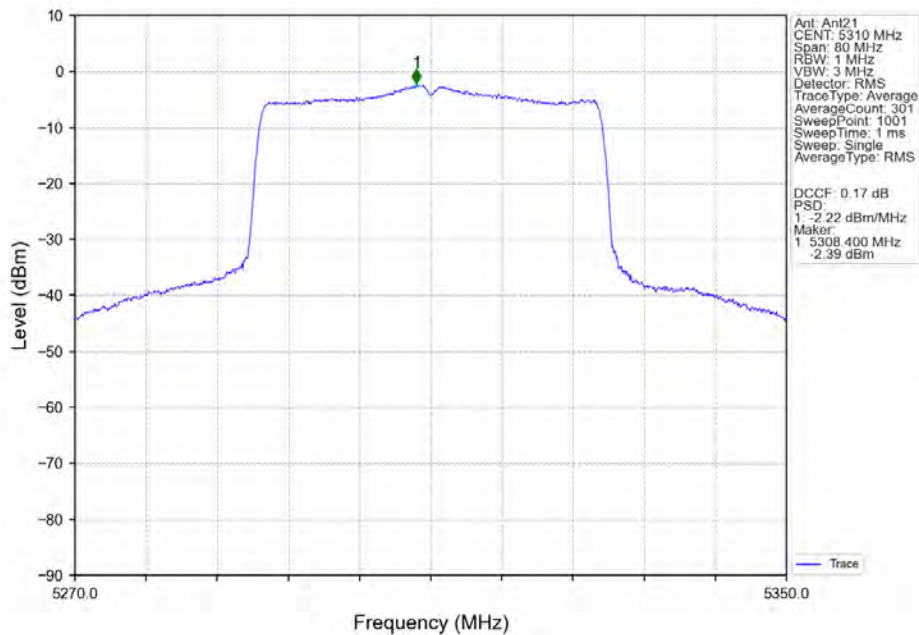
802.11ax(HEW40)_HCH_5310MHz_SU_/_Ant21_NTNV
