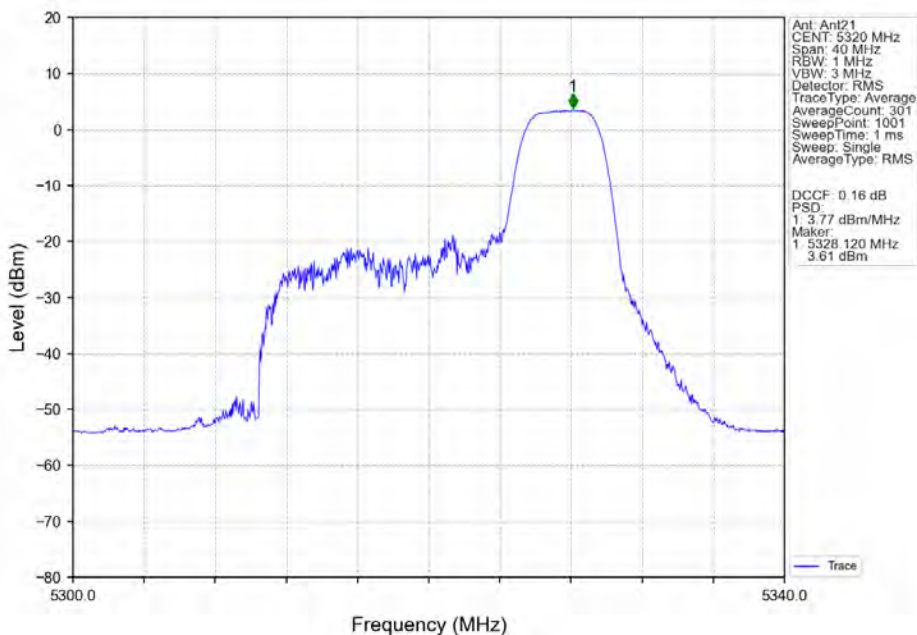
802.11ax(HEW20)_HCH_5320MHz_RU52_Right_Ant21_NTNV
