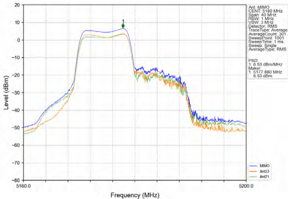
802.11ax(HEW20)_LCH_5180MHz_RU106_Left_MIMO_NTNV
