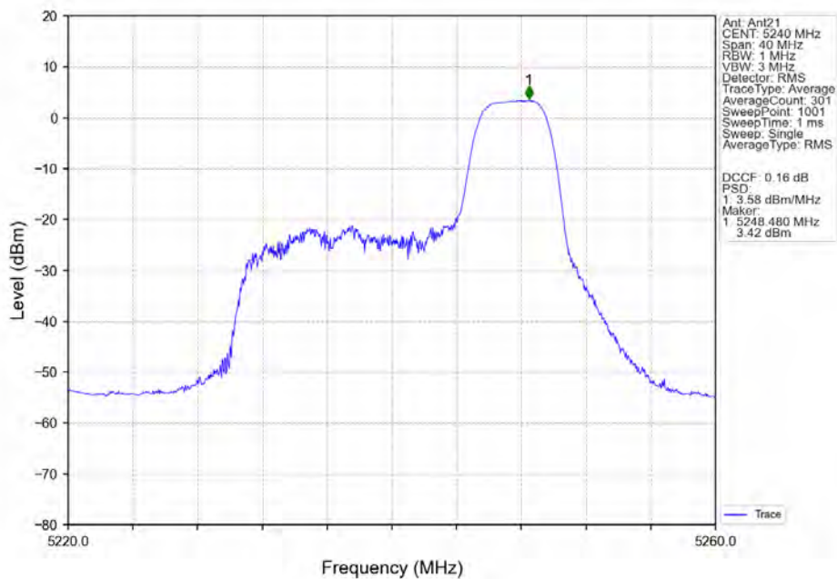
802.11ax(HEW20)_HCH_5240MHz_RU52_Right_Ant21_NTNV
