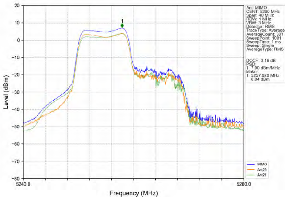
802.11ax(HEW20)_LCH_5260MHz_RU106_Left_MIMO_NTNV
