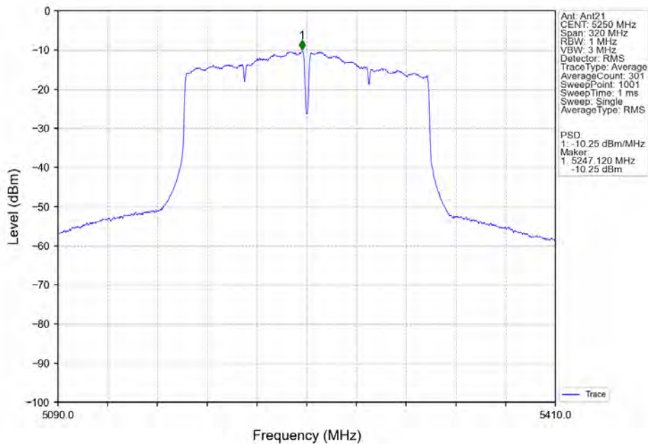
802.11ac(VHT160)_MCH_5250MHz_Ant21_NTNV
