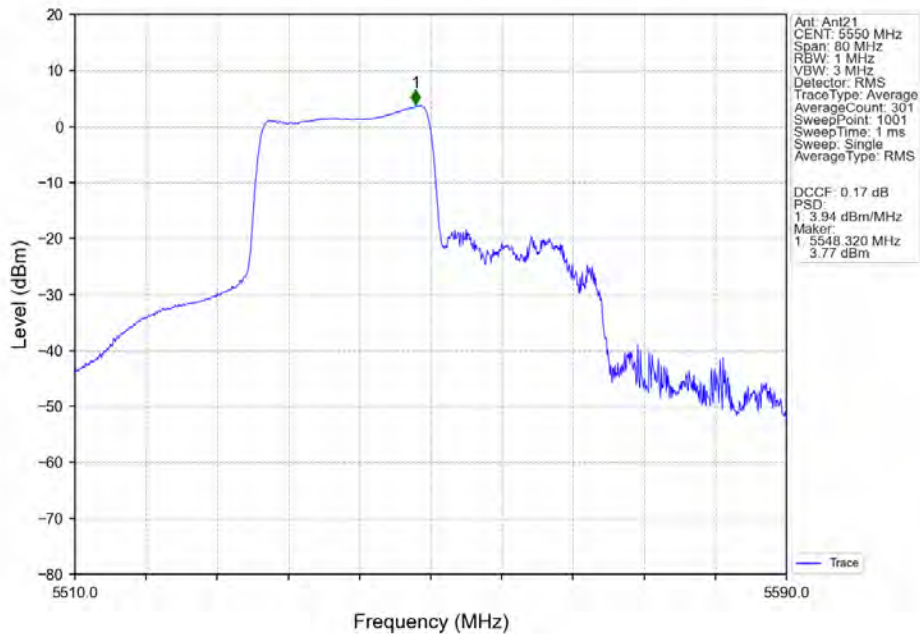
802.11ax(HEW40)_MCH_5550MHz_RU242_Left_MIMO_NTNV
