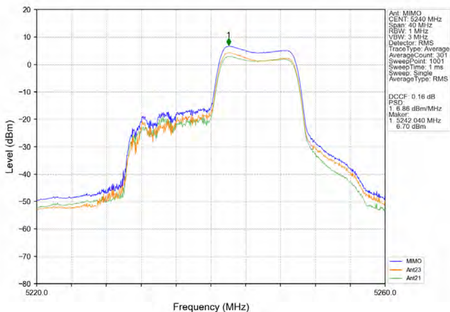
802.11ax(HEW20)_HCH_5240MHz_RU106_Right_MIMO_NTNV
