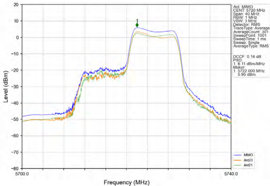
802.11ax(HEW20)_HCH_5720MHz_RU106_Right_MIMO_NTNV
