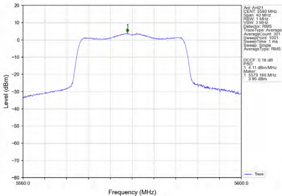
802.11ax(HEW20)_MCH_5580MHz_SU_/_Ant21_NTNV
