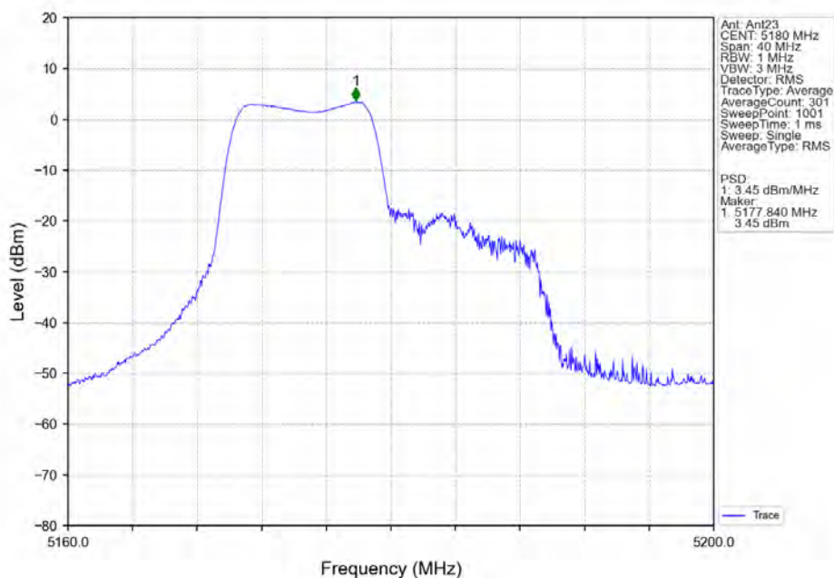
802.11ax(HEW20)_LCH_5180MHz_RU106_Left_Ant23_NTNV
