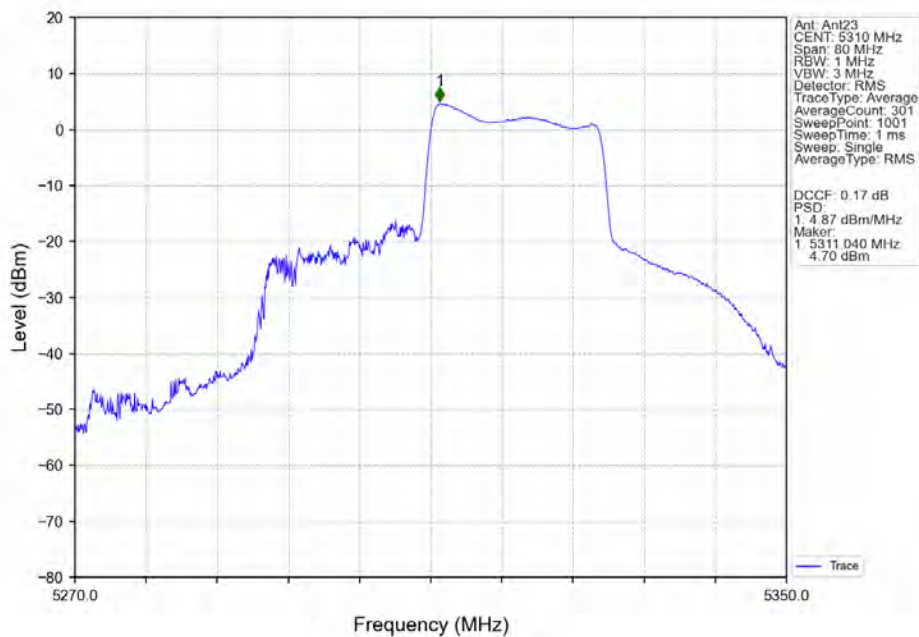
802.11ax(HEW40)_HCH_5310MHz_RU242_Right_Ant23_NTNV
