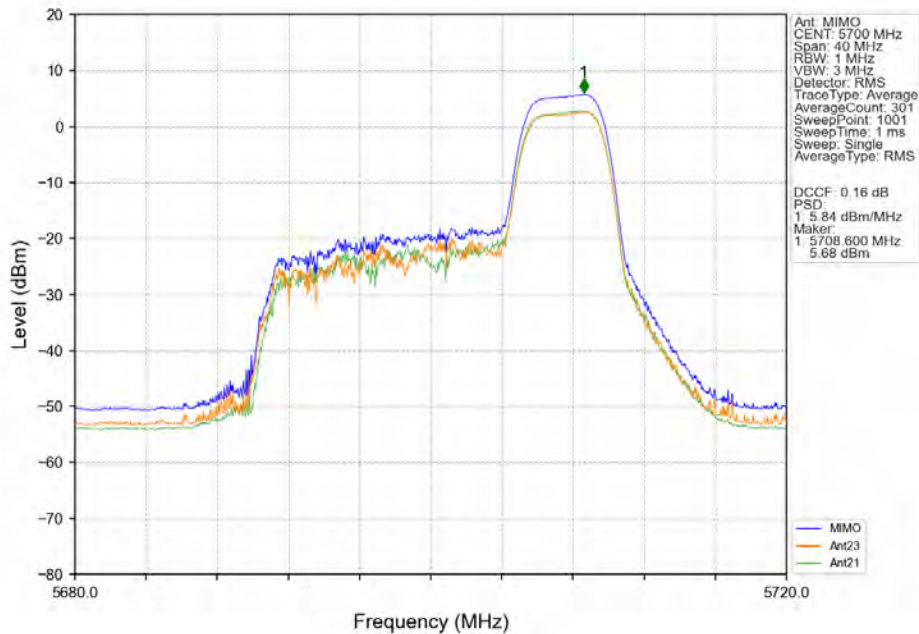
802.11ax(HEW20)_HCH_5700MHz_RU106_Right_Ant23_NTNV
