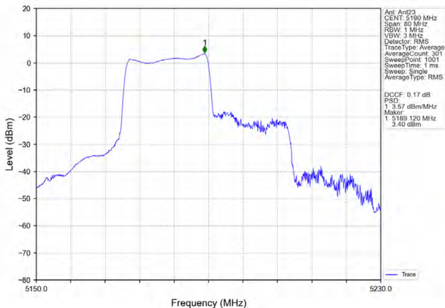
802.11ax(HEW40)_LCH_5190MHz_RU242_Left_Ant23_NTNV
