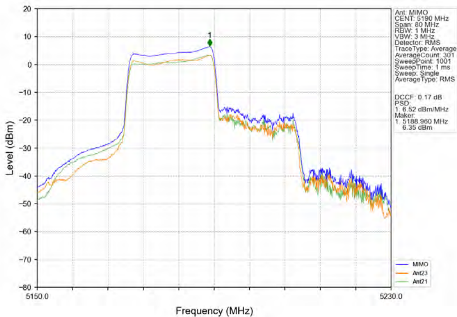
802.11ax(HEW40)_LCH_5190MHz_RU242_Left_MIMO_NTNV
