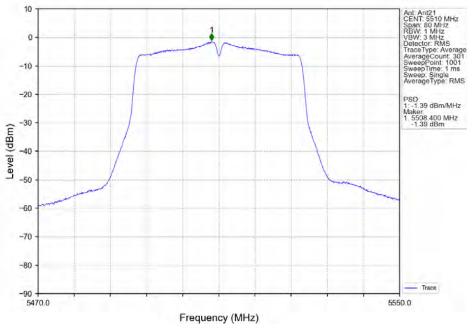
802.11ac(VHT40)_LCH_5510MHz_Ant21_NTNV
