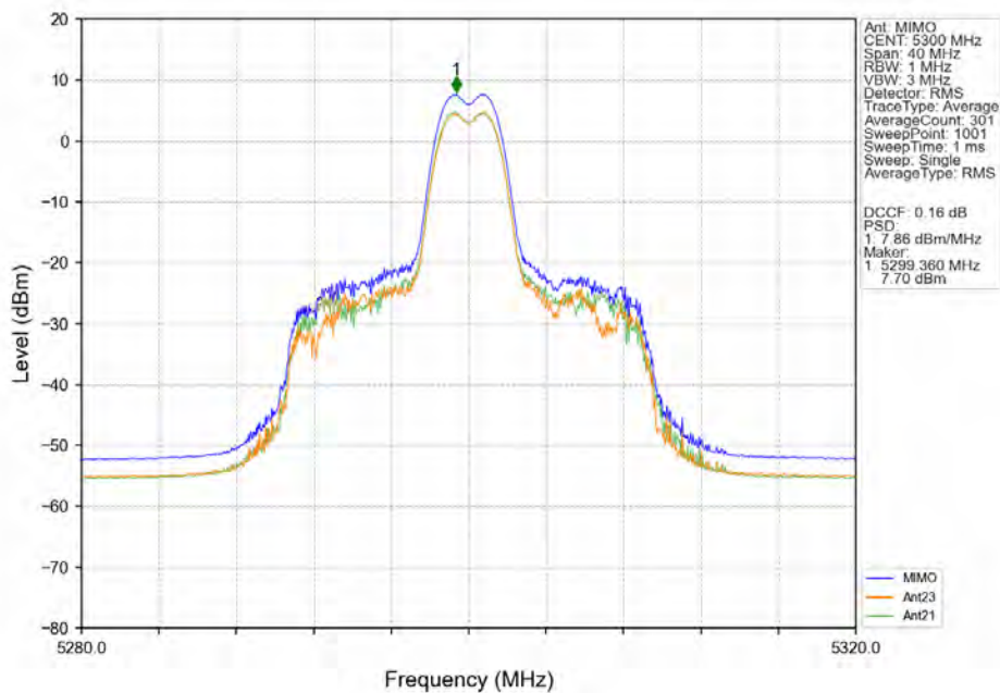
802.11ax(HEW20)_MCH_5300MHz_RU26_Mid_MIMO_NTNV
