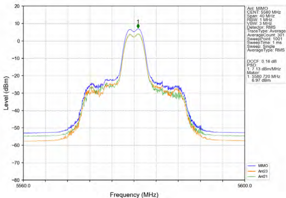
802.11ax(HEW20)_MCH_5580MHz_RU26_Mid_MIMO_NTNV
