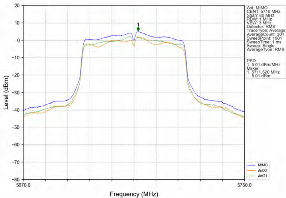
802.11n(HT40)_HCH_5710MHz_MIMO_NTNV
