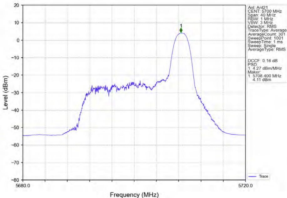
802.11ax(HEW20)_HCH_5700MHz_RU26_Right_MIMO_NTNV
