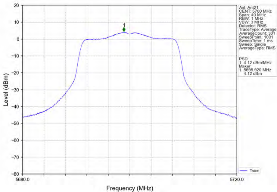
802.11ac(VHT20)_HCH_5700MHz_Ant21_NTNV
