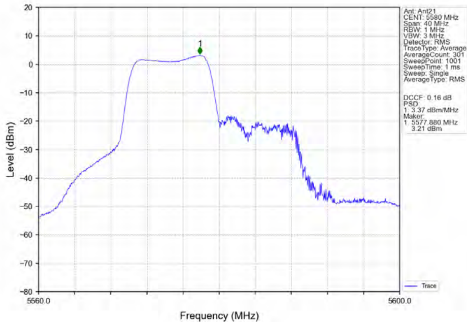
802.11ax(HEW20)_MCH_5580MHz_RU106_Left_MIMO_NTNV
