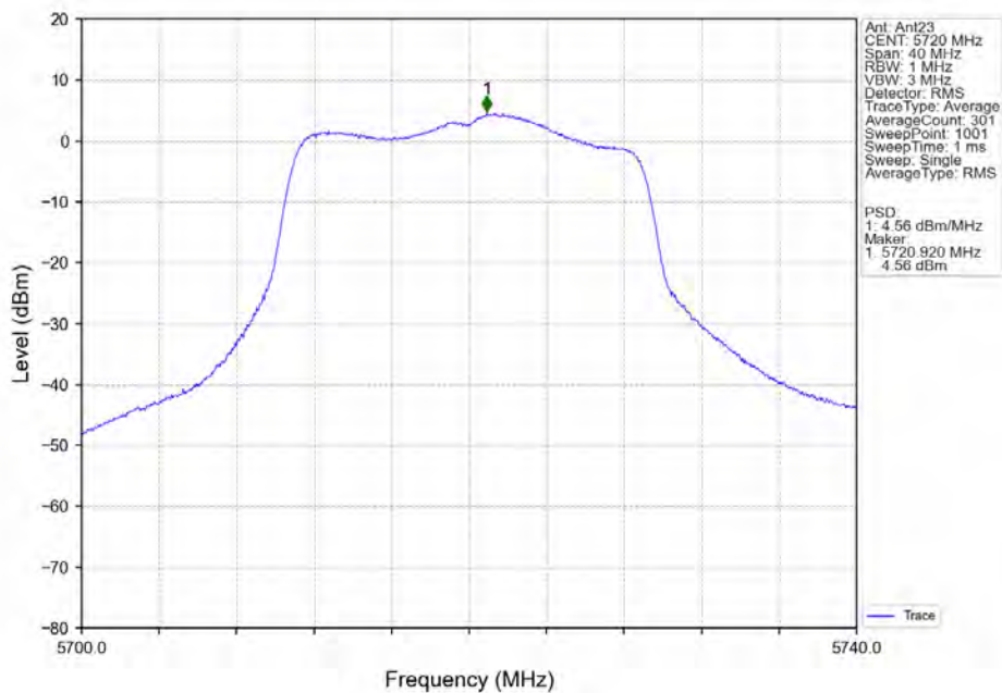
802.11ac(VHT20)_HCH_5720MHz_Ant23_NTNV
