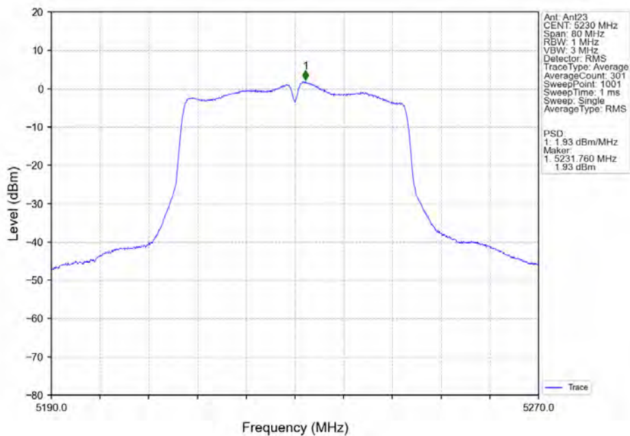
802.11ac(VHT40)_HCH_5230MHz_Ant23_NTNV
