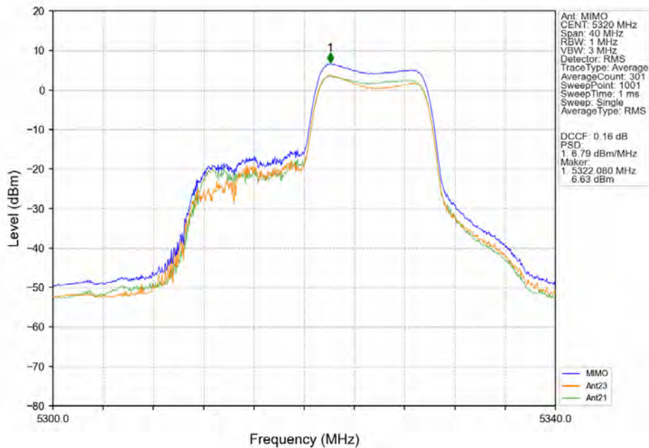
802.11ax(HEW20)_HCH_5320MHz_RU106_Right_MIMO_NTNV
