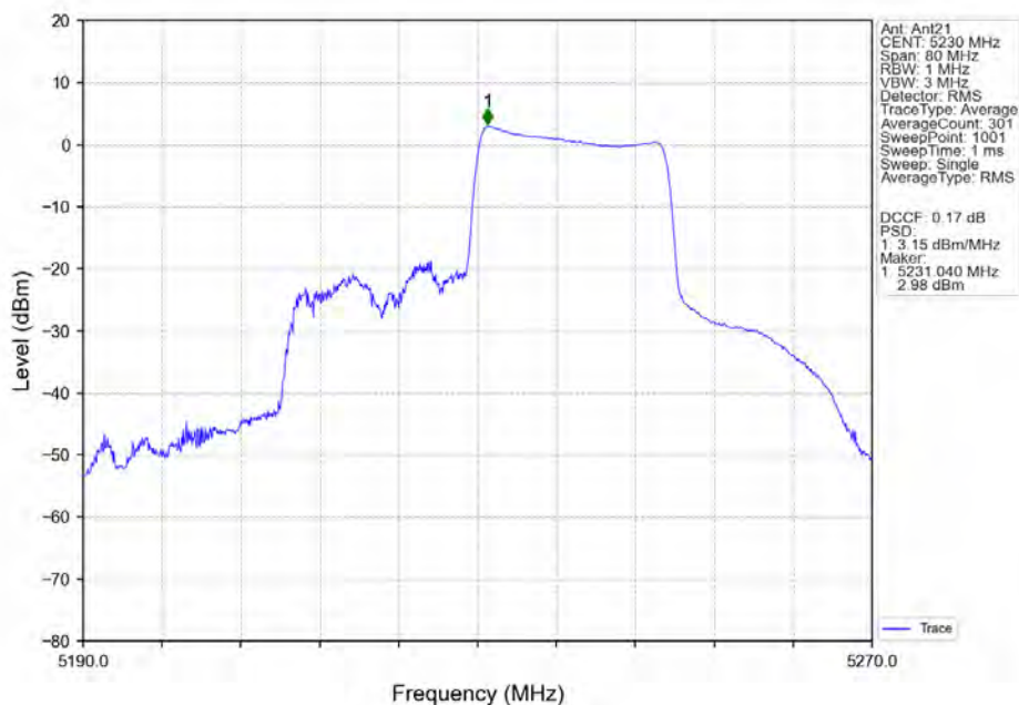
802.11ax(HEW40)_HCH_5230MHz_RU242_Right_MIMO_NTNV
