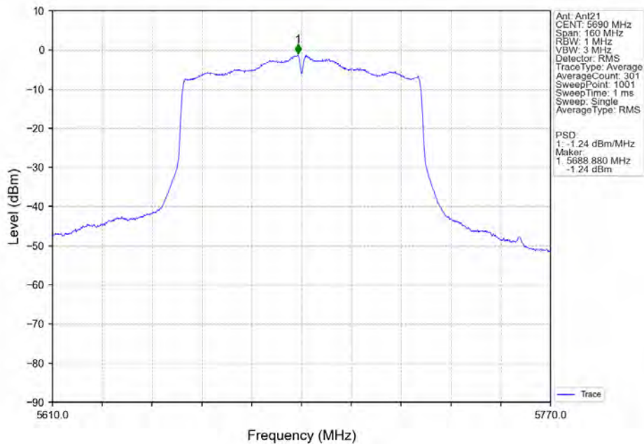
802.11ac(VHT80)_HCH_5690MHz_Ant21_NTNV
