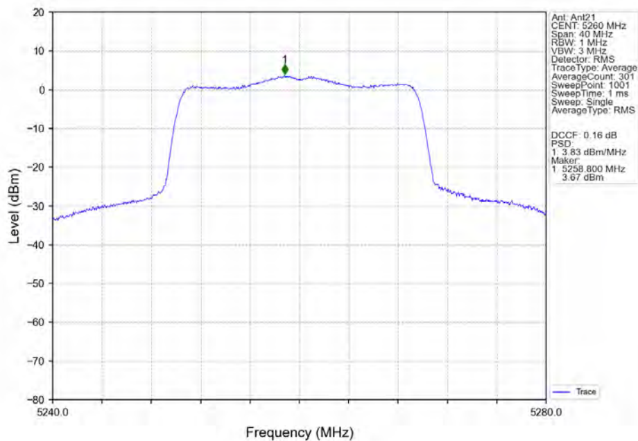
802.11ax(HEW20)_LCH_5260MHz_SU_/_Ant21_NTNV
