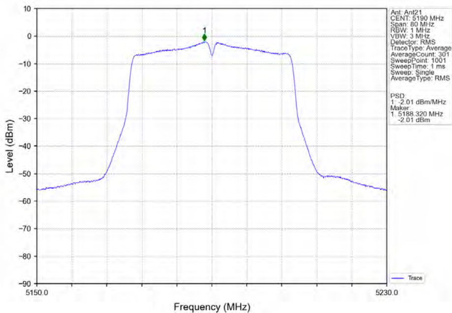
802.11ac(VHT40)_LCH_5190MHz_Ant21_NTNV
