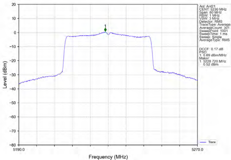
802.11ax(HEW40)_HCH_5230MHz_SU_/_Ant21_NTNV
