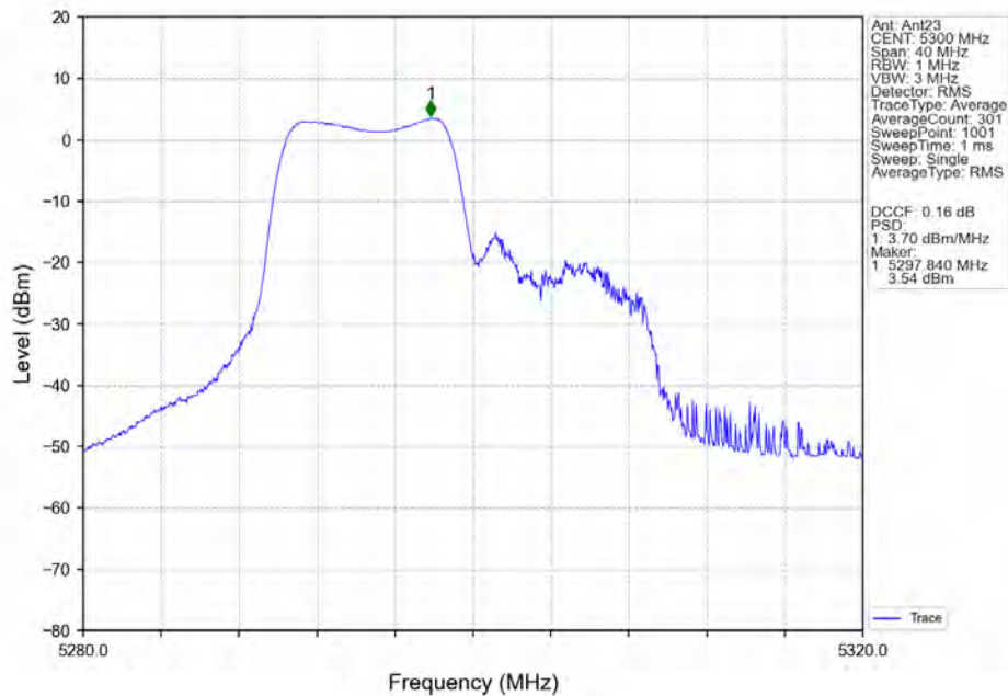
802.11ax(HEW20)_MCH_5300MHz_RU106_Left_Ant23_NTNV
