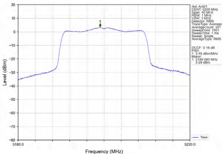
802.11ax(HEW20)_MCH_5200MHz_SU_/_Ant21_NTNV
