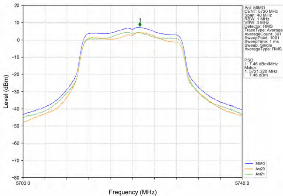
802.11ac(VHT20)_HCH_5720MHz_MIMO_NTNV
