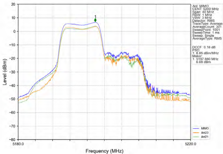
802.11ax(HEW20)_MCH_5200MHz_RU106_Left_MIMO_NTNV
