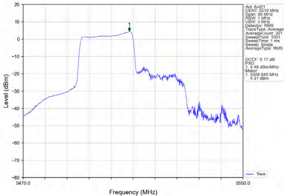
802.11ax(HEW40)_LCH_5510MHz_RU242_Left_MIMO_NTNV
