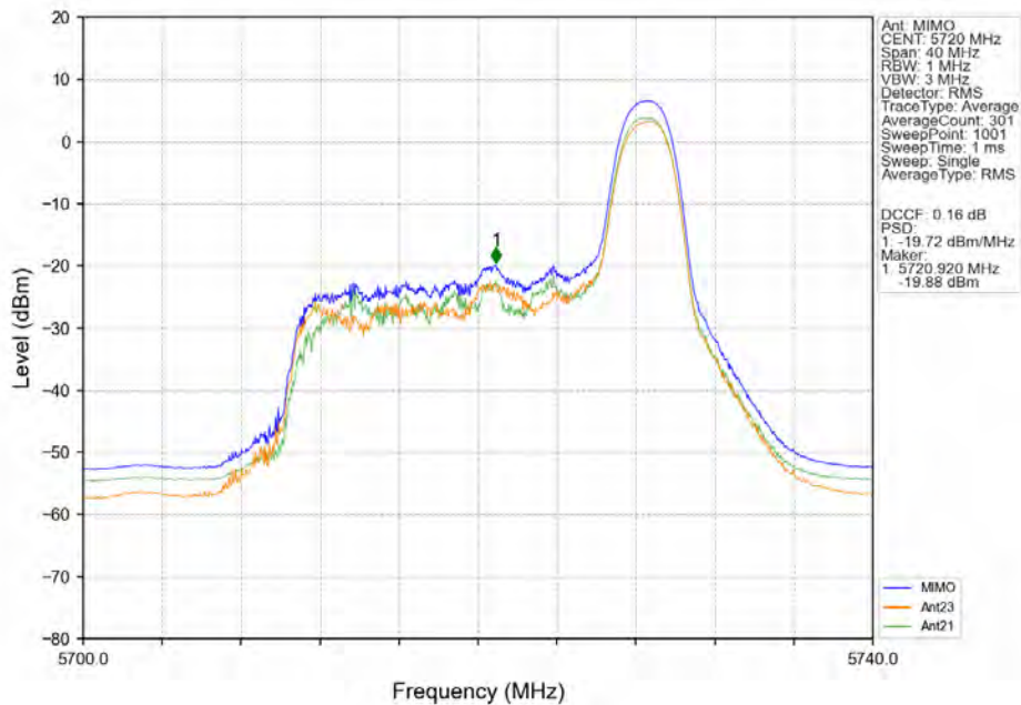
802.11ax(HEW20)_HCH_5720MHz_RU26_Right_MIMO_NTNV
