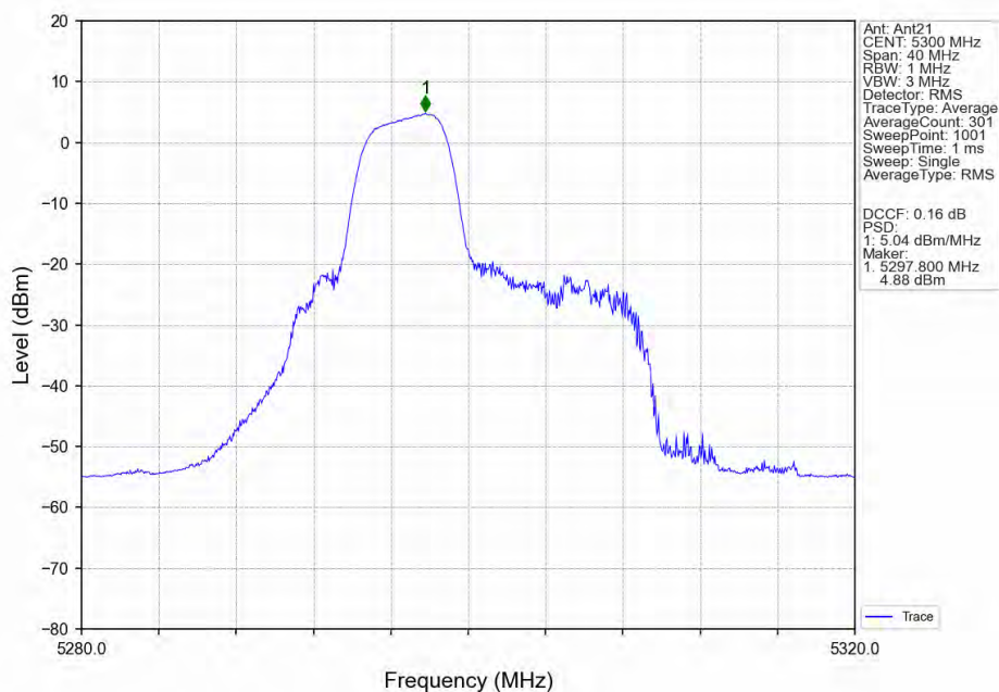
802.11ax(HEW20)_MCH_5300MHz_RU52_Mid_Ant21_NTNV
