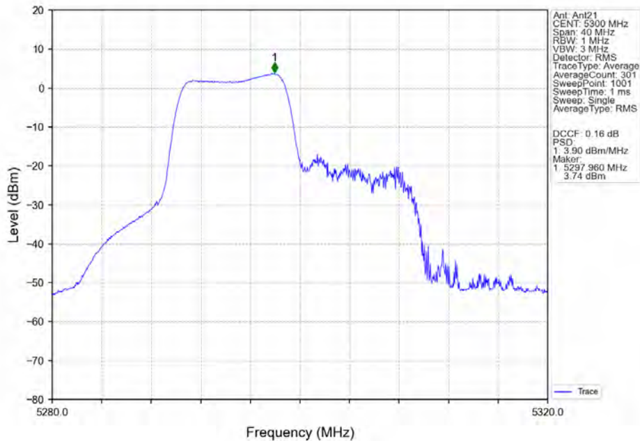
802.11ax(HEW20)_MCH_5300MHz_RU106_Left_MIMO_NTNV
