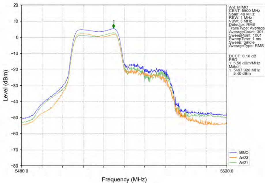
802.11ax(HEW20)_LCH_5500MHz_RU106_Left_MIMO_NTNV
