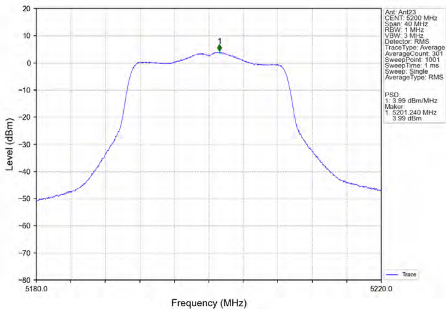
802.11ac(VHT20)_MCH_5200MHz_Ant23_NTNV
