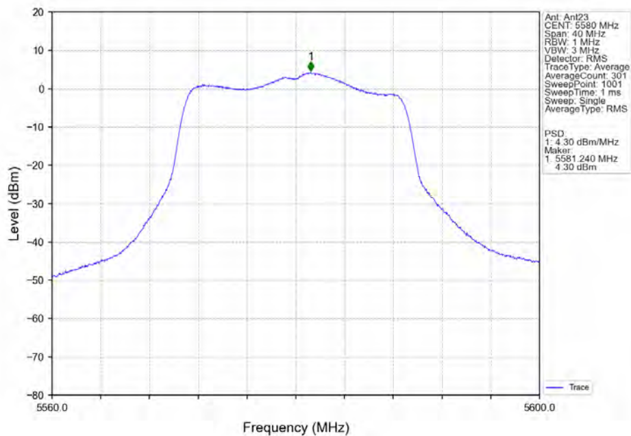
802.11ac(VHT20)_MCH_5580MHz_Ant23_NTNV
