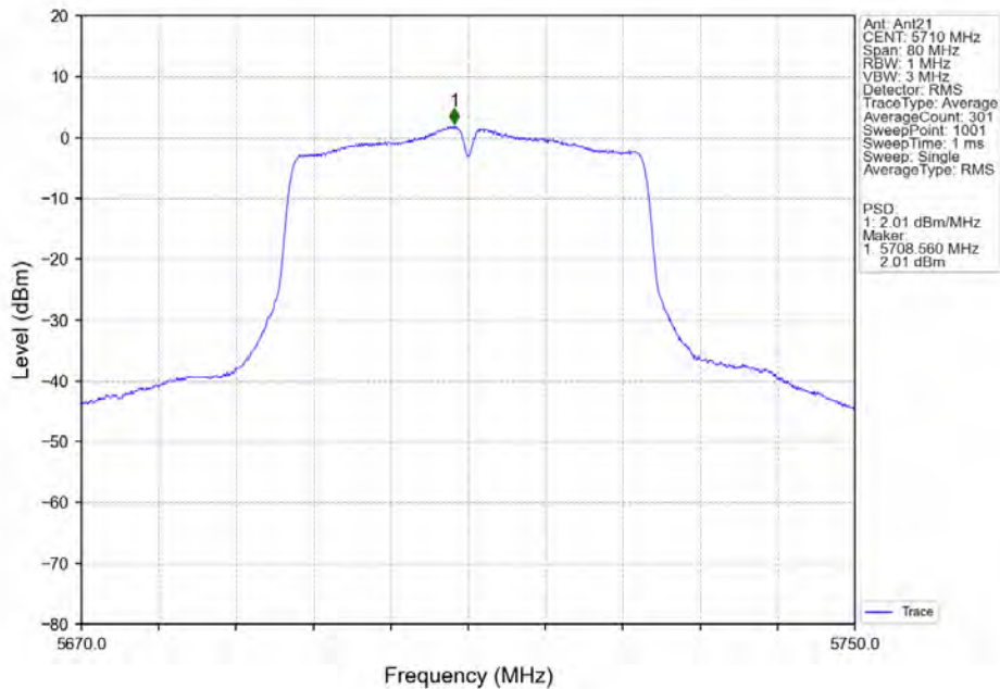
802.11ac(VHT40)_HCH_5710MHz_MIMO_NTNV
