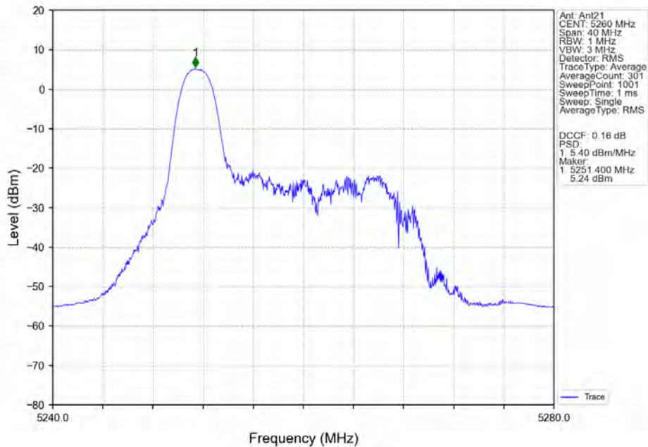
802.11ax(HEW20)_LCH_5260MHz_RU26_Left_MIMO_NTNV
