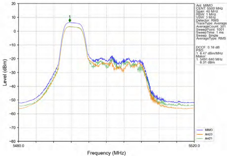
802.11ax(HEW20)_LCH_5500MHz_RU106_Left_Ant23_NTNV
