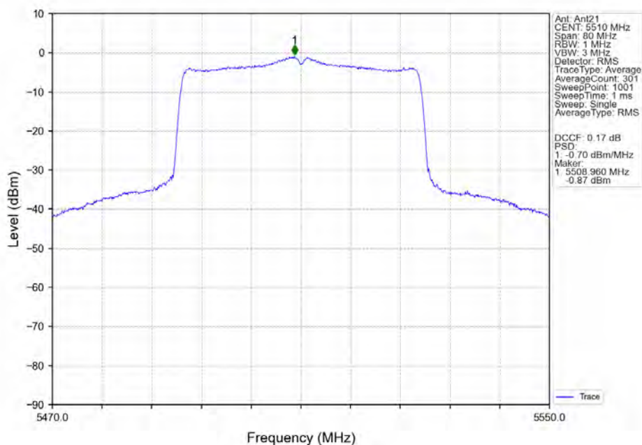
802.11ax(HEW40)_LCH_5510MHz_SU_/_Ant21_NTNV
