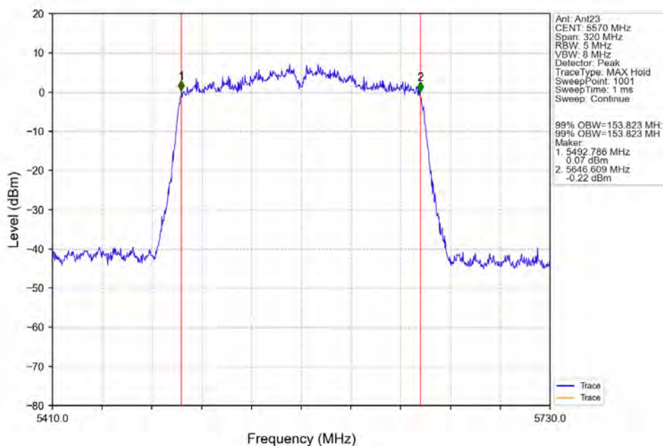
802.11ac(VHT160)_MCH_5570MHz_Ant23_NTNV
