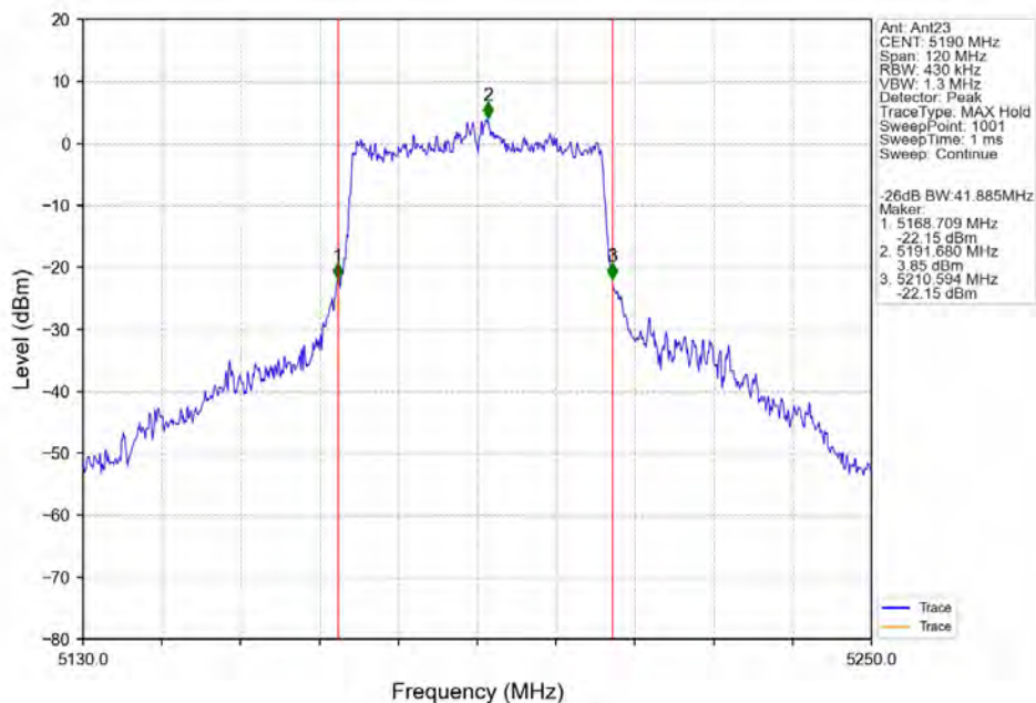
802.11ax(HEW40)_LCH_5190MHz_SU_/_Ant23_NTNV
