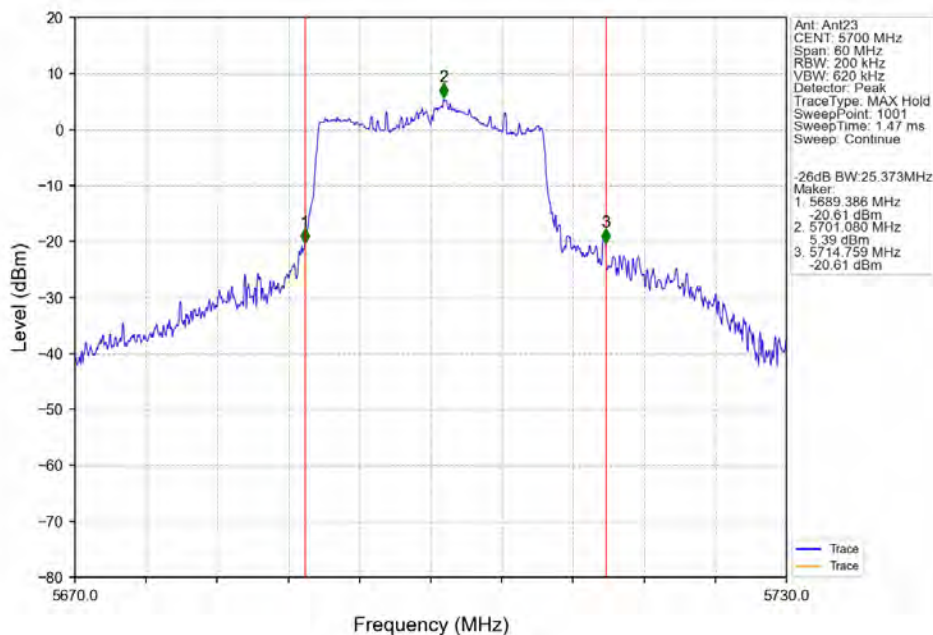
802.11ax(HEW20)_HCH_5700MHz_SU_/_Ant23_NTNV
