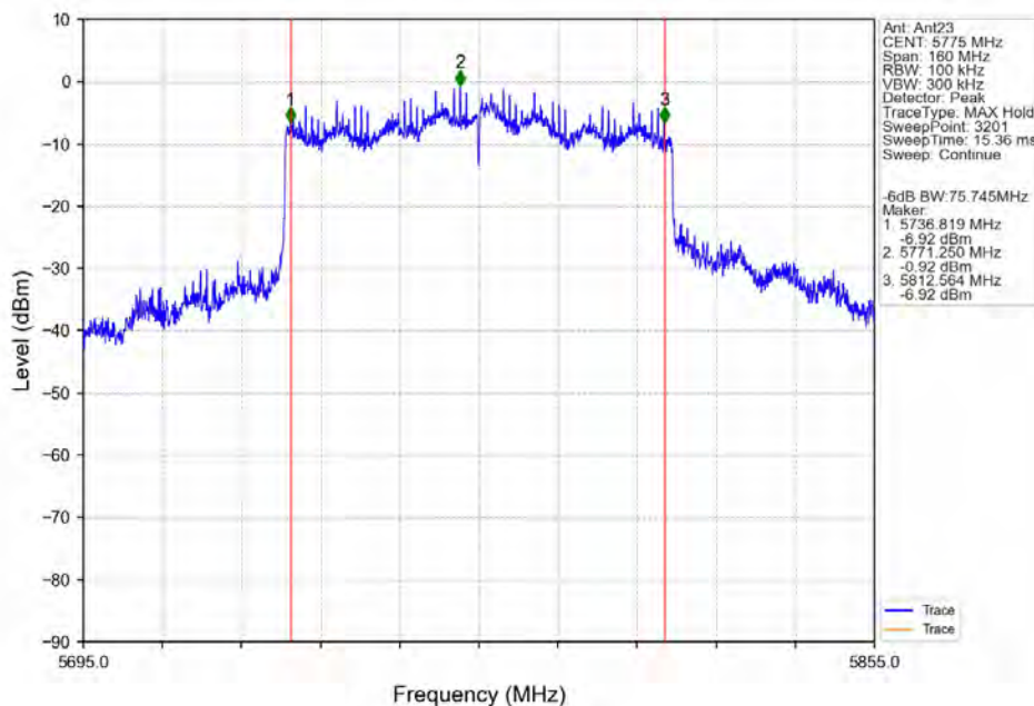
802.11ax(HEW80)_MCH_5775MHz_SU_/_Ant23_NTNV
