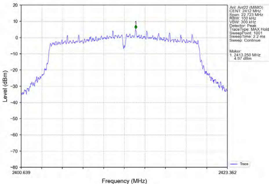
802.11g_LCH_2412MHz_Ant22 (MIMO)_NTNV
