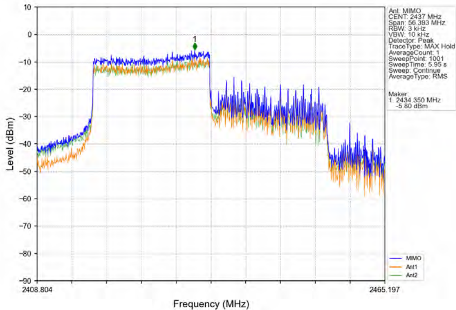
802.11ax(HEW40)_MCH_2437MHz_SU_/_Ant25 (MIMO)_NTNV
