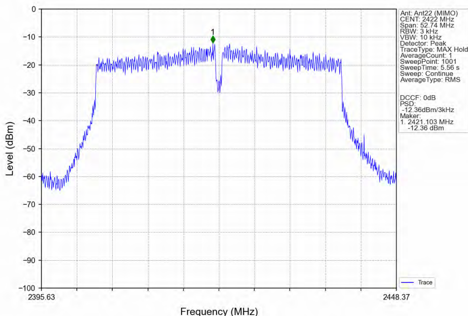
802.11ac(VHT40)_LCH_2422MHz_MIMO_NTNV
