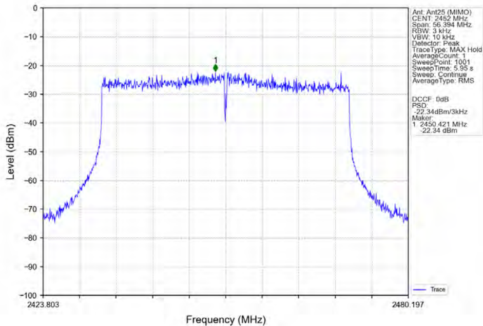
802.11ax(HEW40)_HCH_2452MHz_SU_/_Ant25 (MIMO)_NTNV
