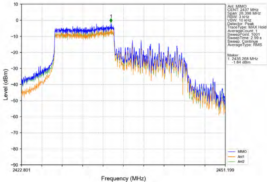
802.11ax(HEW20)_MCH_2437MHz_SU_/_Ant25 (MIMO)_NTNV
