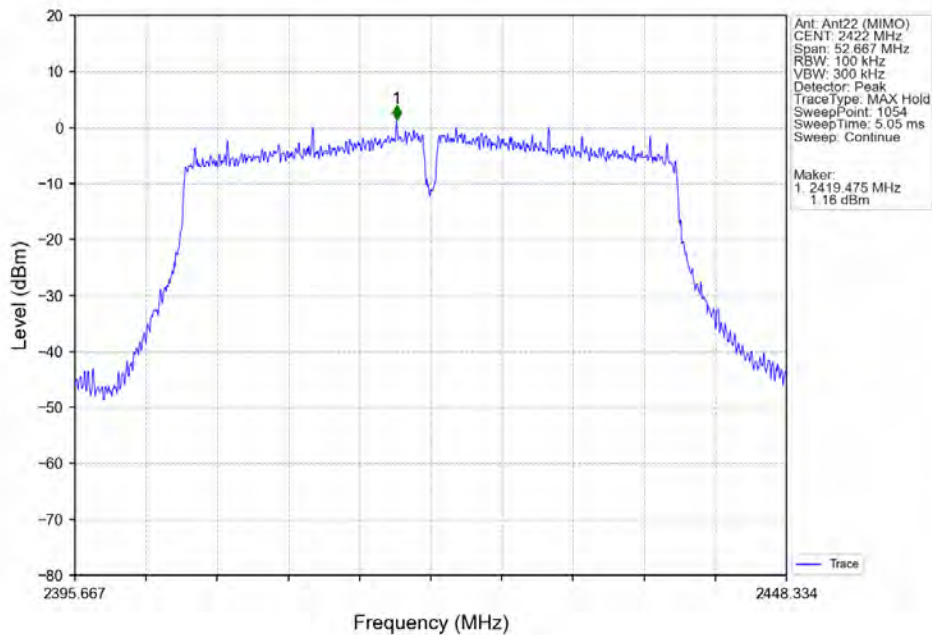
802.11n(HT40)_LCH_2422MHz_Ant22 (MIMO)_NTNV
