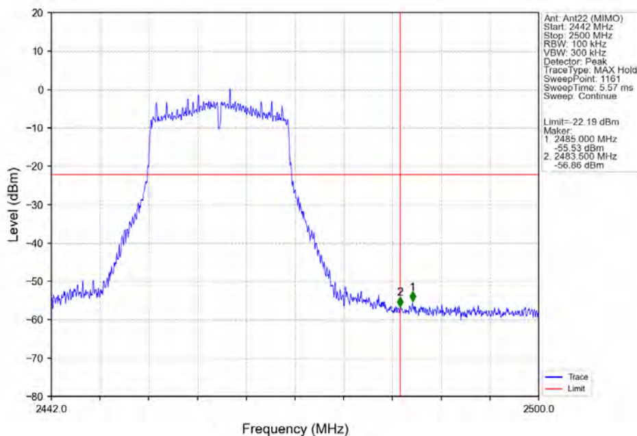
802.11g_HCH_2462MHz_Ant22 (MIMO)_NTNV
