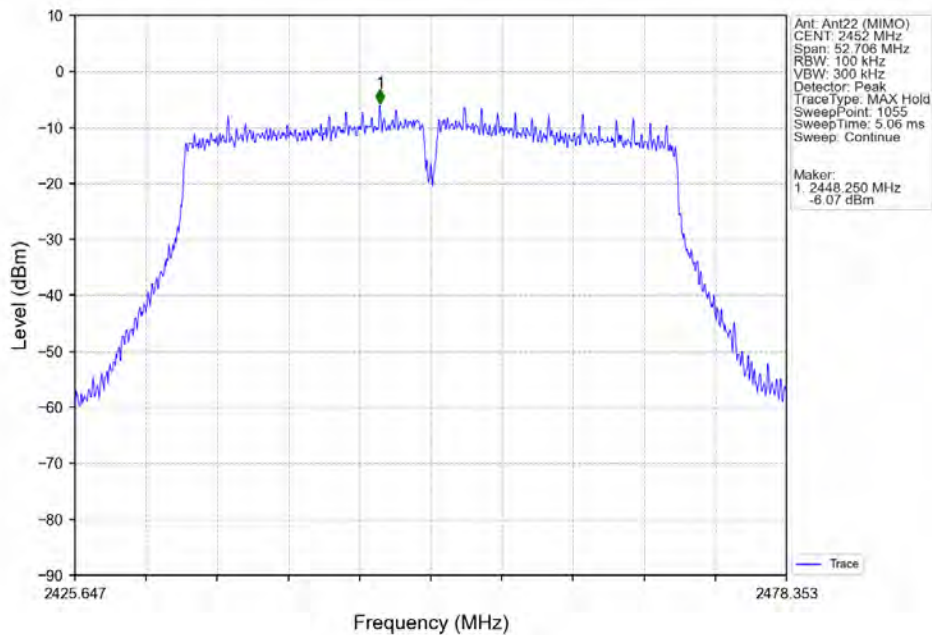
802.11ac(VHT40)_HCH_2452MHz_Ant22 (MIMO)_NTNV
