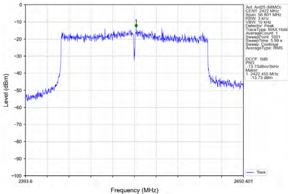
802.11ax(HEW40)_LCH_2422MHz_SU_/_Ant25 (MIMO)_NTNV
