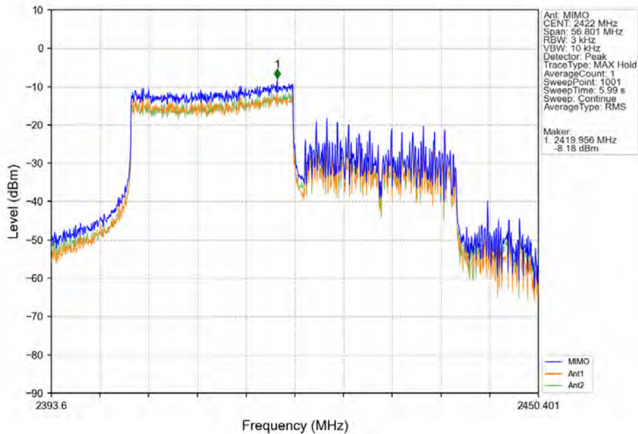
802.11ax(HEW40)_LCH_2422MHz_SU_/_Ant25 (MIMO)_NTNV
