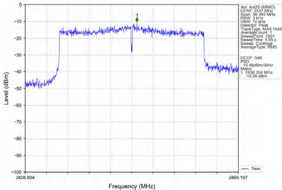
802.11ax(HEW40)_MCH_2437MHz_SU_/_Ant25 (MIMO)_NTNV
