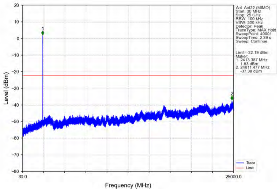
802.11g_LCH_2412MHz_Ant22 (MIMO)_NTNV
