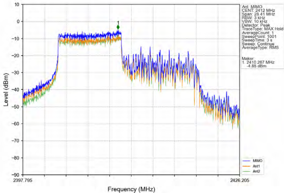
802.11ax(HEW20)_LCH_2412MHz_SU_/_Ant25 (MIMO)_NTNV
