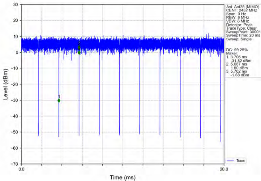
802.11ac(VHT40)_HCH_2452MHz_Ant25 (MIMO)_NTNV
