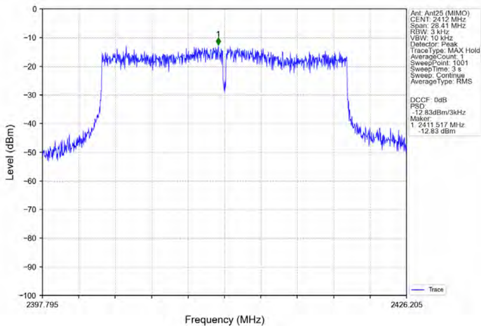
802.11ax(HEW20)_LCH_2412MHz_SU_/_Ant25 (MIMO)_NTNV
