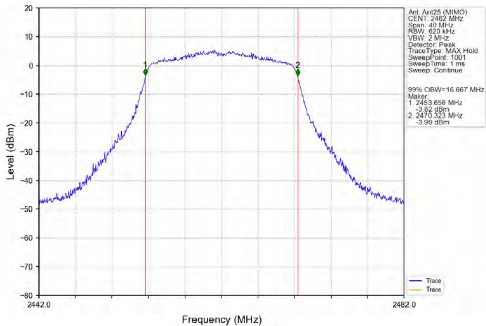
802.11g_HCH_2462MHz_Ant25 (MIMO)_NTNV
