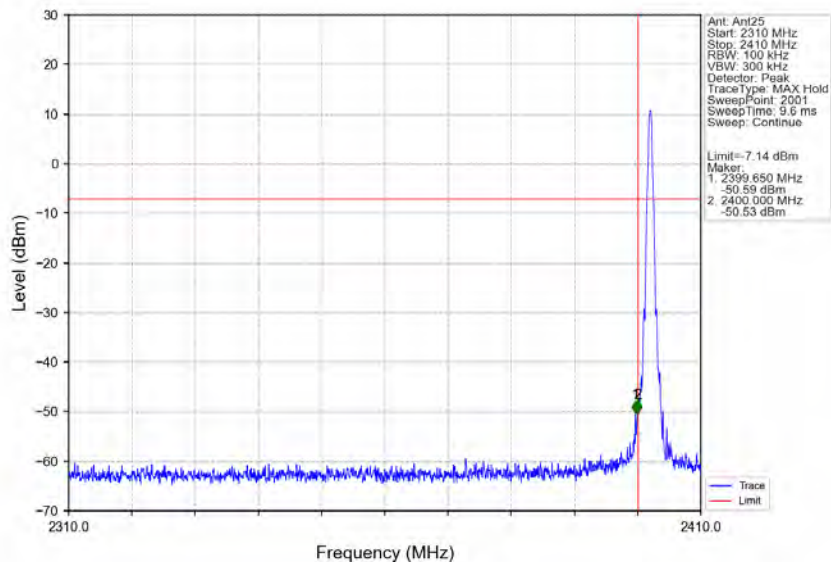
GFSK_DH5_LCH_2402MHz_Ant25_NTNV
