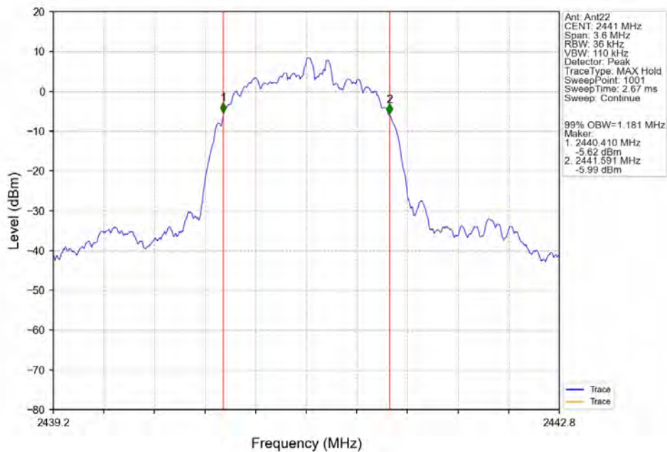
8DPSK_3DH5_MCH_2441MHz_Ant22_NTNV
