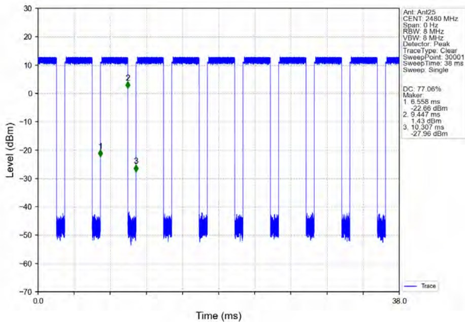
Pi/4DQPSK_2DH5_HCH_2480MHz_Ant25_NTNV
