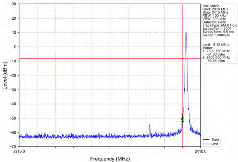
GFSK_DH5_LCH_2402MHz_Ant22_NTNV
