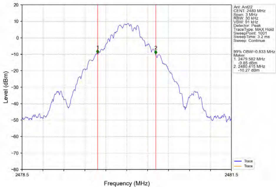
GFSK_DH5_HCH_2480MHz_Ant22_NTNV
