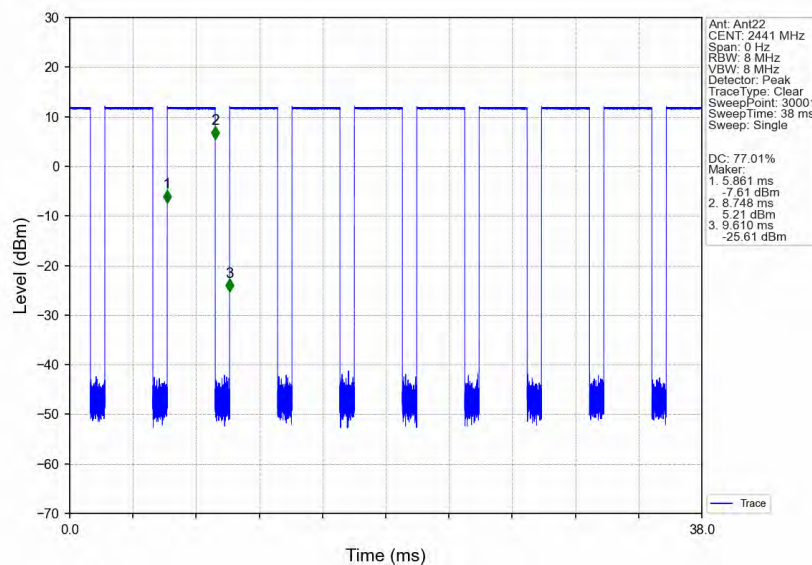
GFSK_DH5_MCH_2441MHz_Ant22_NTNV
