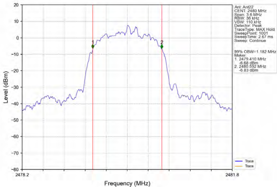
8DPSK_3DH5_HCH_2480MHz_Ant22_NTNV
