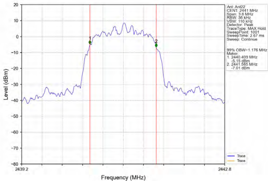
Pi/4DQPSK_2DH5_MCH_2441MHz_Ant22_NTNV
