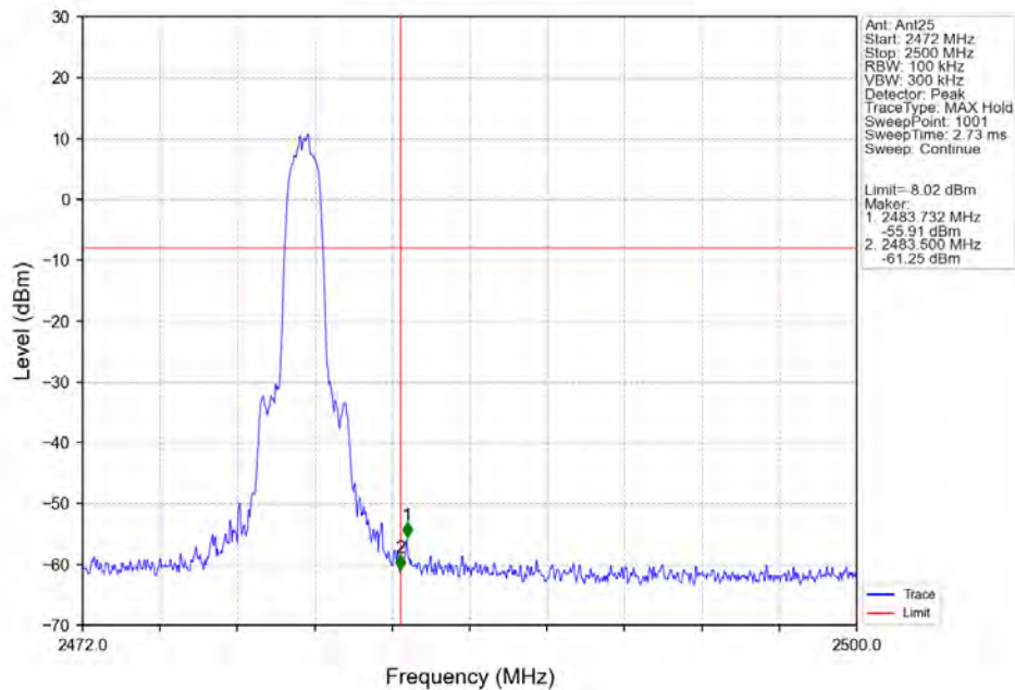
Pi/4DQPSK_2DH5_HCH_2480MHz_Ant25_NTNV
