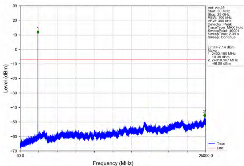
GFSK_DH5_LCH_2402MHz_Ant25_NTNV
