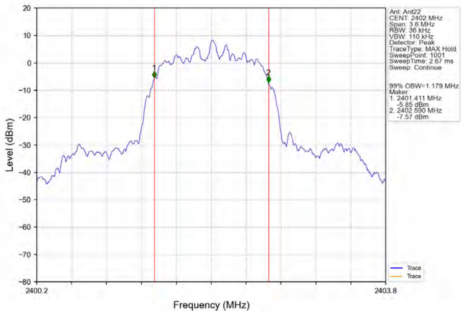
Pi/4DQPSK_2DH5_LCH_2402MHz_Ant22_NTNV
