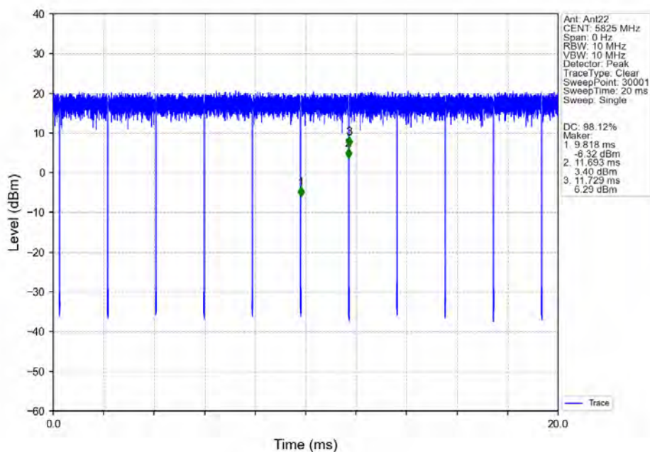
802.11n(HT20)_HCH_5825MHz_Ant22_NTNV
