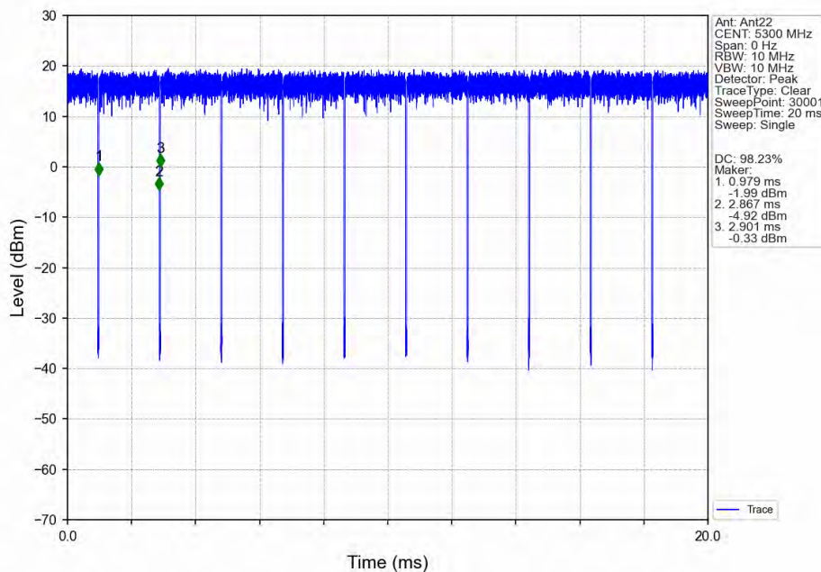
802.11ac(VHT20)_MCH_5300MHz_Ant22_NTNV
