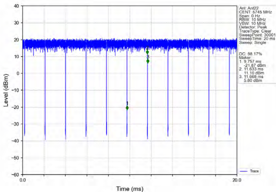
802.11n(HT20)_LCH_5745MHz_Ant22_NTNV
