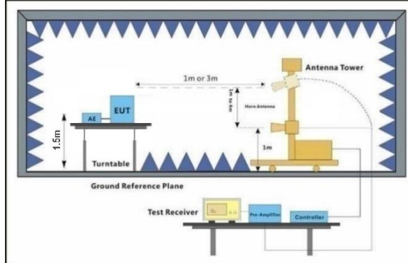
Figure 3. above 1GHz
