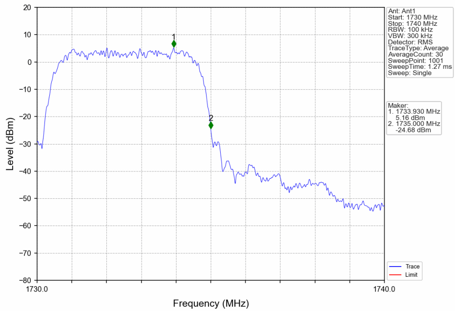
Band IV_RMC_MCH_1732.6MHz_12.2kbps RMC_NTNV
