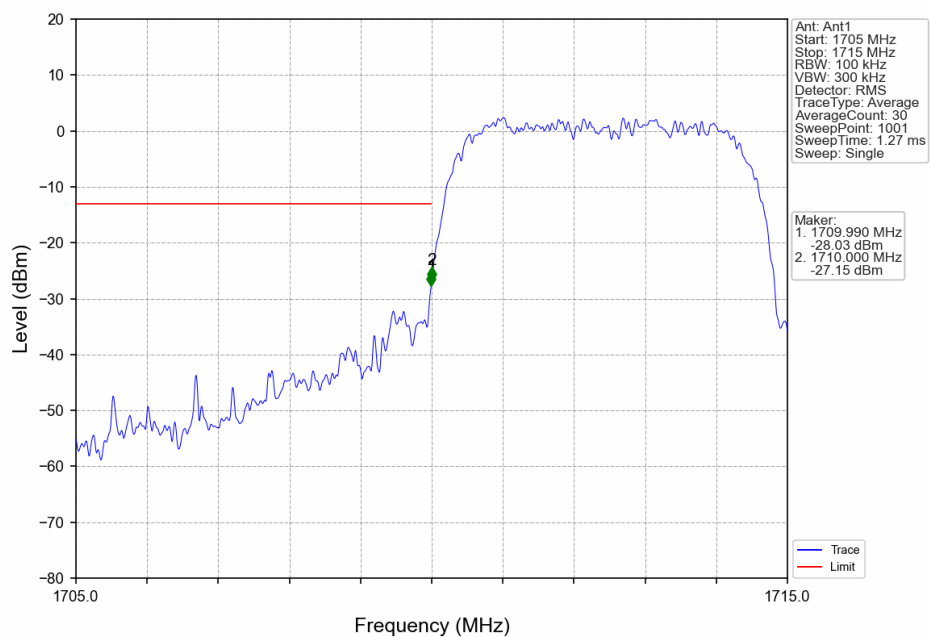
Band IV_HSDPA_LCH_1712.4MHz_Subtest 1_NTNV
