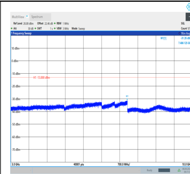
Band13_10MHz_QPSK_23230_1RB#0_3000~10000_3000~10000
