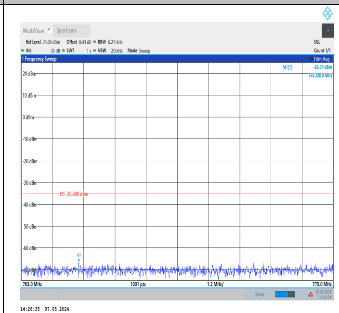
Band13_5MHz_QPSK_23255_1RB#0_763~775_763~775
