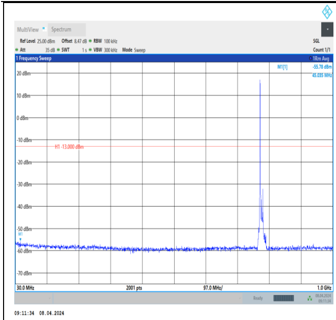
Band13_10MHz_QPSK_23230_1RB#0_30~1000_30~1000
