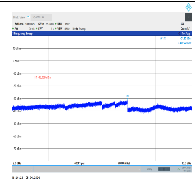
Band13_5MHz_QPSK_23230_1RB#0_3000~10000_3000~10000
