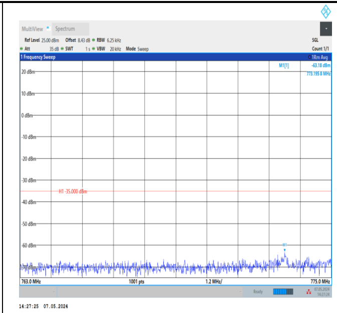
Band13_10MHz_QPSK_23230_1RB#0_763~775_763~775
