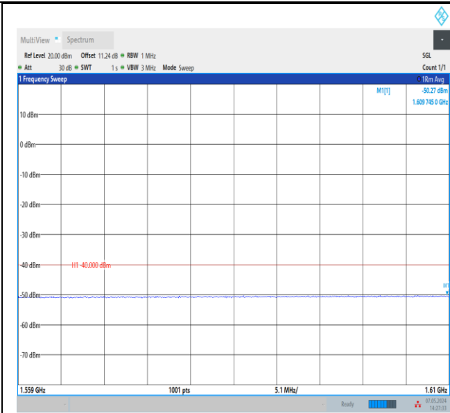
Band13_10MHz_QPSK_23230_1RB#0_1559~1610_1559~1610
