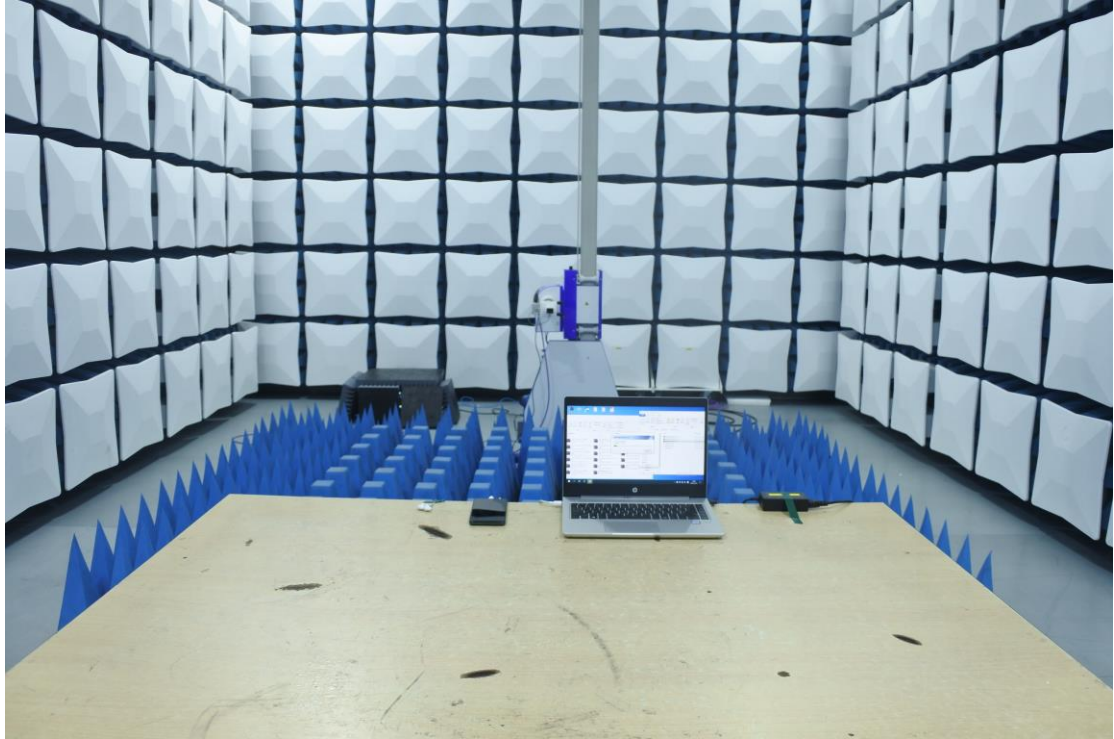
FCC Part15B Radiated Emission 18GHz-26.5GHz -Front
