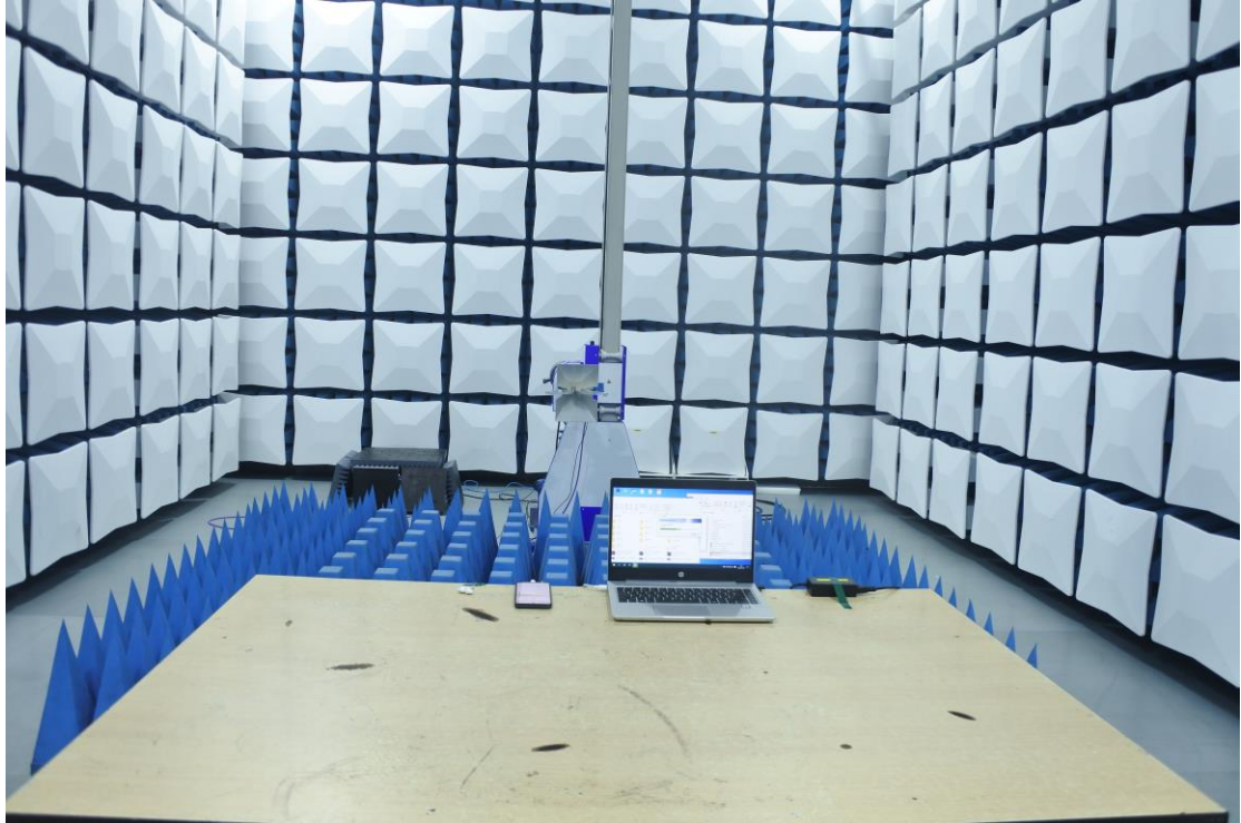
FCC Part15B Radiated Emission 1GHz-18GHz -Front
