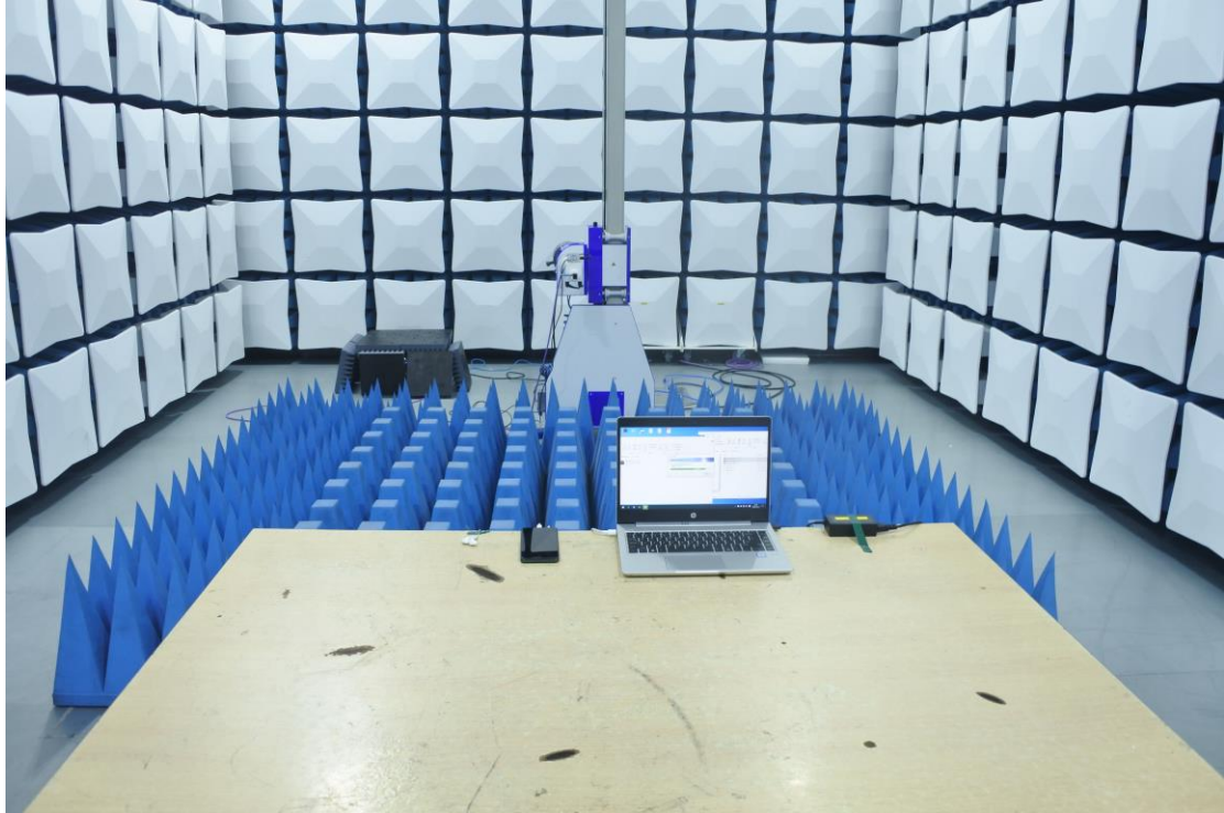
FCC Part15B Radiated Emission 26.5GHz-40GHz -Front
