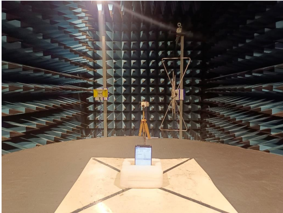
Radiated Emission Above 18 GHz -26.5 GHz -Front
