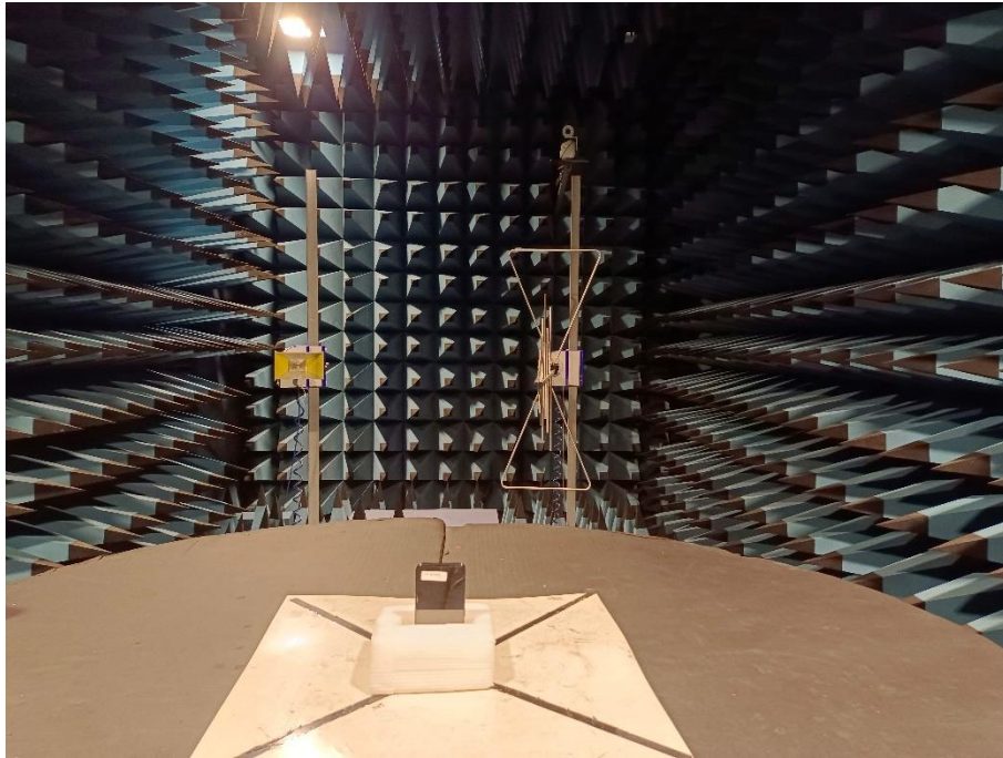
Radiated Emission 1 GHz-18 GHz -Front
