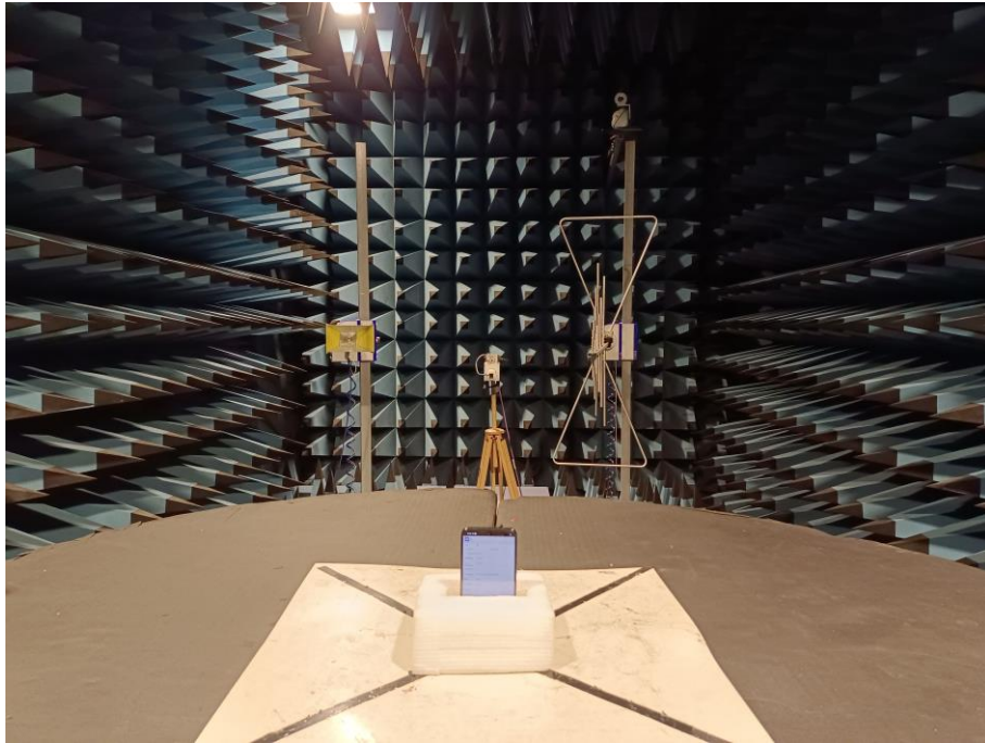
Radiated Emission Above 26.5 GHz -40 GHz -Front
