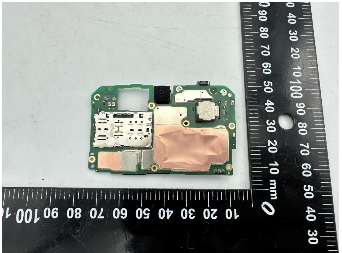
Photo 11 Inside of EUT
