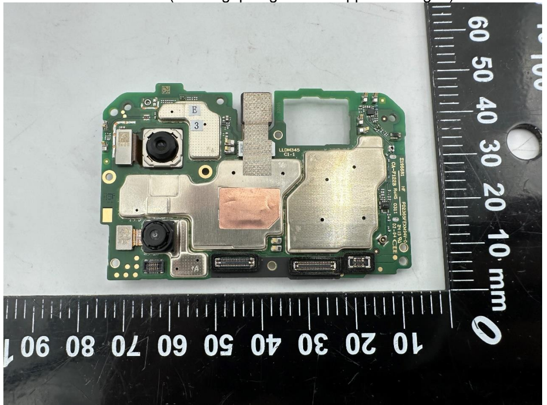
Photo 10 Inside of EUT (Shield gap largen and copper foil largen)
