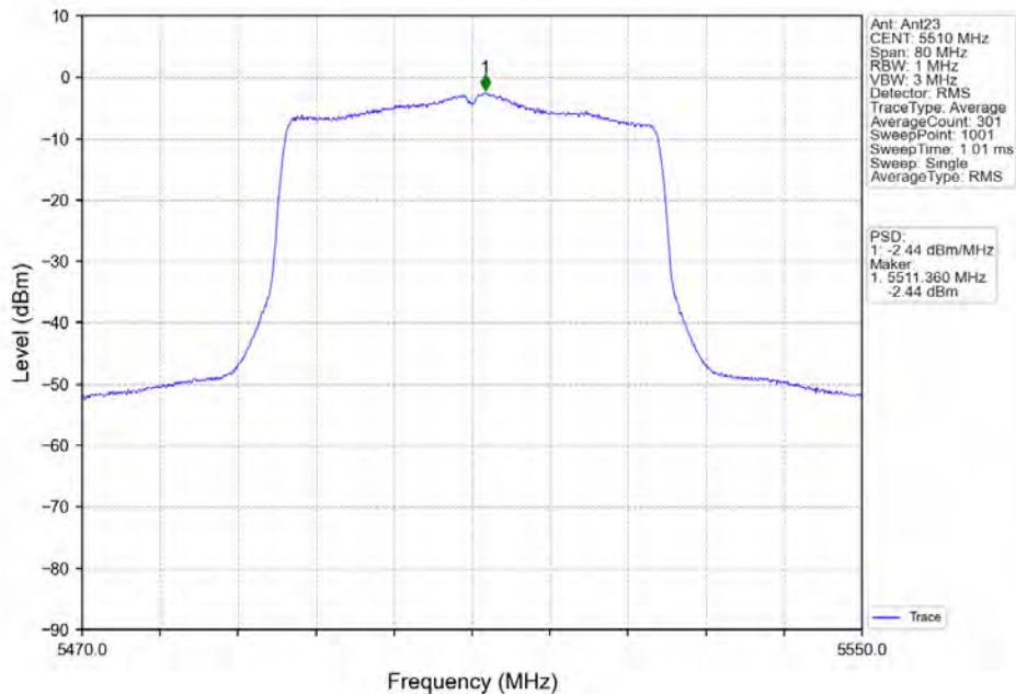
802.11ax(HE40) LCH_5510MHz RU484 Left MIMO_NTNV
