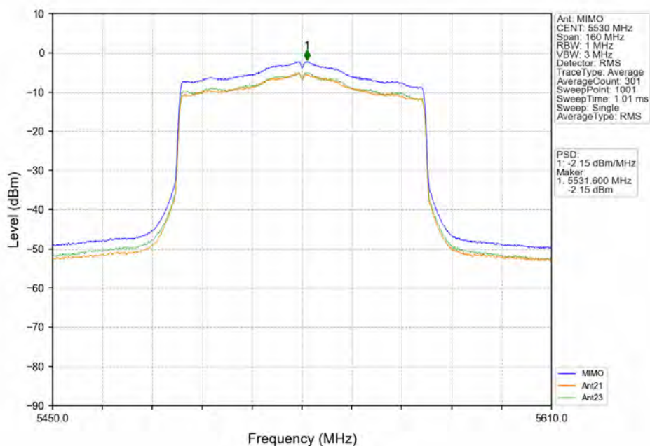
802.11ax(HE80) LCH_5530MHz RU996 Left MIMO_NTNV
