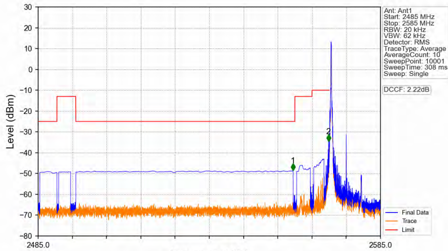
Band38_10MHz_64QAM_LCH_2575MHz_RB_1_0_NTNV
