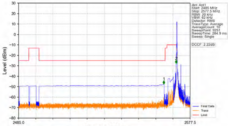
Band38_5MHz_64QAM_LCH_2572.5MHz_RB_1_0_NTNV
