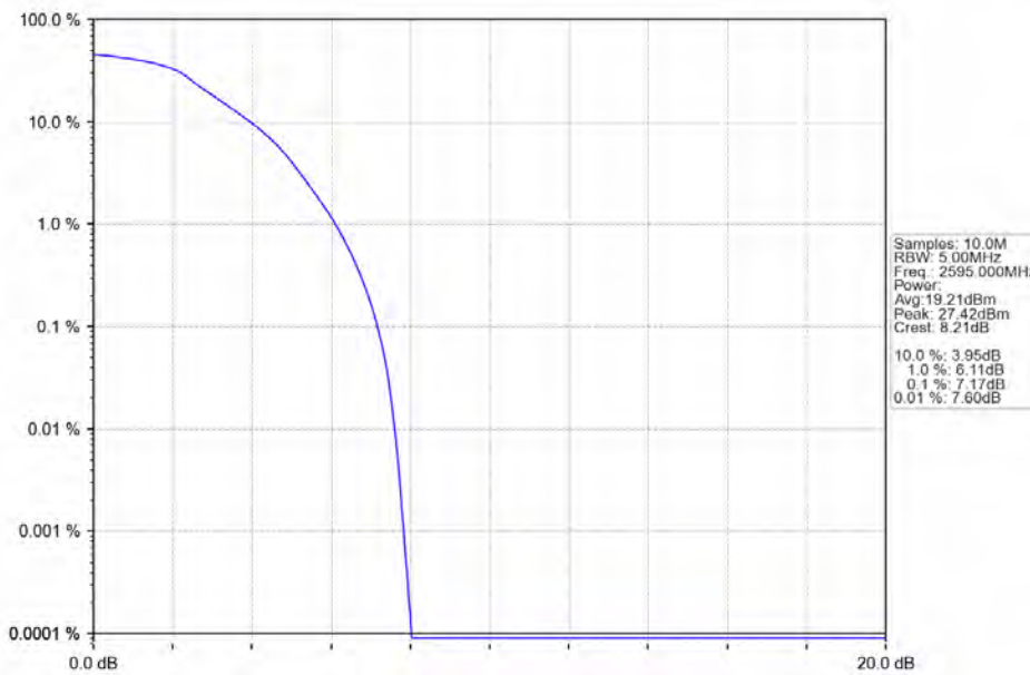
Band38_5MHz_QPSK_MCH_2595MHz_RB_25_0_NTV
