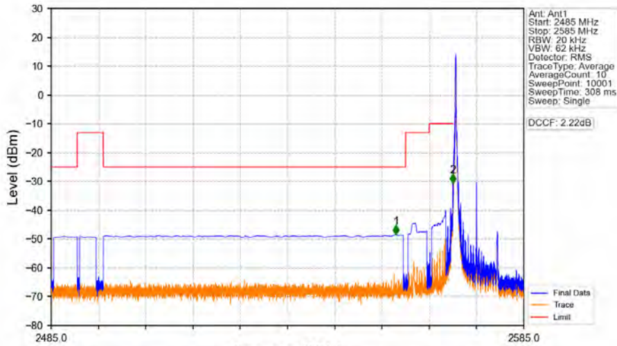
Band38_10MHz_16QAM_LCH_2575MHz_RB_1_0_NTNV
