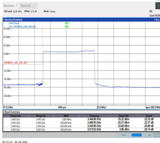
1-N78-3450-3550-PC2-30-70-L-3-DFT-PI2BPSK-Outer_Full-180@0-Ant12-1--PASS-see graph
