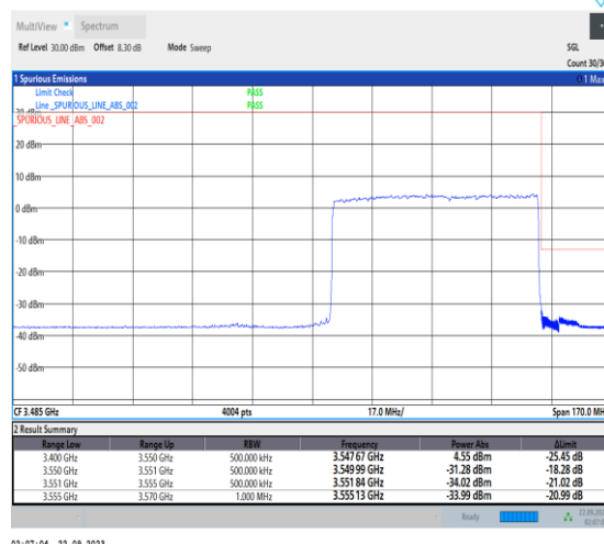
1-N78-3450-3550-PC2-30-60-H-3-DFT-PI2BPSK-Outer_Full-162@0-Ant12-1--PASS-see graph
