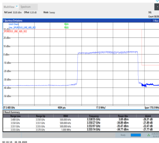
1-N78-3450-3550-PC2-30-70-H-3-DFT-PI2BPSK-Outer_Full-180@0-Ant12-1--PASS-see graph
