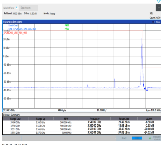
1-N78-3450-3550-PC2-30-60-H-5-CP-QPSK-Edge_1RB_Right-1@161-Ant12-1--PASS-see graph
