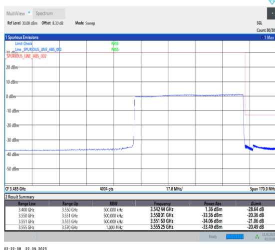
1-N78-3450-3550-PC2-30-70-H-6-CP-QPSK-Outer_Full-189@0-Ant12-1--PASS-see graph
