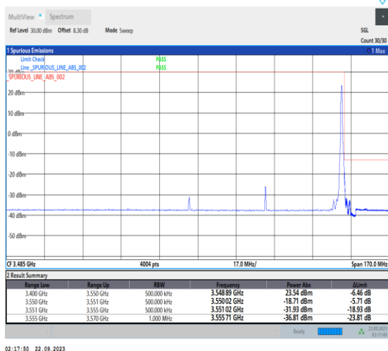
1-N78-3450-3550-PC2-30-70-H-2-DFT-PI2BPSK-Edge_1RB_Right-1@188-Ant12-1--PASS-see graph
