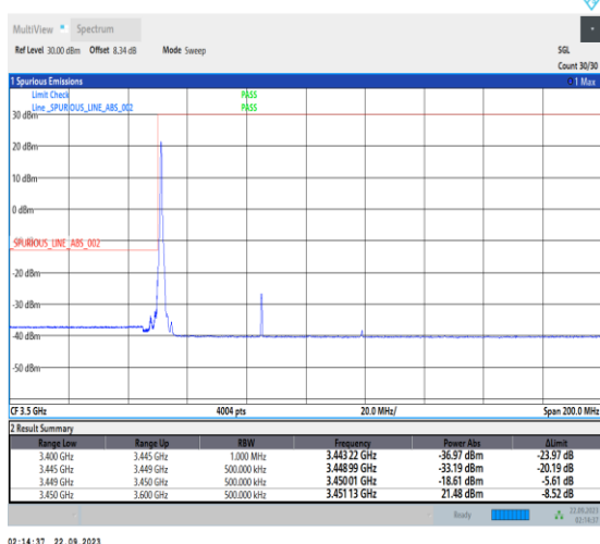
1-N78-3450-3550-PC2-30-70-L-4-CP-QPSK-Edge_1RB_Left-1@0-Ant12-1--PASS-see graph
