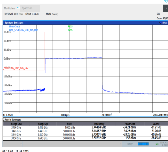
1-N78-3450-3550-PC2-30-70-L-6-CP-QPSK-Outer_Full-189@0-Ant12-1--PASS-see graph
