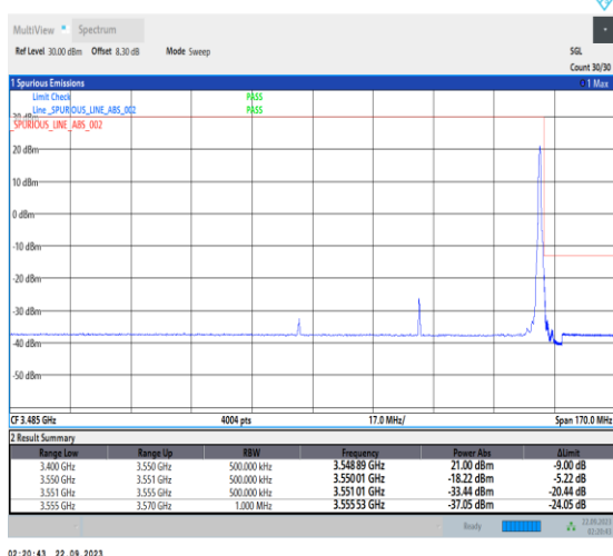
1-N78-3450-3550-PC2-30-70-H-5-CP-QPSK-Edge_1RB_Right-1@188-Ant12-1--PASS-see graph
