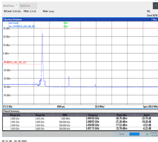
1-N78-3450-3550-PC2-30-70-L-1-DFT-PI2BPSK-Edge_1RB_Left-1@0-Ant12-1--PASS-see graph
