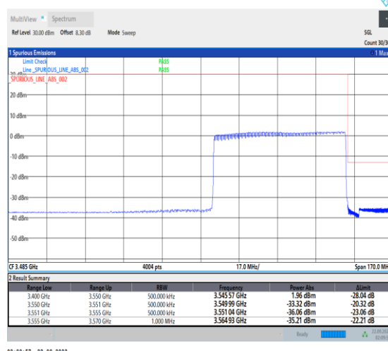
1-N78-3450-3550-PC2-30-60-H-6-CP-QPSK-Outer_Full-162@0-Ant12-1--PASS-see graph
