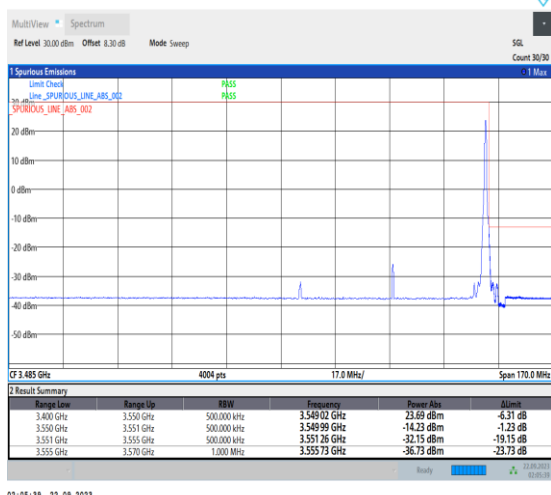
1-N78-3450-3550-PC2-30-60-H-2-DFT-PI2BPSK-Edge_1RB_Right-1@161-Ant12-1--PASS-see graph
