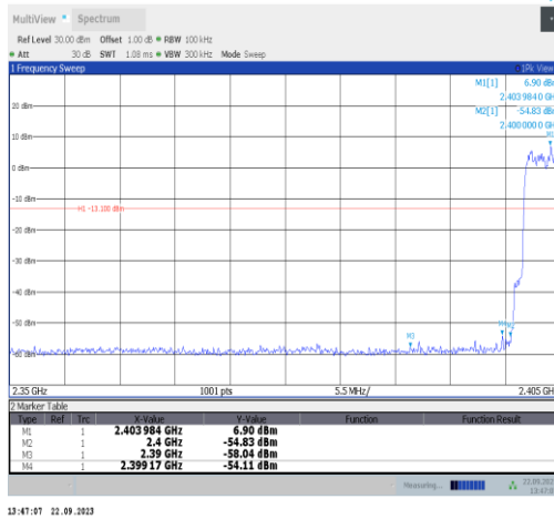
3DH5-Ant22-Hop_2402-PASS
