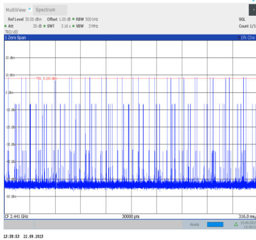
2DH1-Ant22-Hop-PASS
