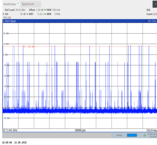
3DH3-Ant22-Hop-PASS
