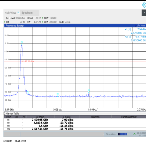
2DH5-Ant22-2480-PASS
