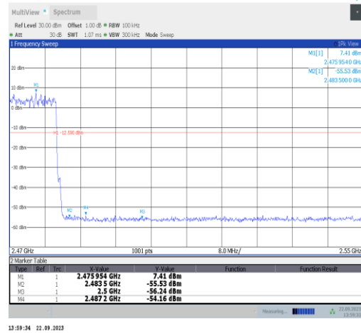
3DH5-Ant22-Hop_2480-PASS
