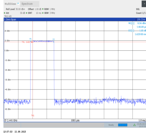
3DH3-Ant22-Hop-PASS
