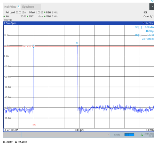
DH5-Ant22-Hop-PASS
