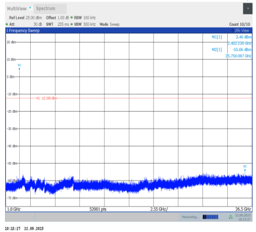
2DH5-Ant22-2402-1000~26500-PASS
