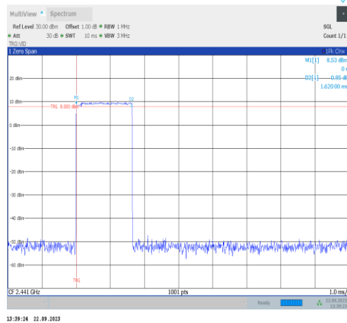
2DH3-Ant22-Hop-PASS
