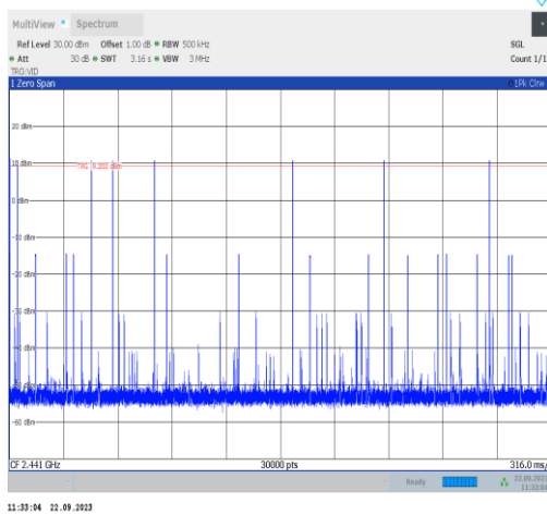
DH5-Ant22-Hop-PASS
