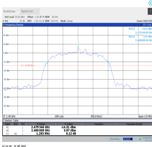
3DH5-Ant22-2480
