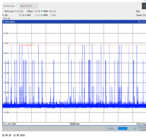
2DH3-Ant22-Hop-PASS
