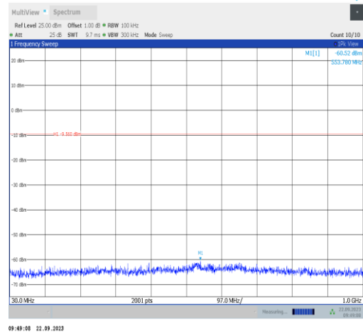
DH5-Ant22-2480-30~1000-PASS
