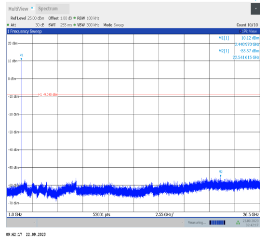
DH5-Ant22-2441-1000~26500-PASS
