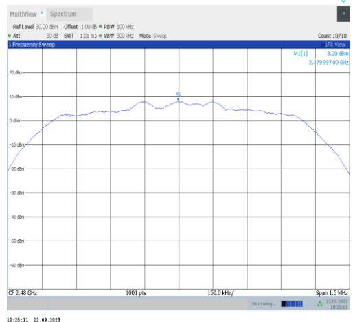
2DH5-Ant22-2480-0~Reference-PASS
