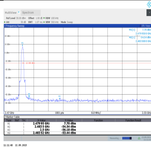
3DH5-Ant22-2480-PASS
